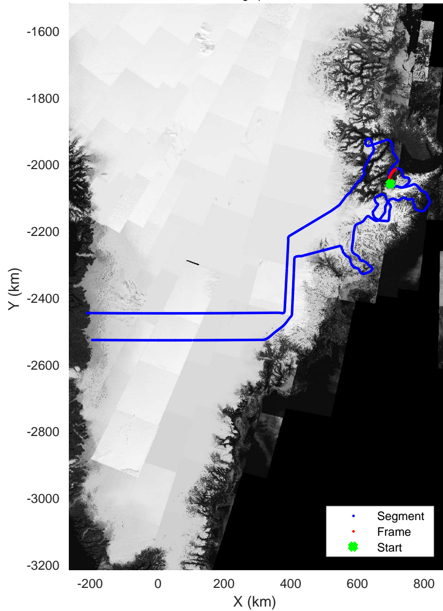
Geikie 02 20180421_01_040 Polar Stereograph 70N/-45E
