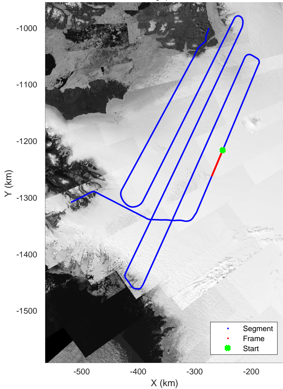
ICESat-2 North 20190417_02_041 Polar Stereograph 70N/-45E
