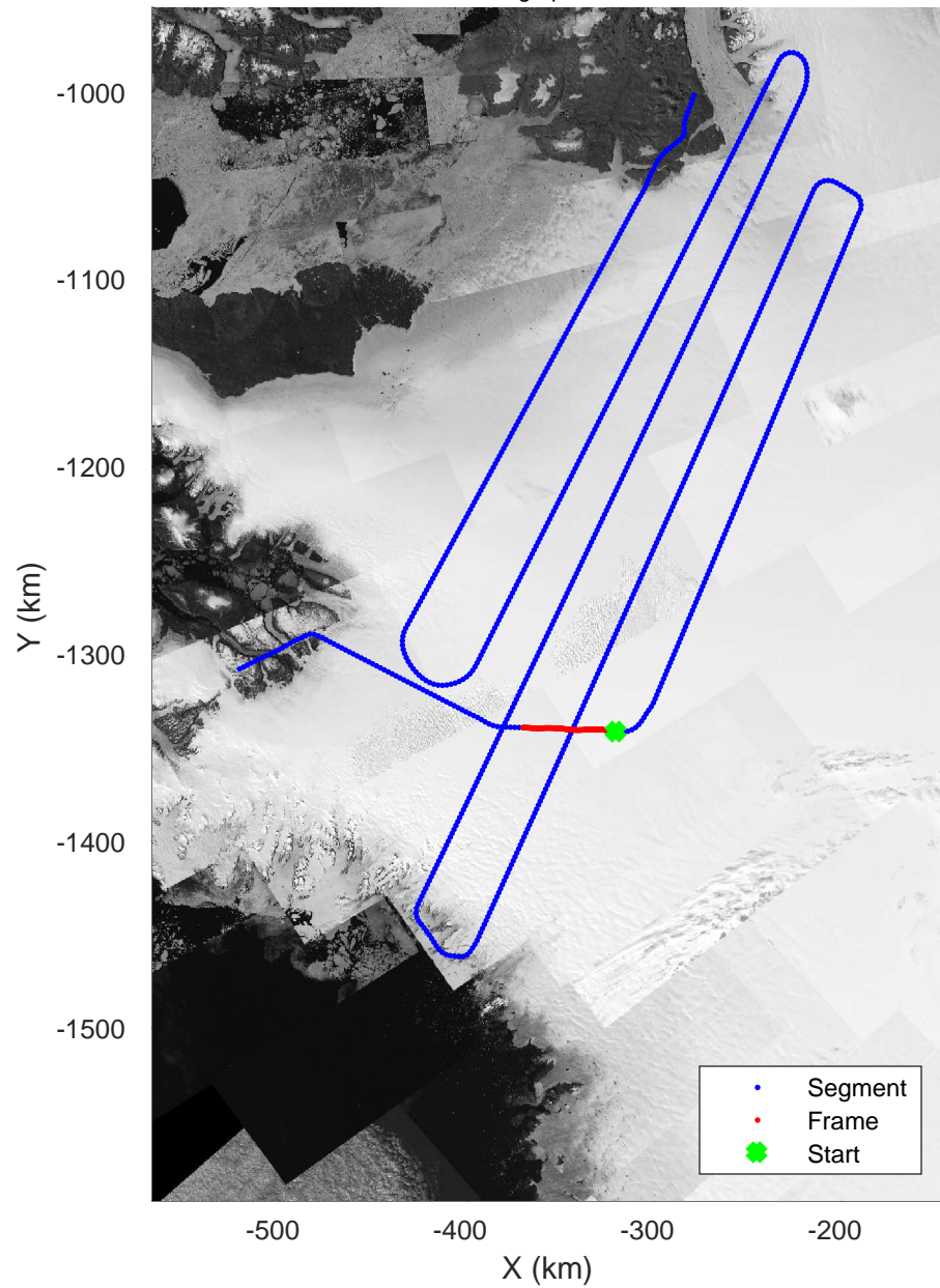
ICESat-2 North 20190417_02_044 Polar Stereograph 70N/-45E
