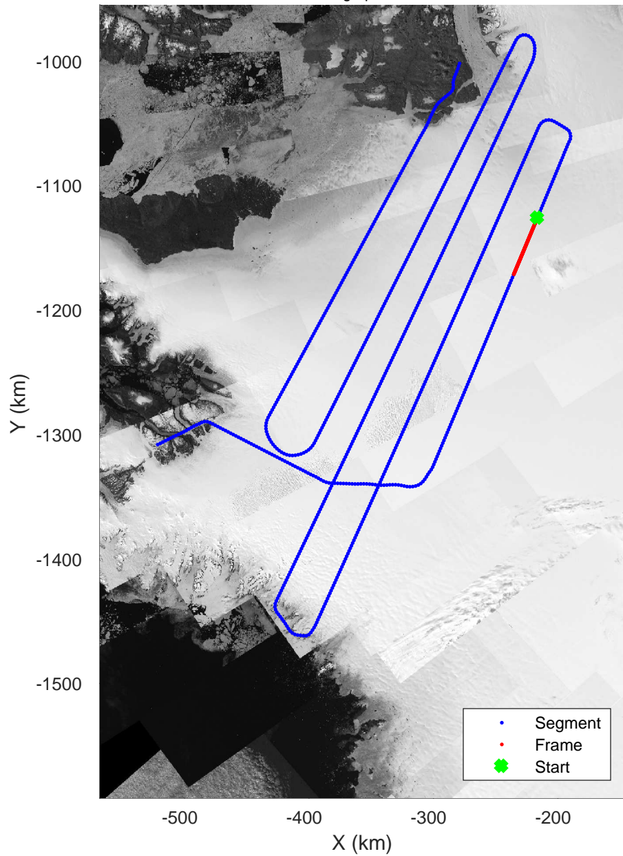
ICESat-2 North 20190417_02_039 Polar Stereograph 70N/-45E
