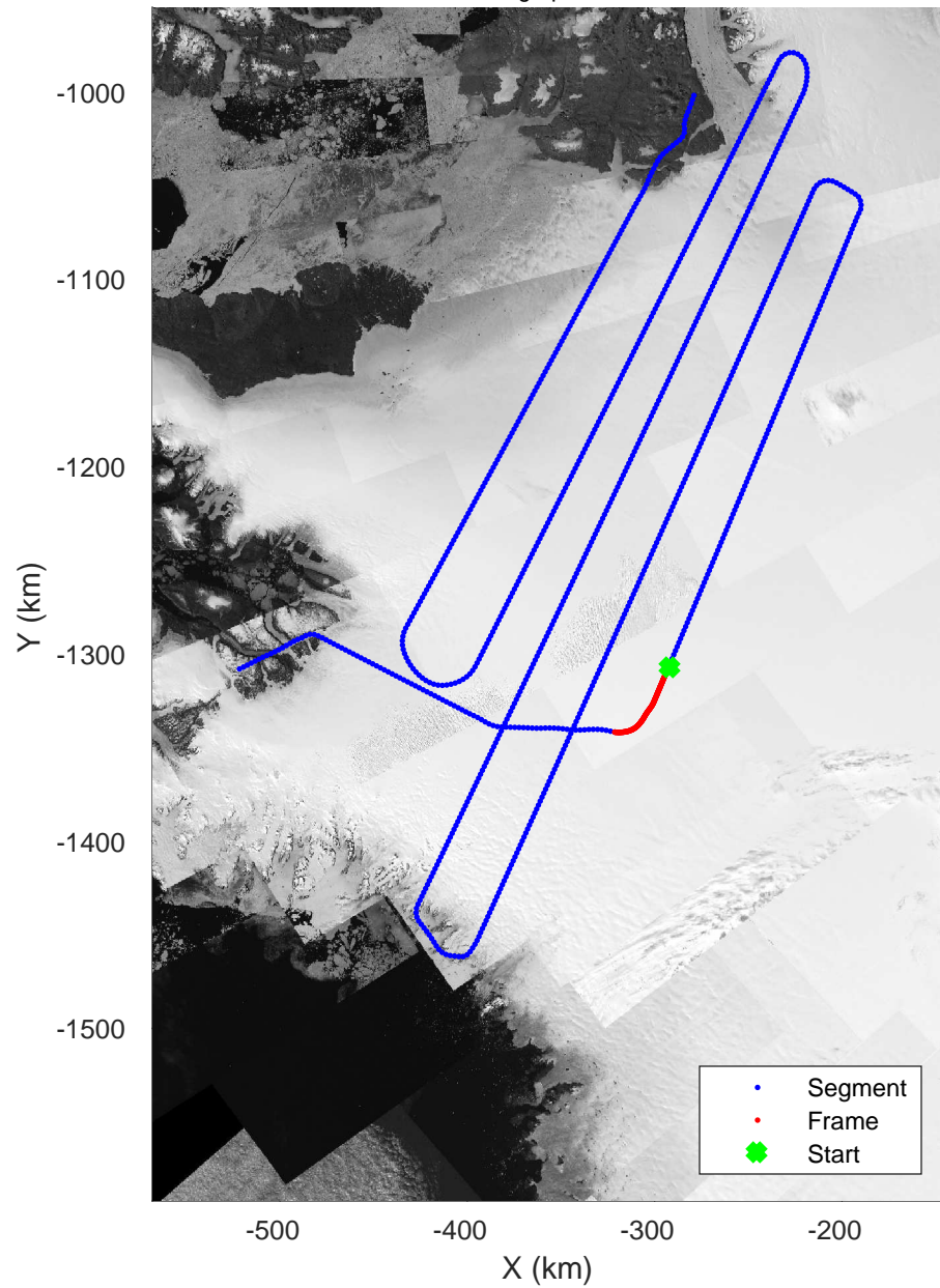
ICESat-2 North 20190417_02_043 Polar Stereograph 70N/-45E
