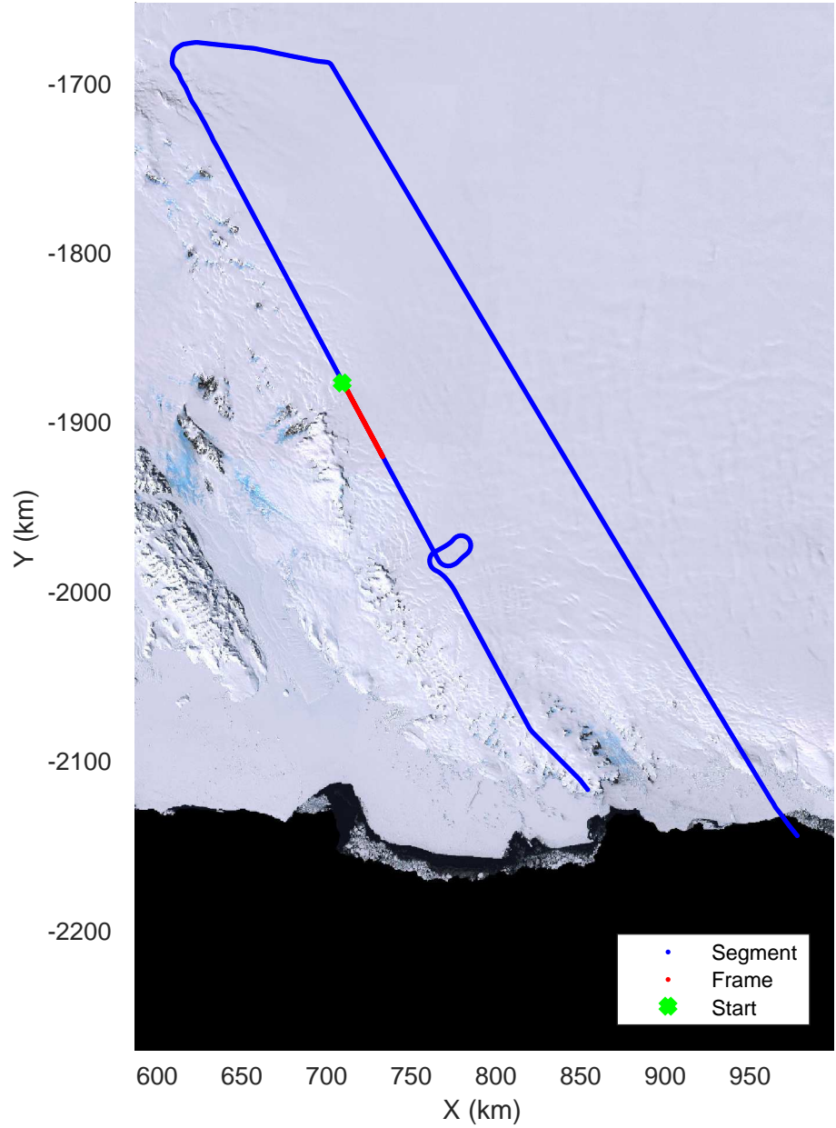
Matusevich-Cook IS-2 20191104_01_018 Polar Stereograph -71N/0E
