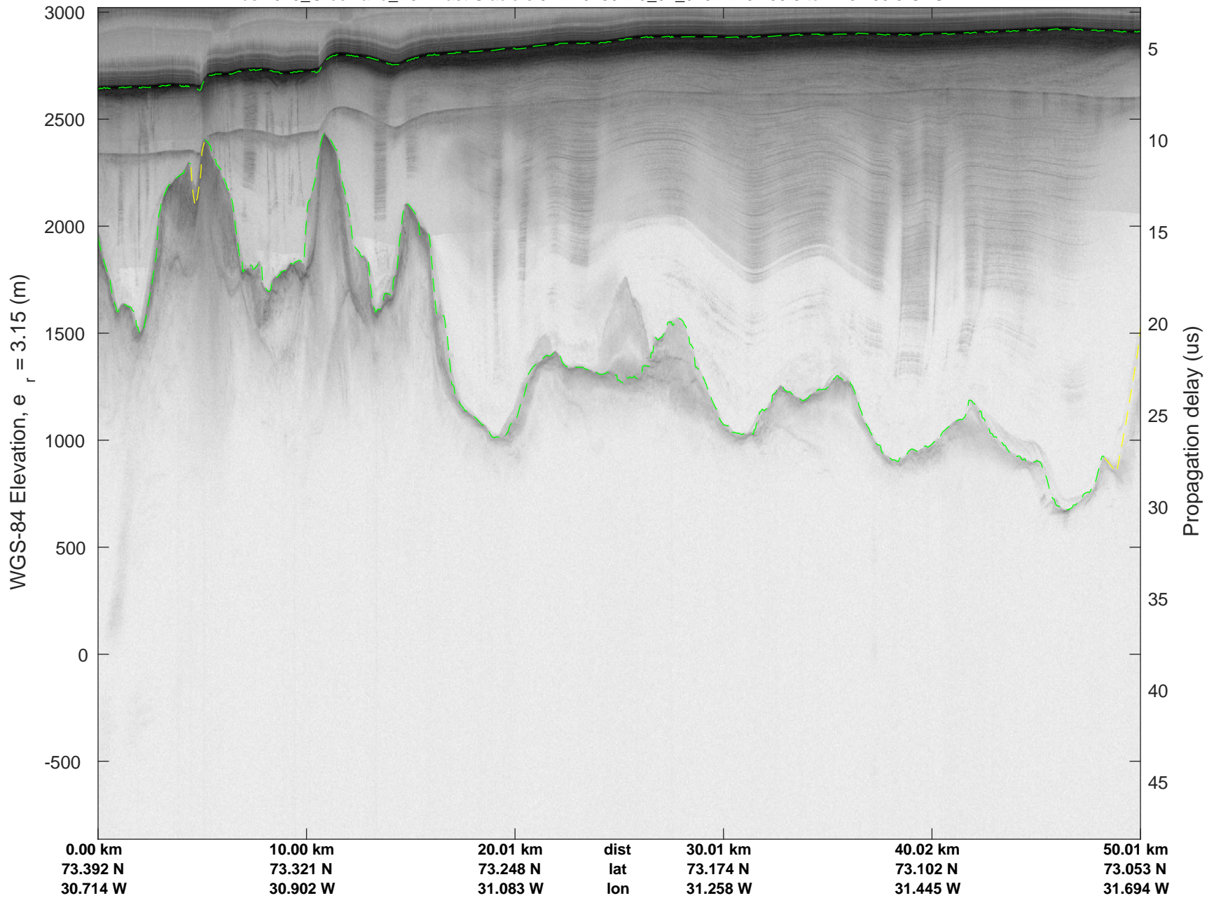
rds 2018_Greenland_P3: "East Glaciers 01" 20180423_01_045: 17:32:35.8 to 17:37:55.3 GPS
