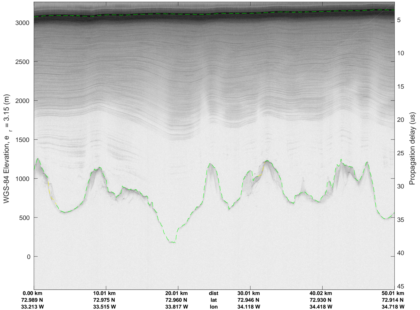
rds 2018_Greenland_P3: "East Glaciers 01" 20180423_01_047: 17:43:16.2 to 17:48:36.1 GPS
