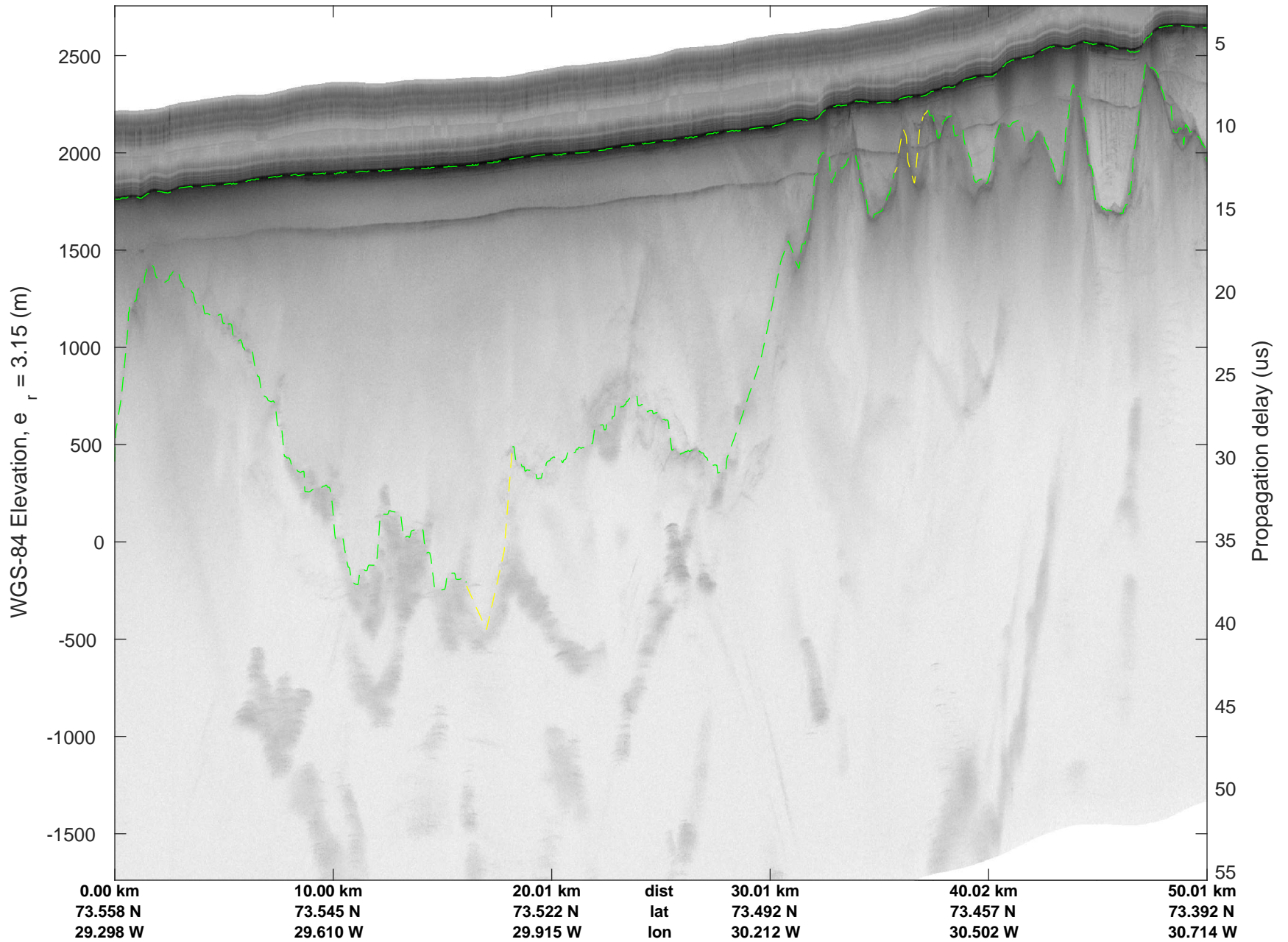
rds 2018_Greenland_P3: "East Glaciers 01" 20180423_01_044: 17:26:26.4 to 17:32:35.7 GPS
