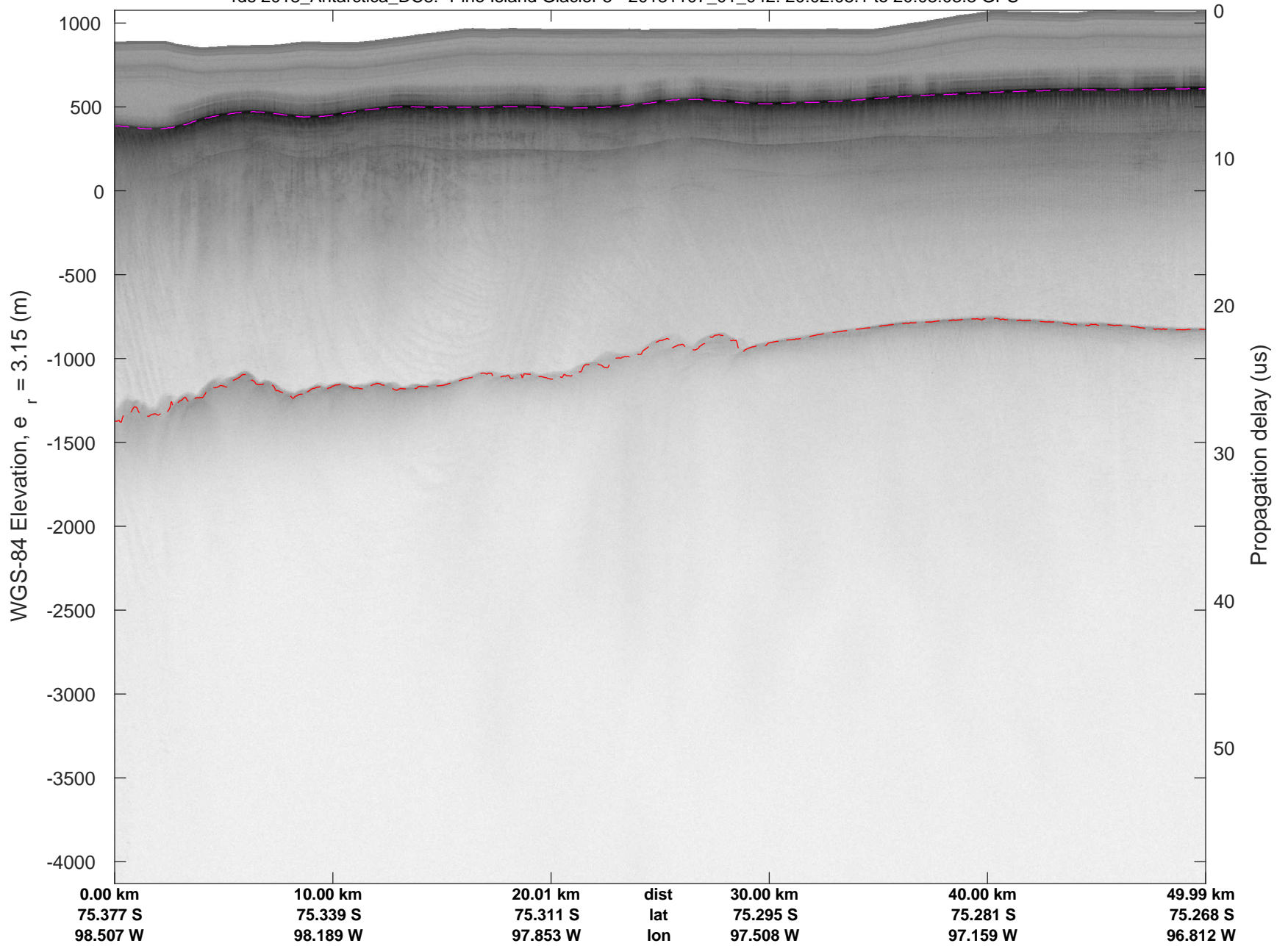
rds 2018_Antarctica_DC8: "Pine Island Glacier 5" 20181107_01_042: 20:02:08.1 to 20:08:03.3 GPS
