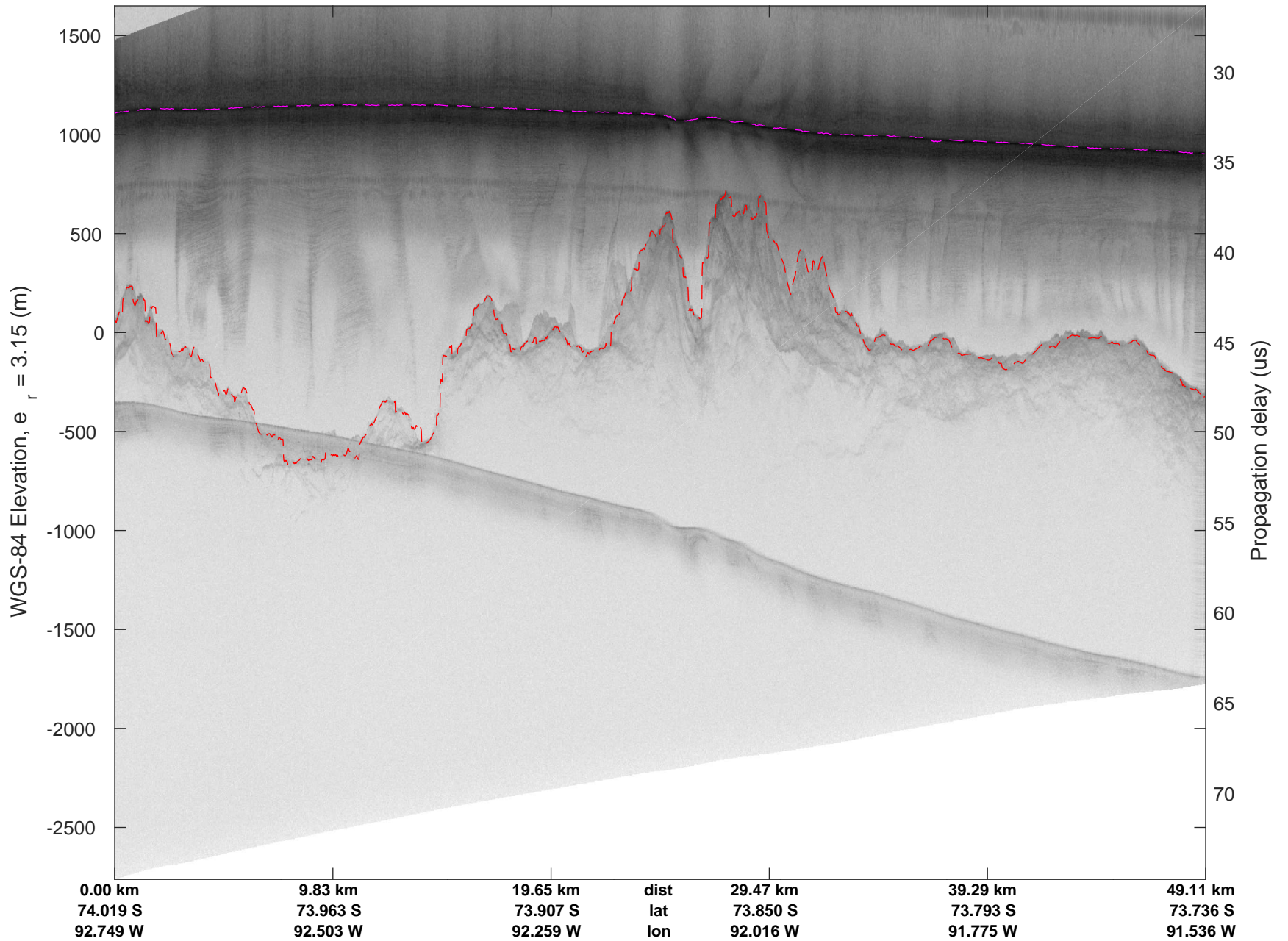
rds 2018_Antarctica_DC8: "Pine Island Glacier 5" 20181107_01_047: 20:29:37.2 to 20:33:16.7 GPS
