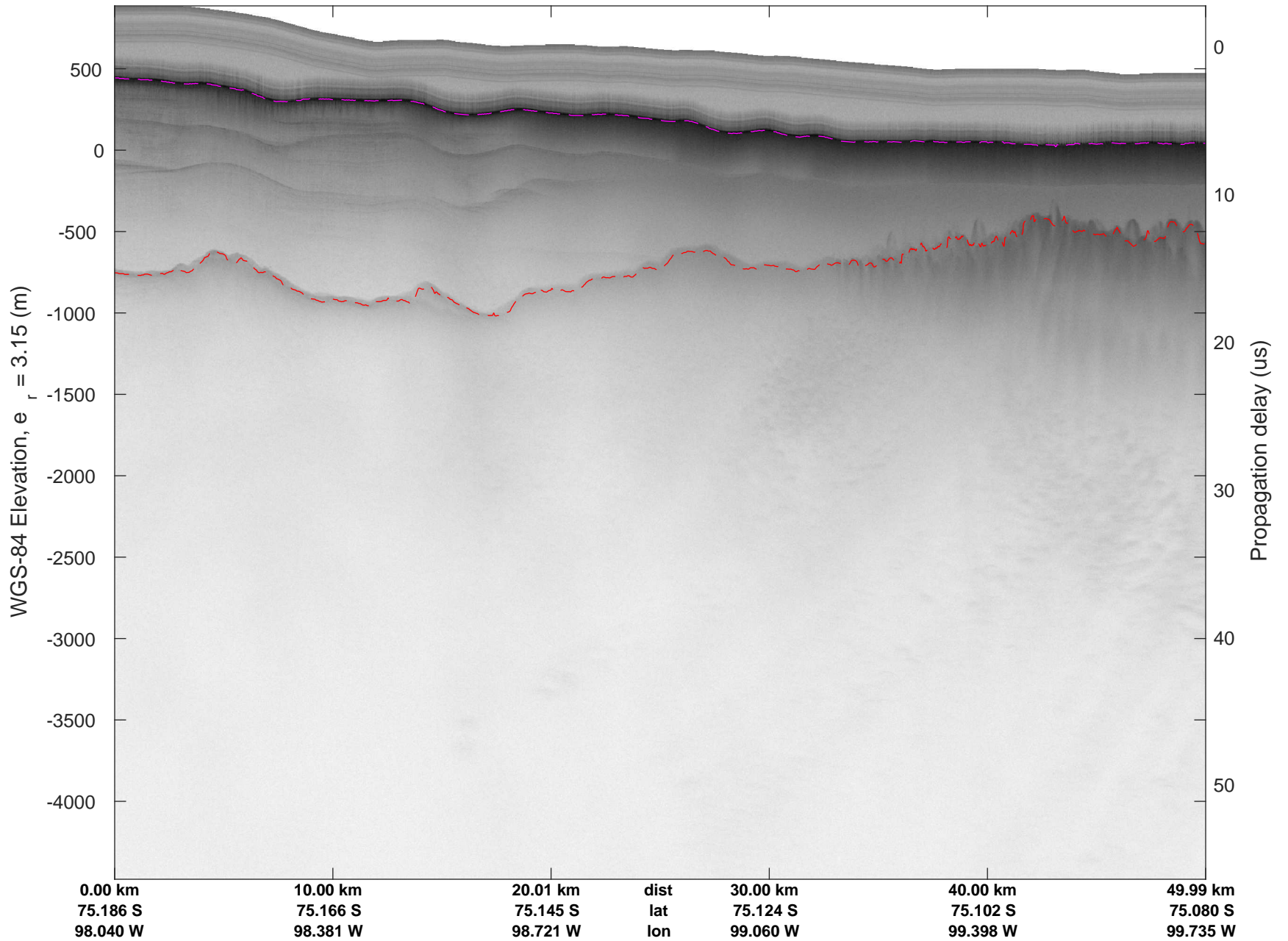
rds 2018_Antarctica_DC8: "Pine Island Glacier 5" 20181107_01_019: 17:45:17.9 to 17:51:07.3 GPS
