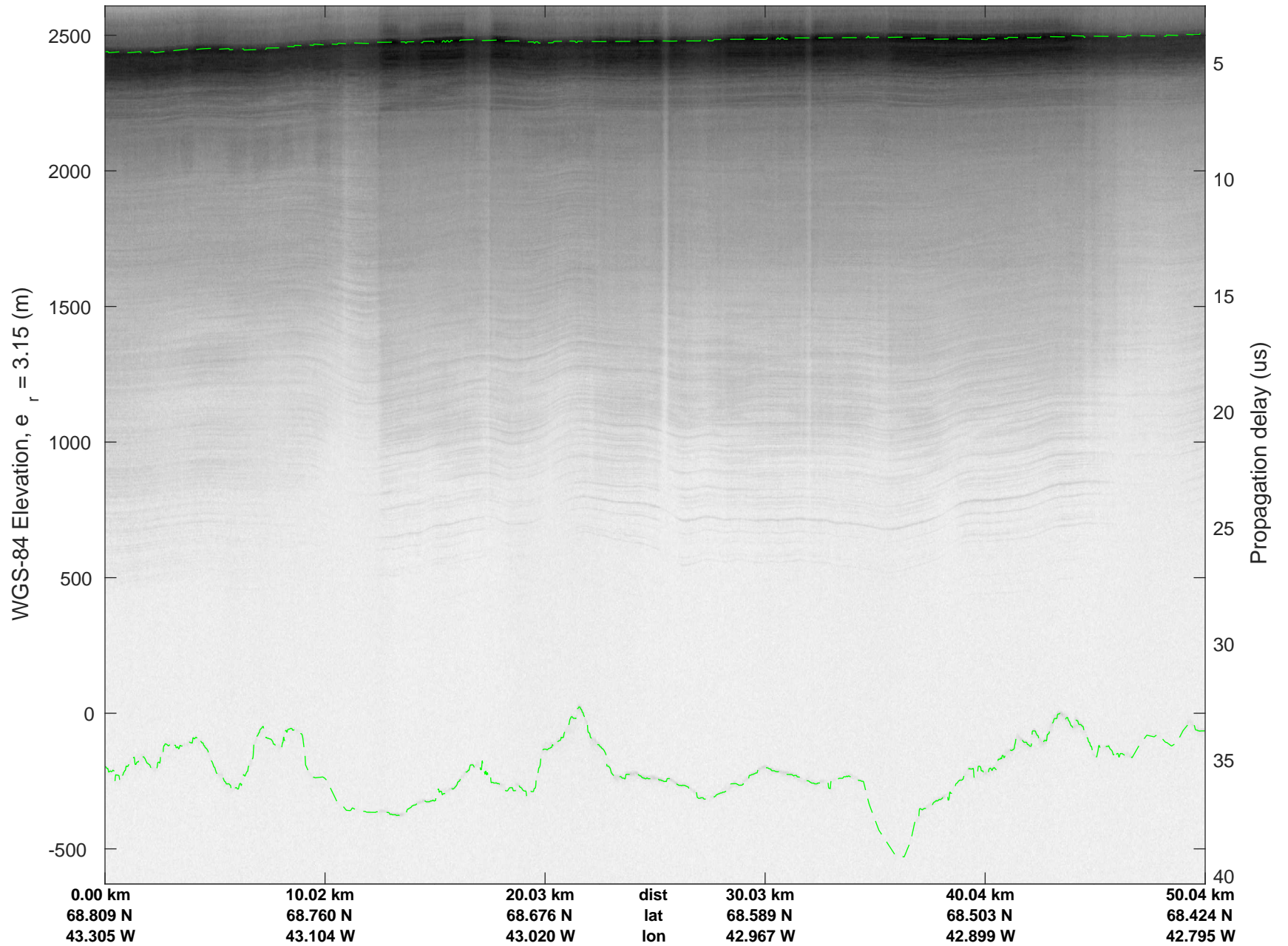
rds 2017_Greenland_P3: "ICESat-2 Central" 20170502_01_044: 14:54:29.7 to 15:00:50.3 GPS
