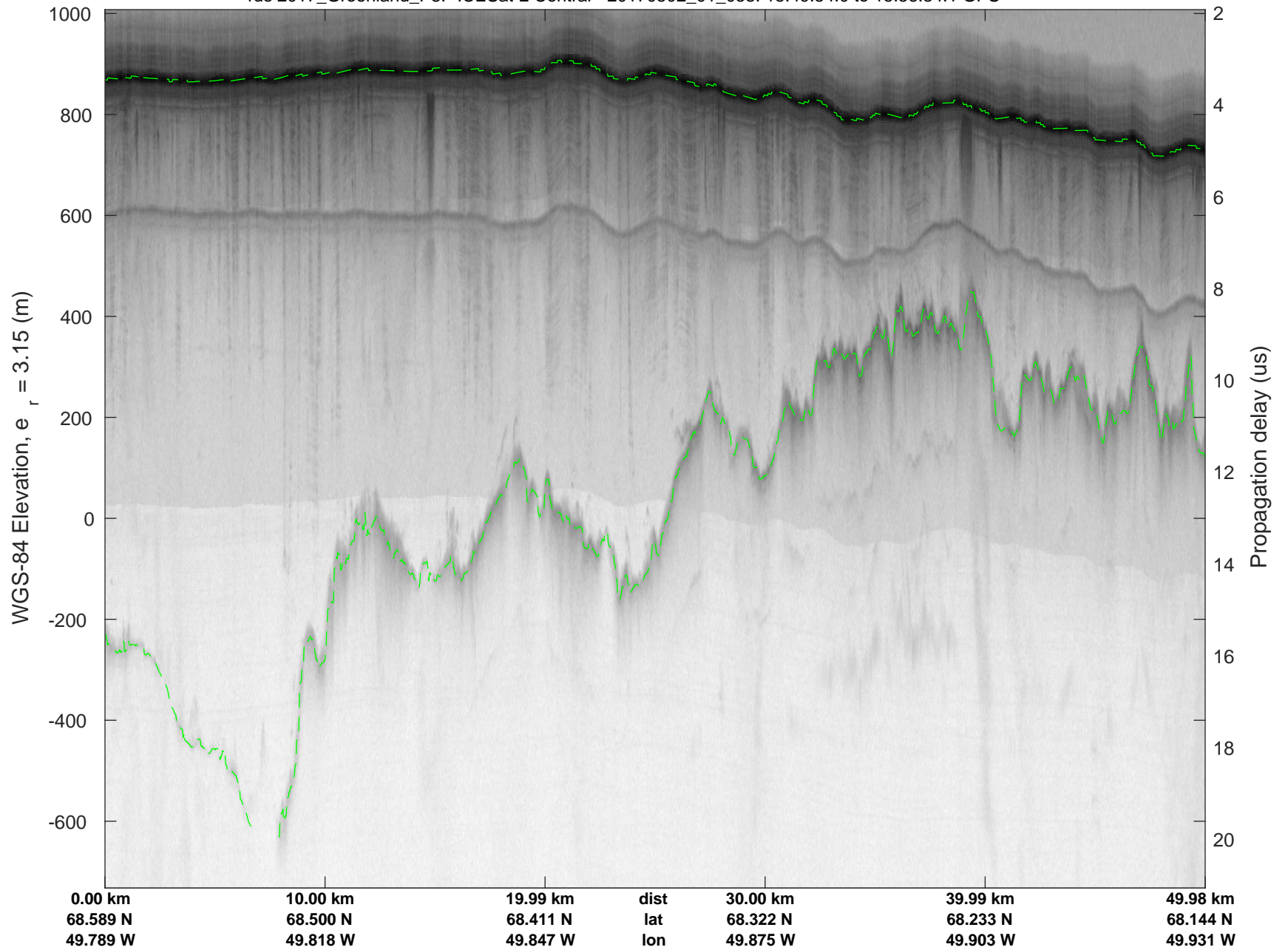
rds 2017_Greenland_P3: "ICESat-2 Central" 20170502_01_053: 15:49:54.0 to 15:56:34.1 GPS
