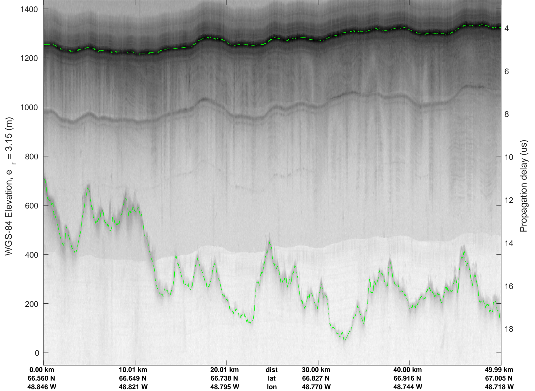
rds 2017_Greenland_P3: "ICESat-2 Central" 20170502_01_012: 11:36:11.2 to 11:41:59.7 GPS
