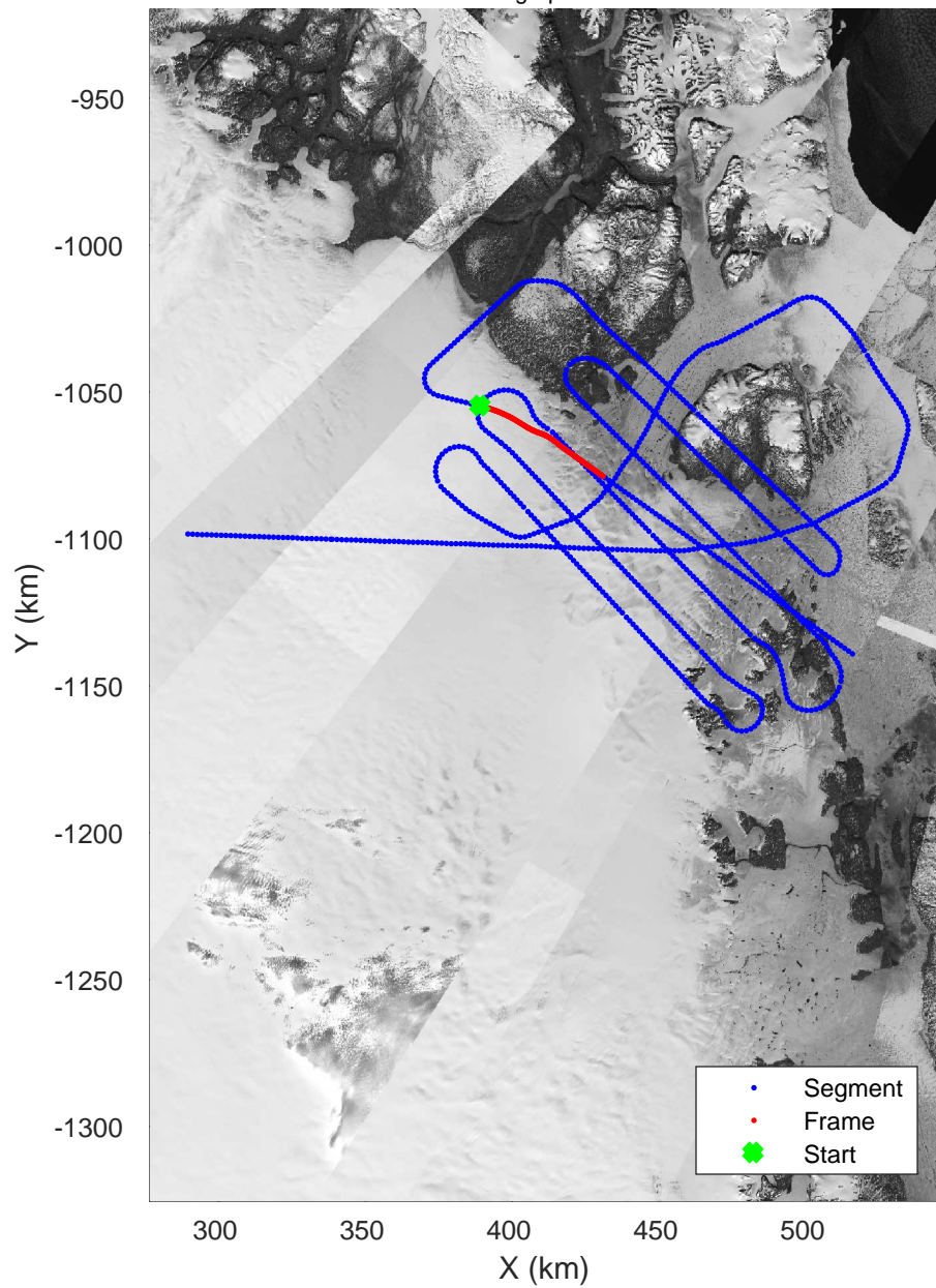
Zachariae-79N 20170403_02_031 Polar Stereograph 70N/-45E
