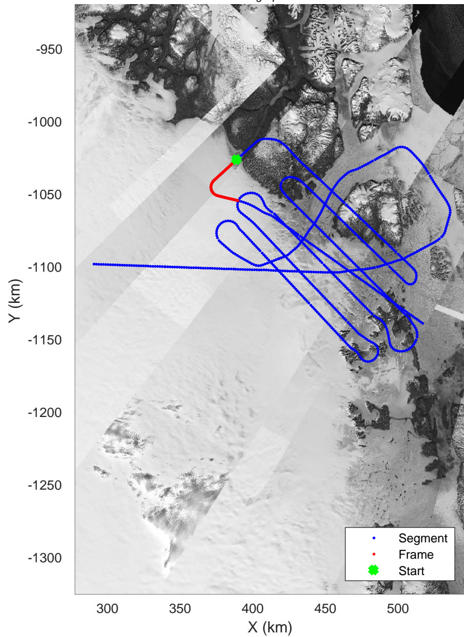
Zachariae-79N 20170403_02_030 Polar Stereograph 70N/-45E
