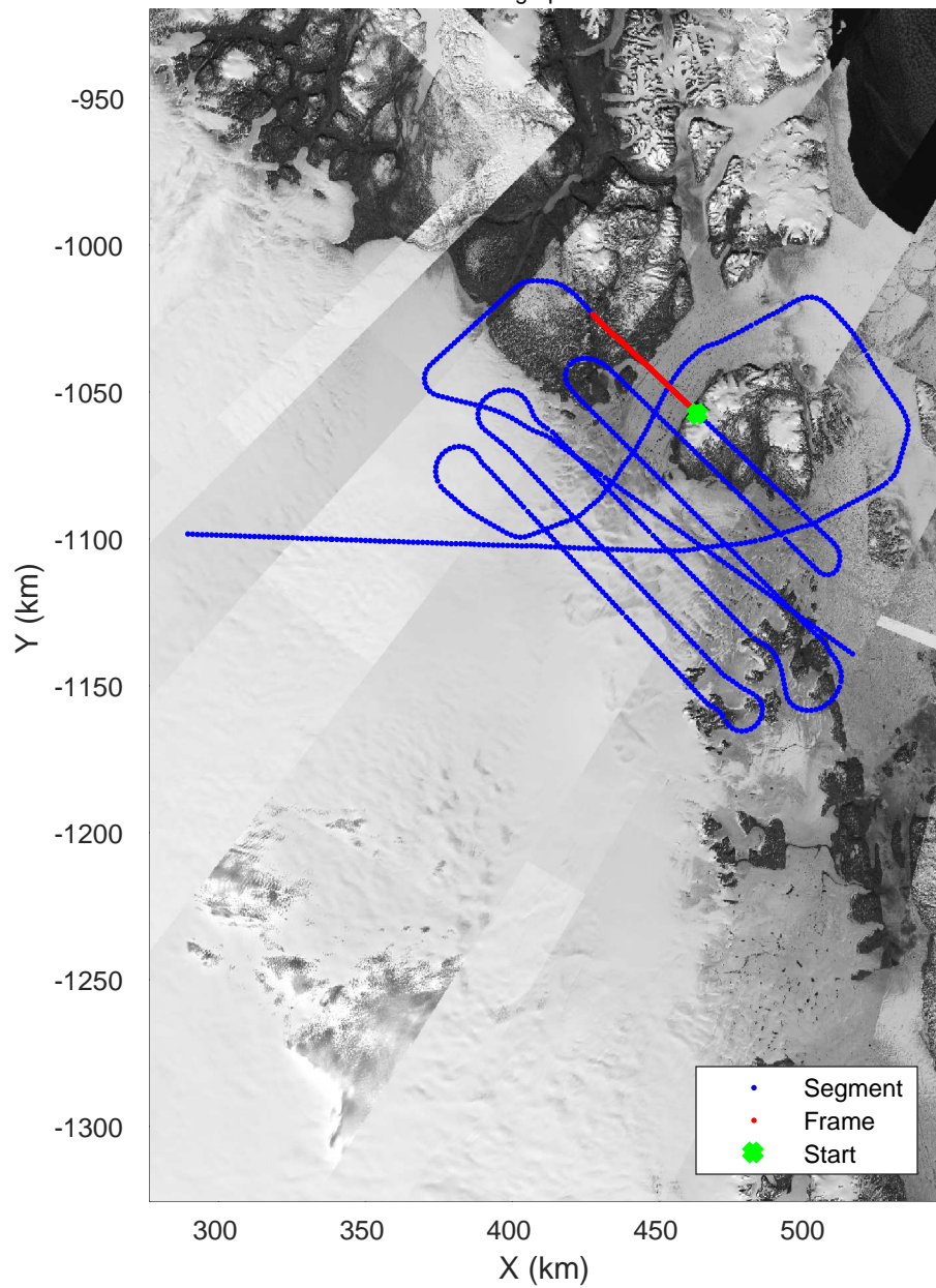
Zachariae-79N 20170403_02_028 Polar Stereograph 70N/-45E
