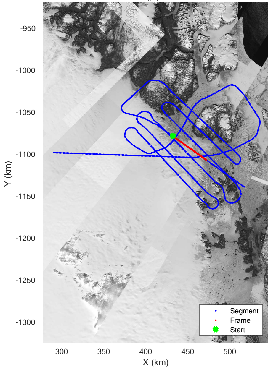
Zachariae-79N 20170403_02_032 Polar Stereograph 70N/-45E
