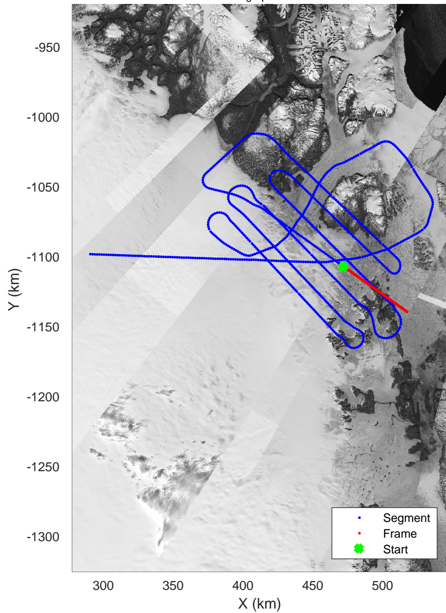
Zachariae-79N 20170403_02_033 Polar Stereograph 70N/-45E
