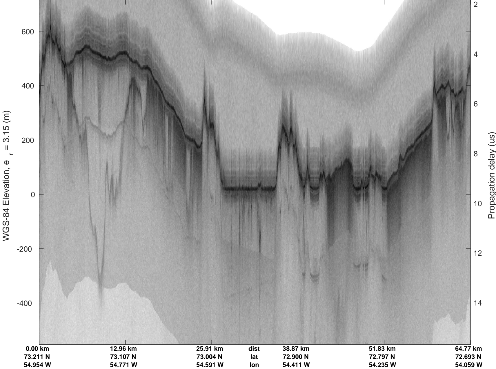
rds 2017_Greenland_P3: "Northwest Coastal A" 20170327_01_009: 12:24:16.7 to 12:32:46.0 GPS
