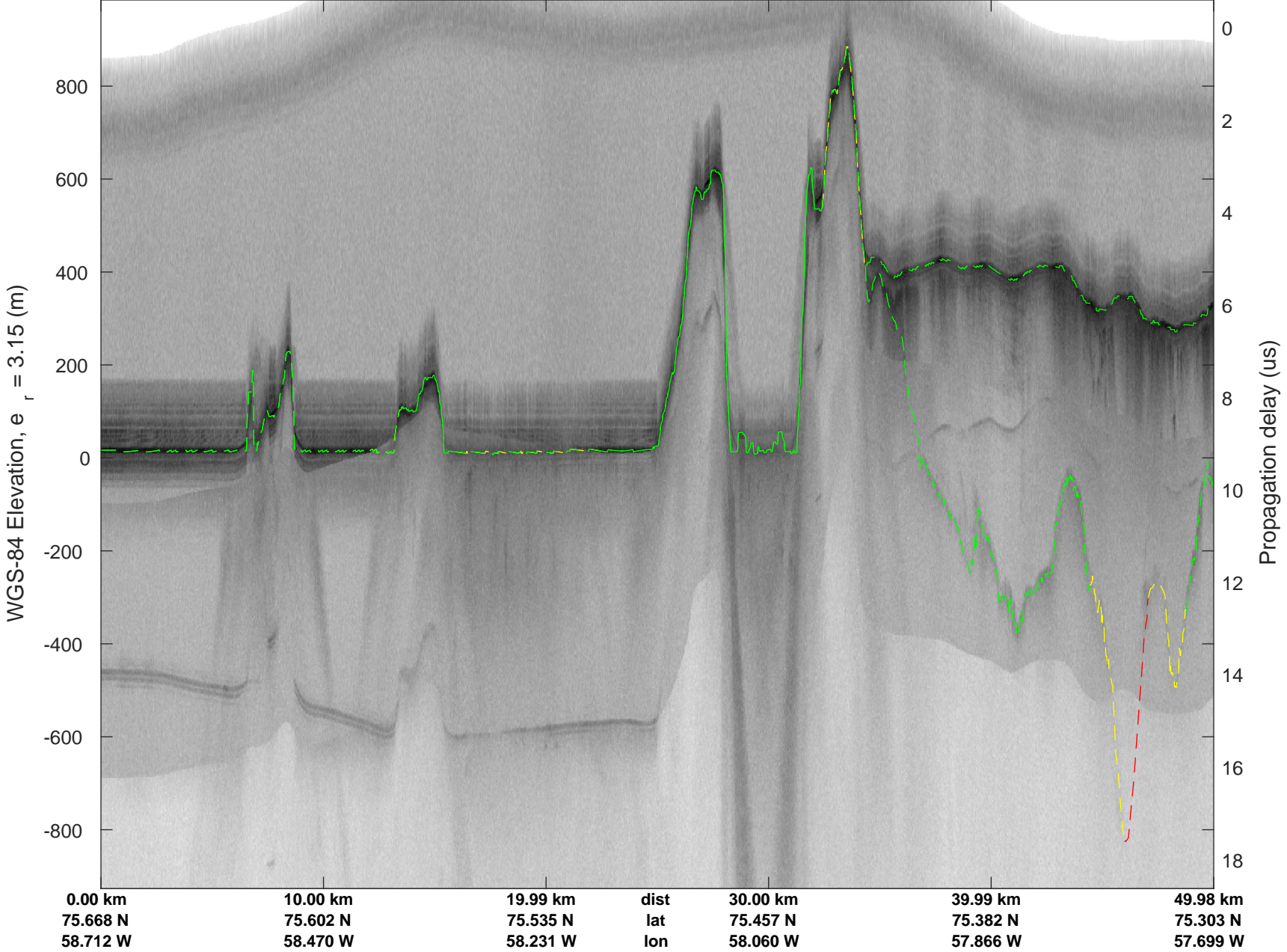
rds 2017_Greenland_P3: "Northwest Coastal A" 20170327_01_003: 11:44:20.7 to 11:50:56.9 GPS
