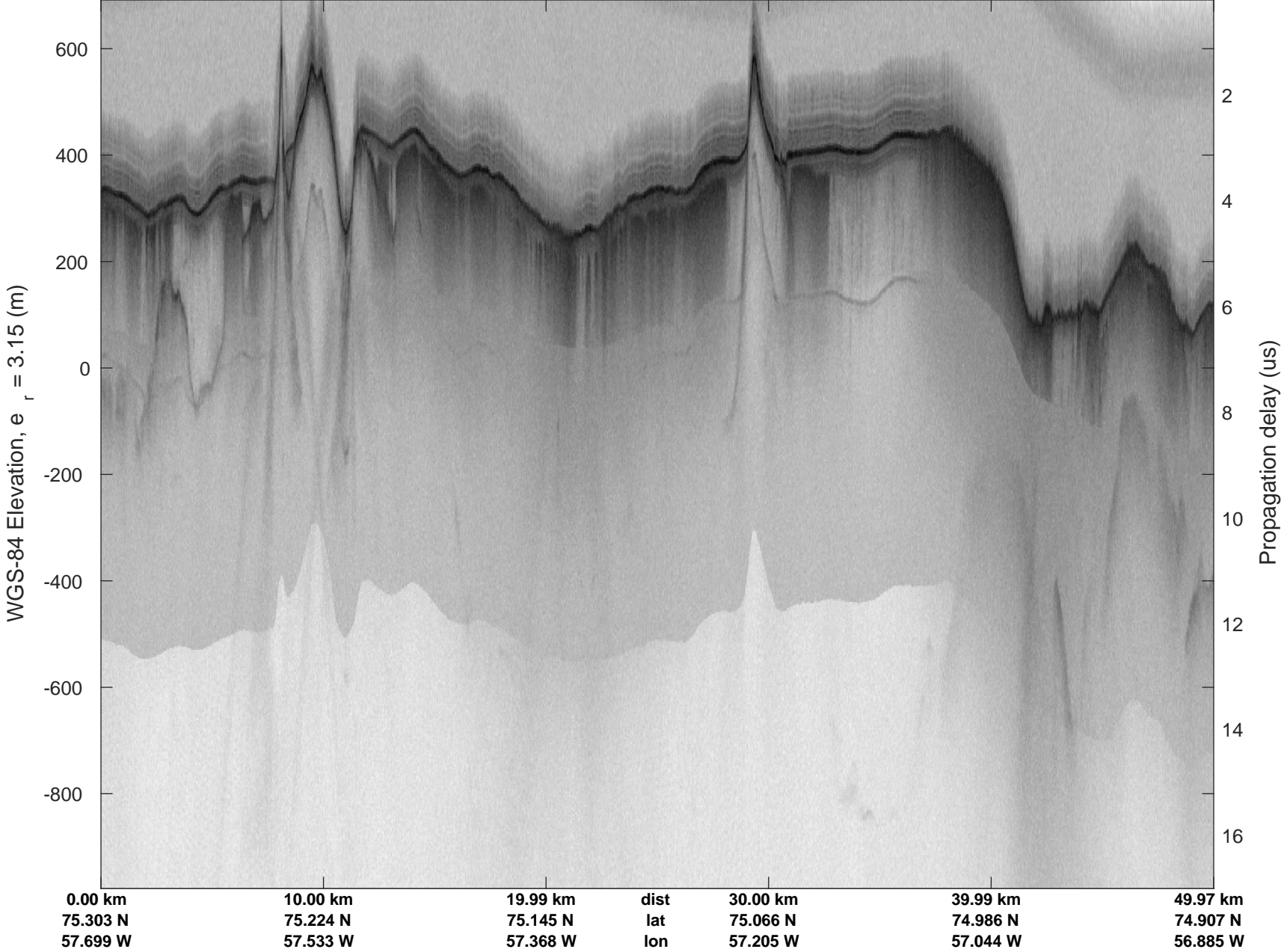
rds 2017_Greenland_P3: "Northwest Coastal A" 20170327_01_004: 11:50:57.2 to 11:57:51.0 GPS
