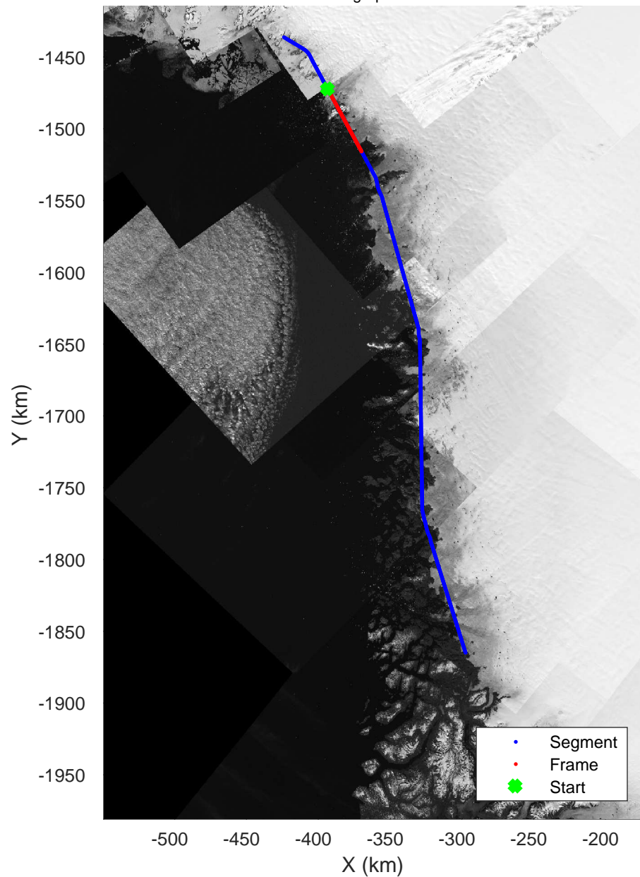
Northwest Coastal A 20170327_01_002 Polar Stereograph 70N/-45E
