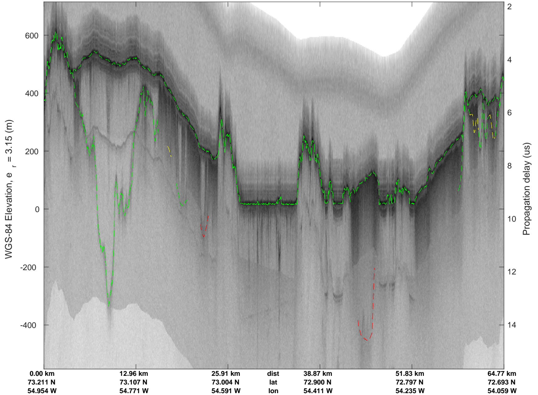
rds 2017_Greenland_P3: "Northwest Coastal A" 20170327_01_009: 12:24:16.7 to 12:32:46.0 GPS
