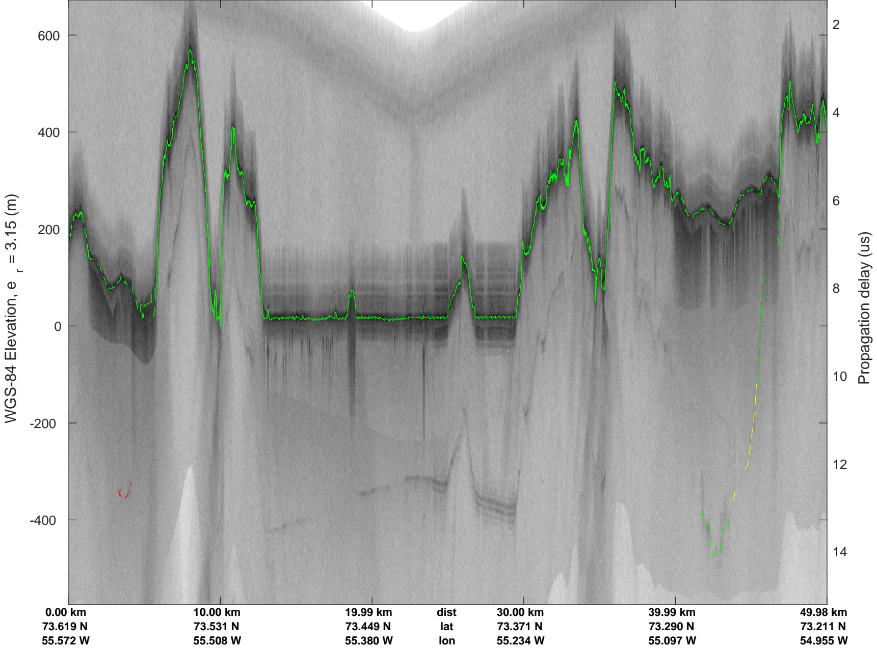
rds 2017_Greenland_P3: "Northwest Coastal A" 20170327_01_008: 12:17:41.7 to 12:24:16.4 GPS
