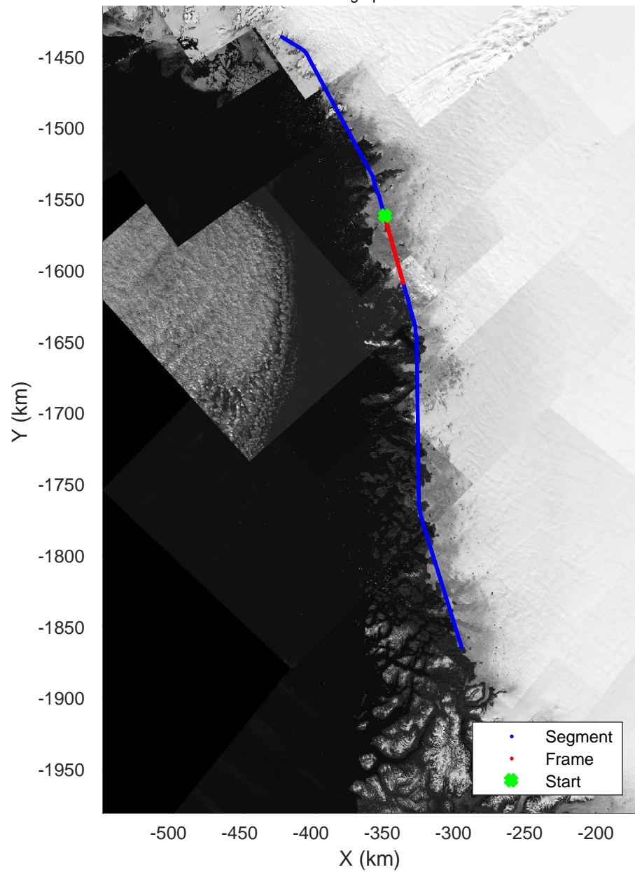
Northwest Coastal A 20170327_01_004 Polar Stereograph 70N/-45E
