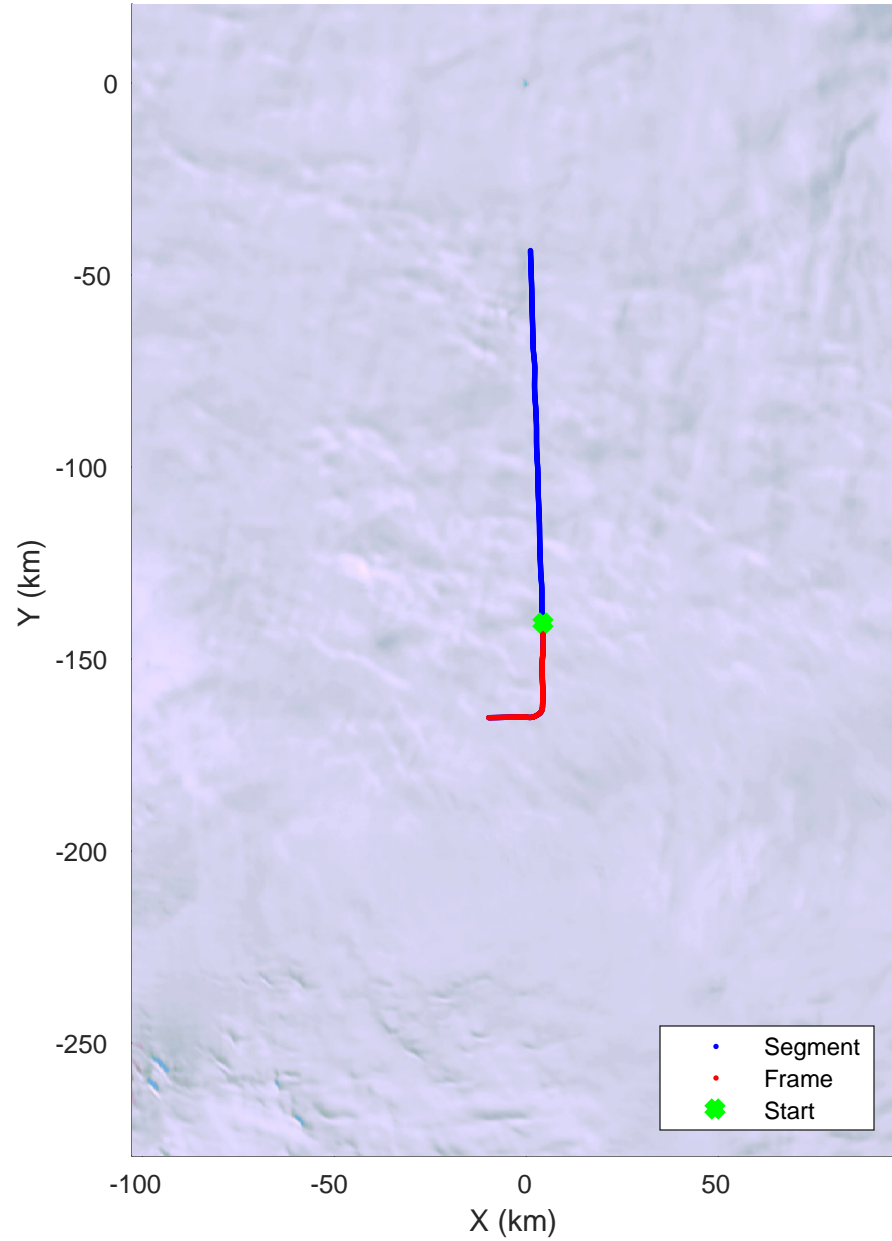
TAM Gate East Low/Hamilton Line 2/TAM East 20171204_05_003 Polar Stereograph -71N/0E
