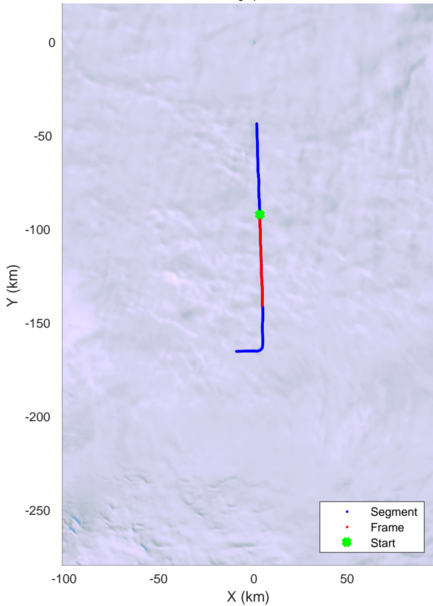
TAM Gate East Low/Hamilton Line 2/TAM East 20171204_05_002 Polar Stereograph -71N/0E
