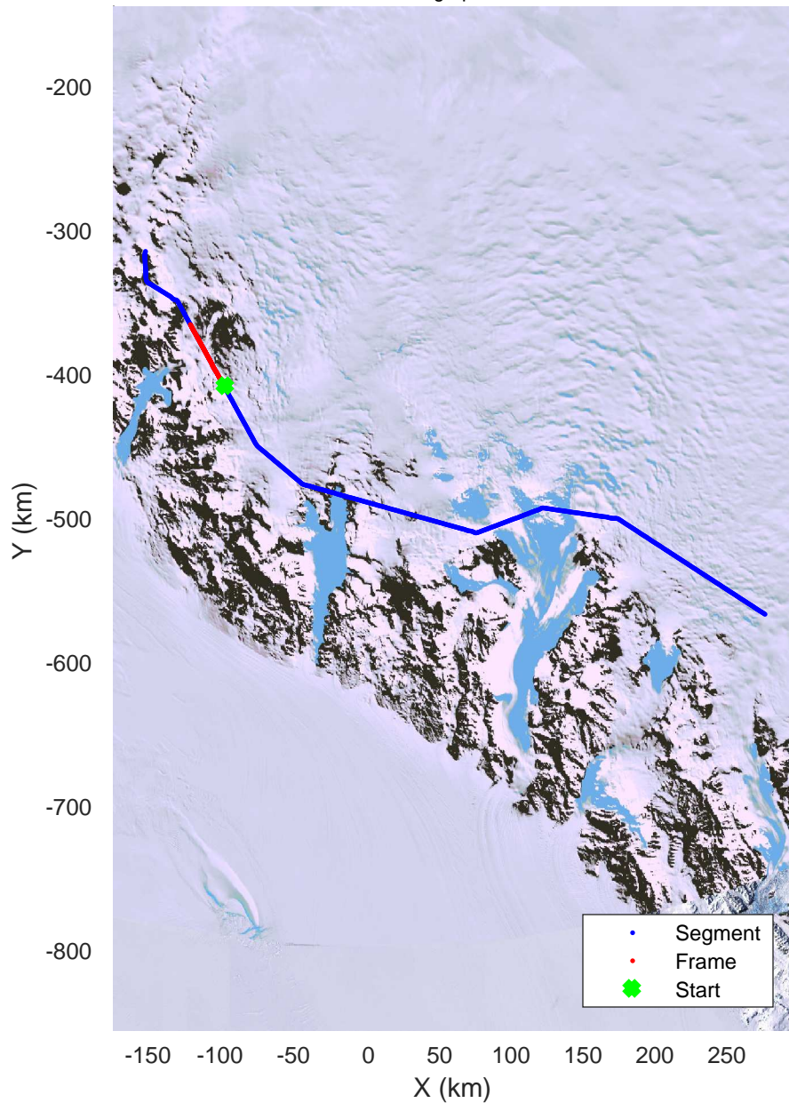
TAM Gate East Low/Hamilton Line 2/TAM East 20171204_03_010 Polar Stereograph -71N/0E
