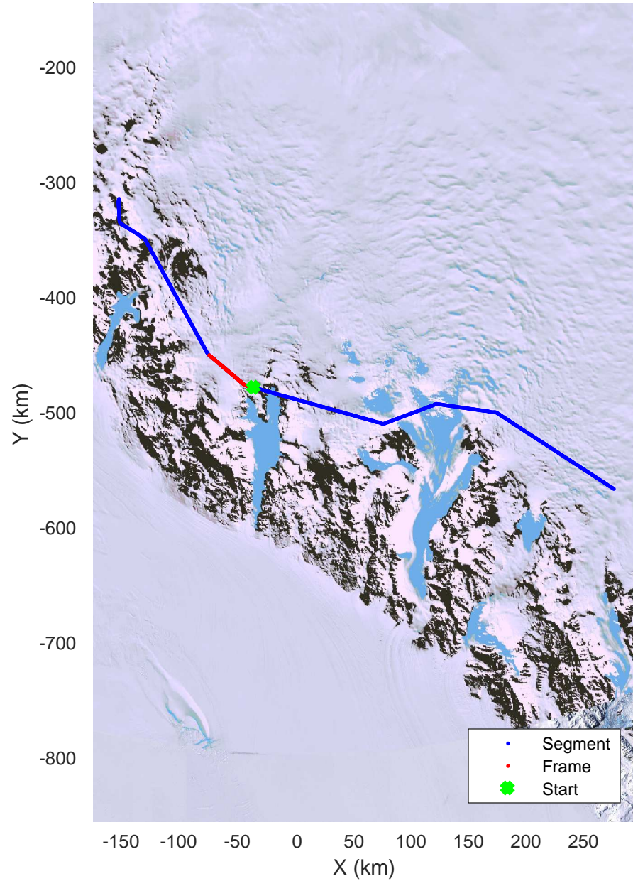
TAM Gate East Low/Hamilton Line 2/TAM East 20171204_03_008 Polar Stereograph -71N/0E
