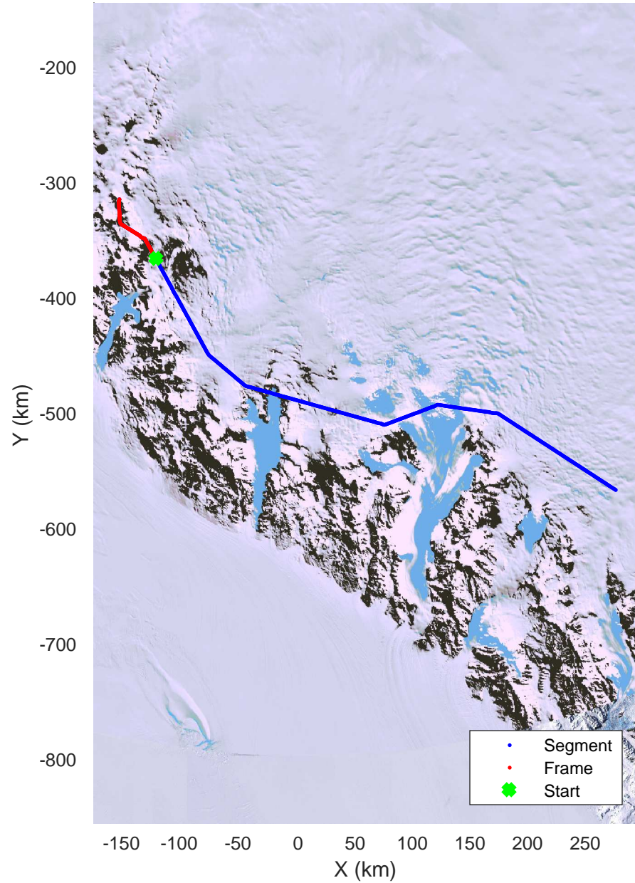
TAM Gate East Low/Hamilton Line 2/TAM East 20171204_03_011 Polar Stereograph -71N/0E
