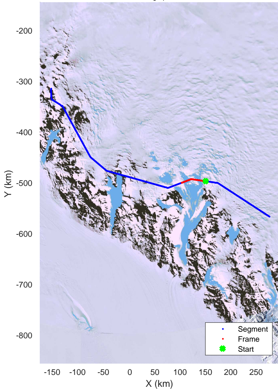
TAM Gate East Low/Hamilton Line 2/TAM East 20171204_03_004 Polar Stereograph -71N/0E
