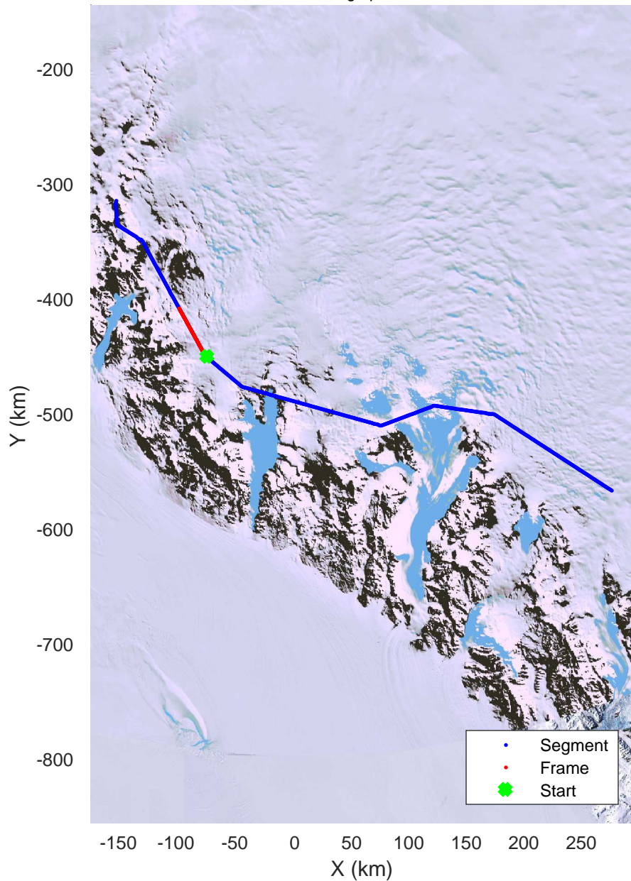
TAM Gate East Low/Hamilton Line 2/TAM East 20171204_03_009 Polar Stereograph -71N/0E
