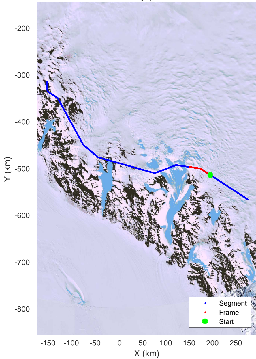
TAM Gate East Low/Hamilton Line 2/TAM East 20171204_03_003 Polar Stereograph -71N/0E
