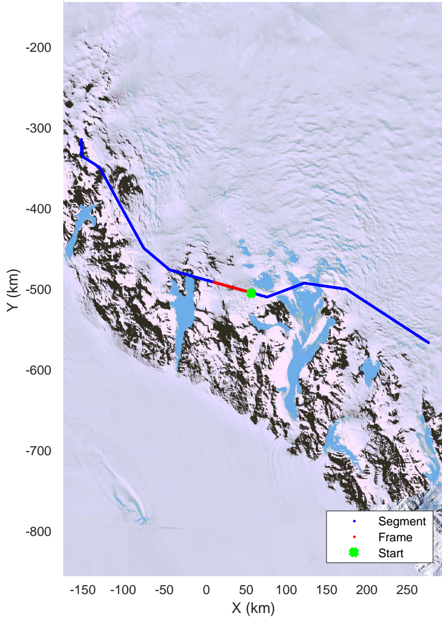
TAM Gate East Low/Hamilton Line 2/TAM East 20171204_03_006 Polar Stereograph -71N/0E
