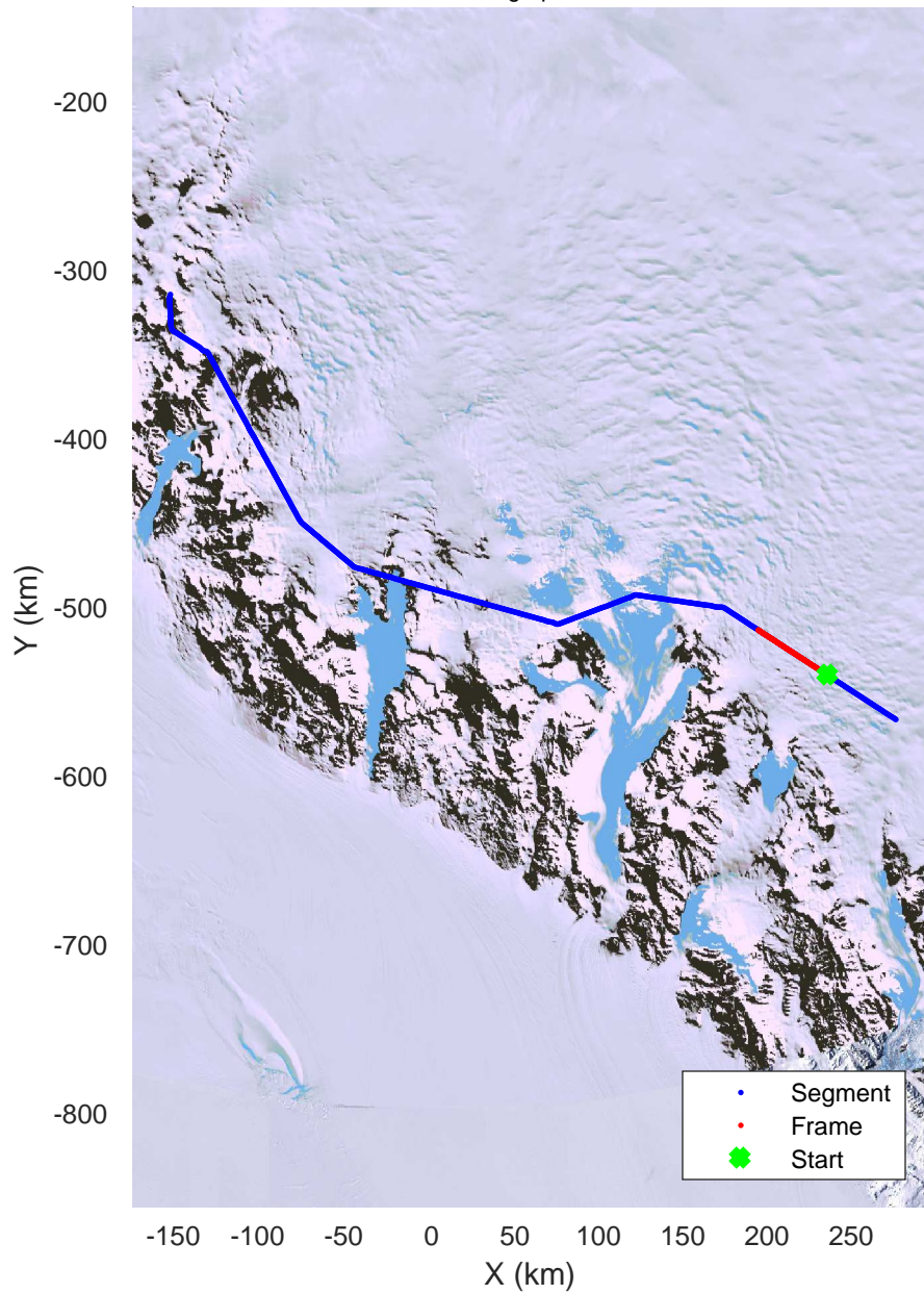
TAM Gate East Low/Hamilton Line 2/TAM East 20171204_03_002 Polar Stereograph -71N/0E
