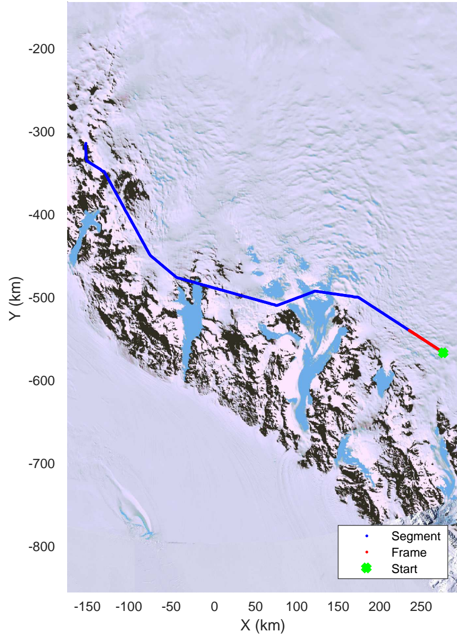
TAM Gate East Low/Hamilton Line 2/TAM East 20171204_03_001 Polar Stereograph -71N/0E
