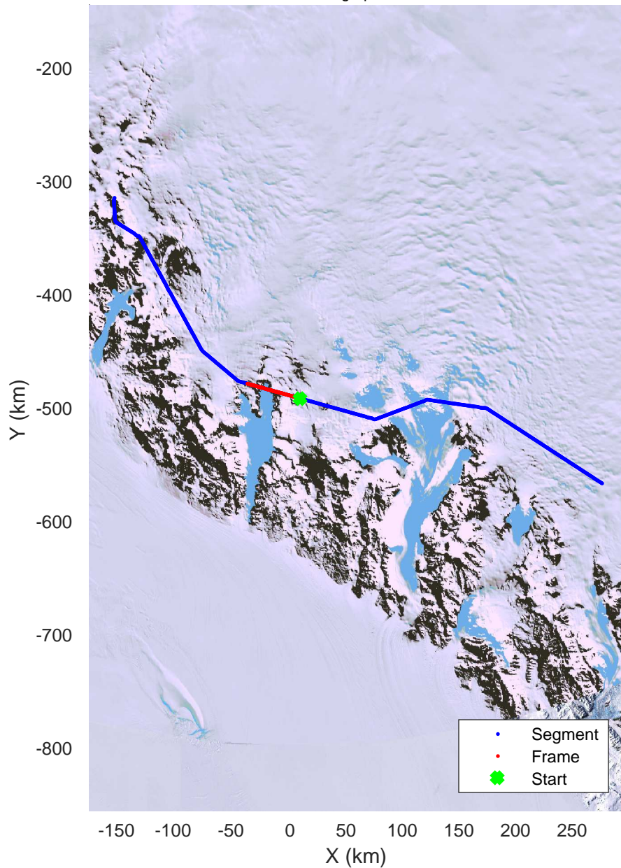
TAM Gate East Low/Hamilton Line 2/TAM East 20171204_03_007 Polar Stereograph -71N/0E
