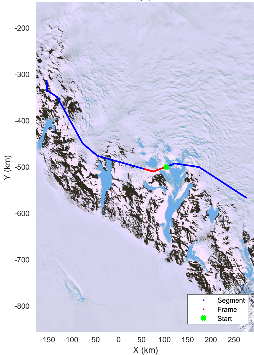
TAM Gate East Low/Hamilton Line 2/TAM East 20171204_03_005 Polar Stereograph -71N/0E
