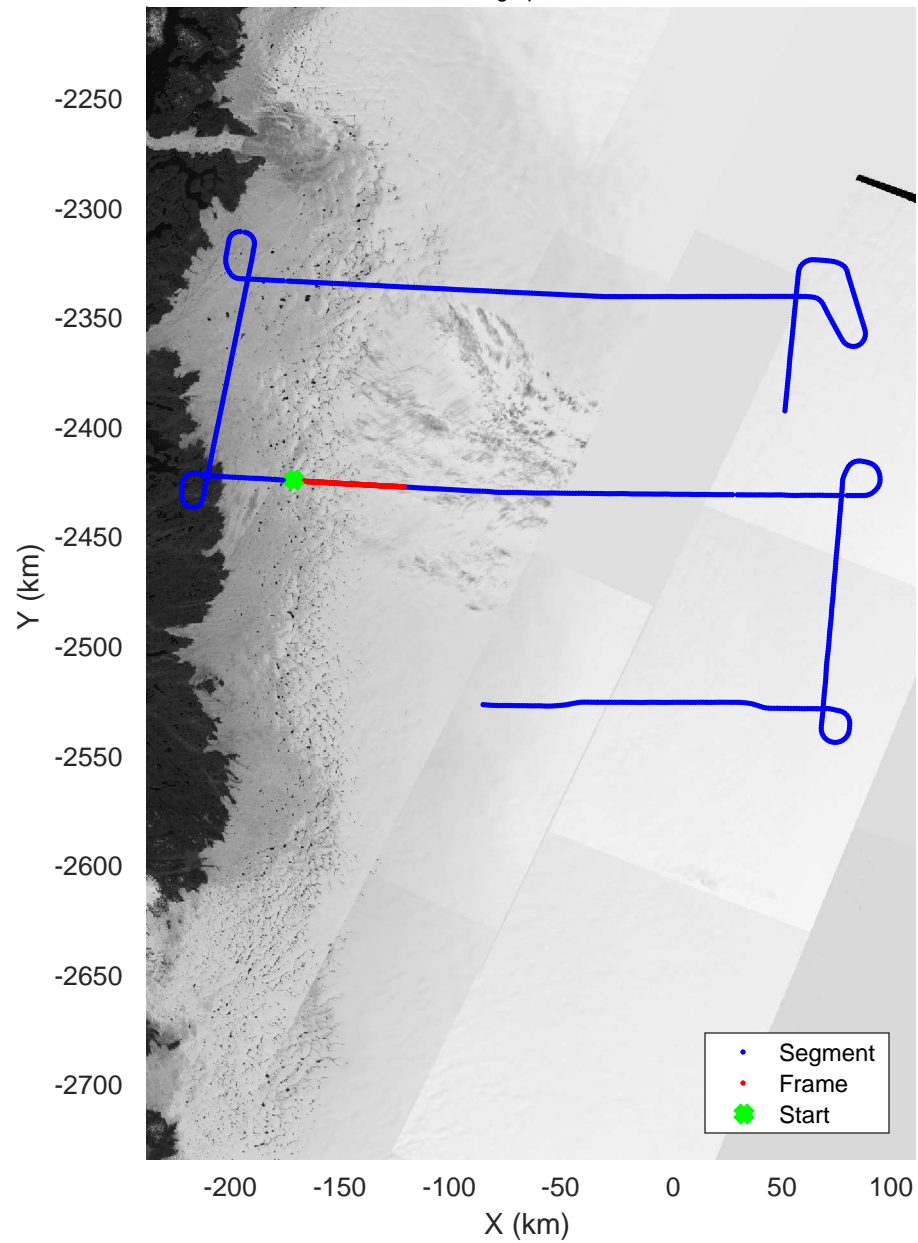
IceSat-2 Central 20160518_02_014 Polar Stereograph 70N/-45E
