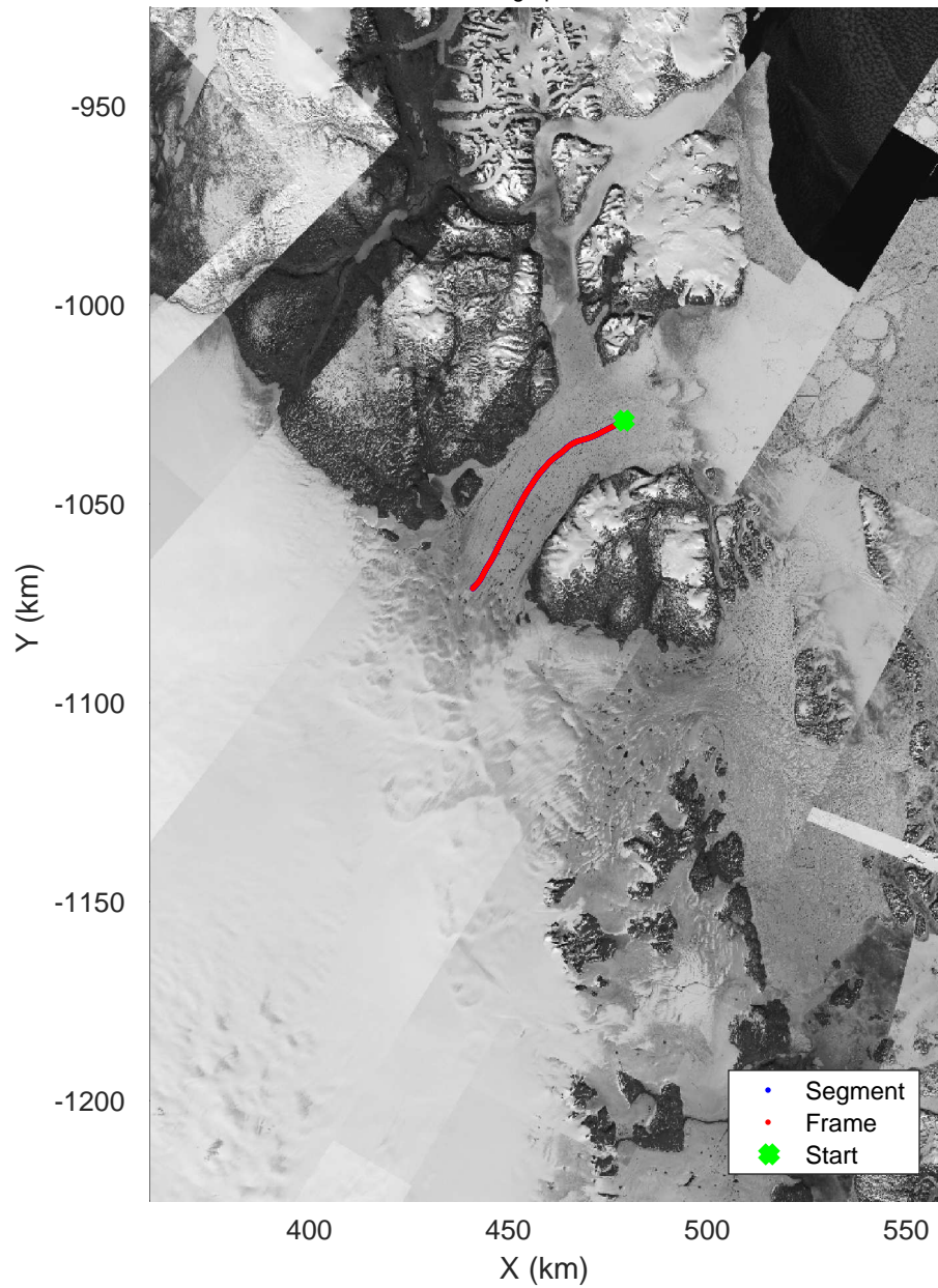
Zachariae-79N 20160509_10_001 Polar Stereograph 70N/-45E
