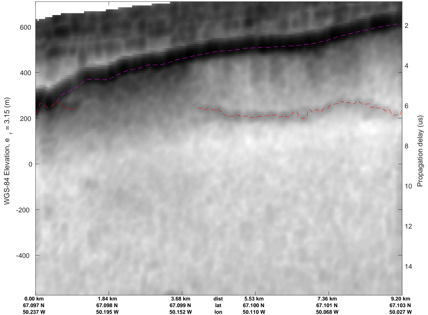
rds 2016_Greenland_G1XB: "Medium line 3" 20160417_04_004: 21:30:34.3 to 21:37:07.1 GPS
