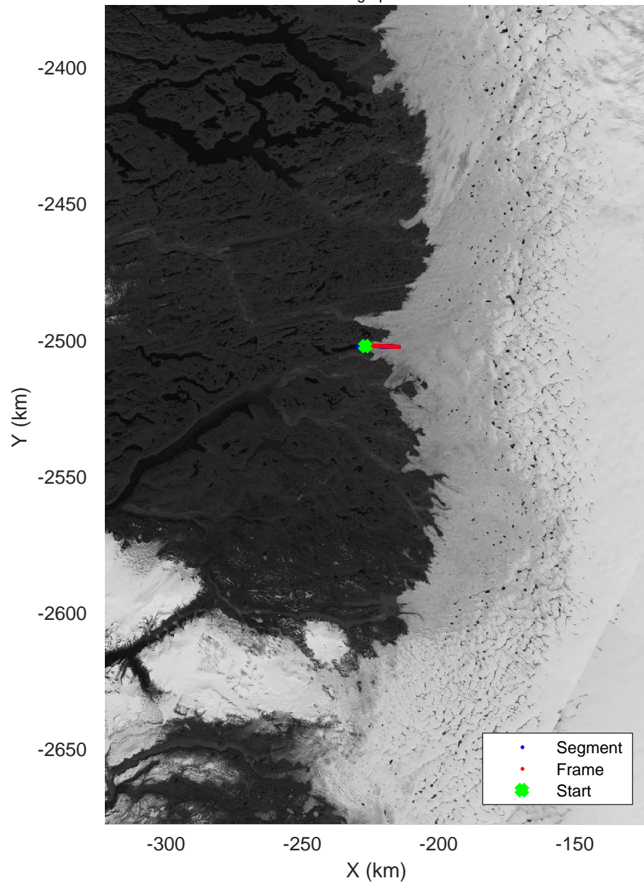
Bad line 3 20160417_03_002 Polar Stereograph 70N/-45E
