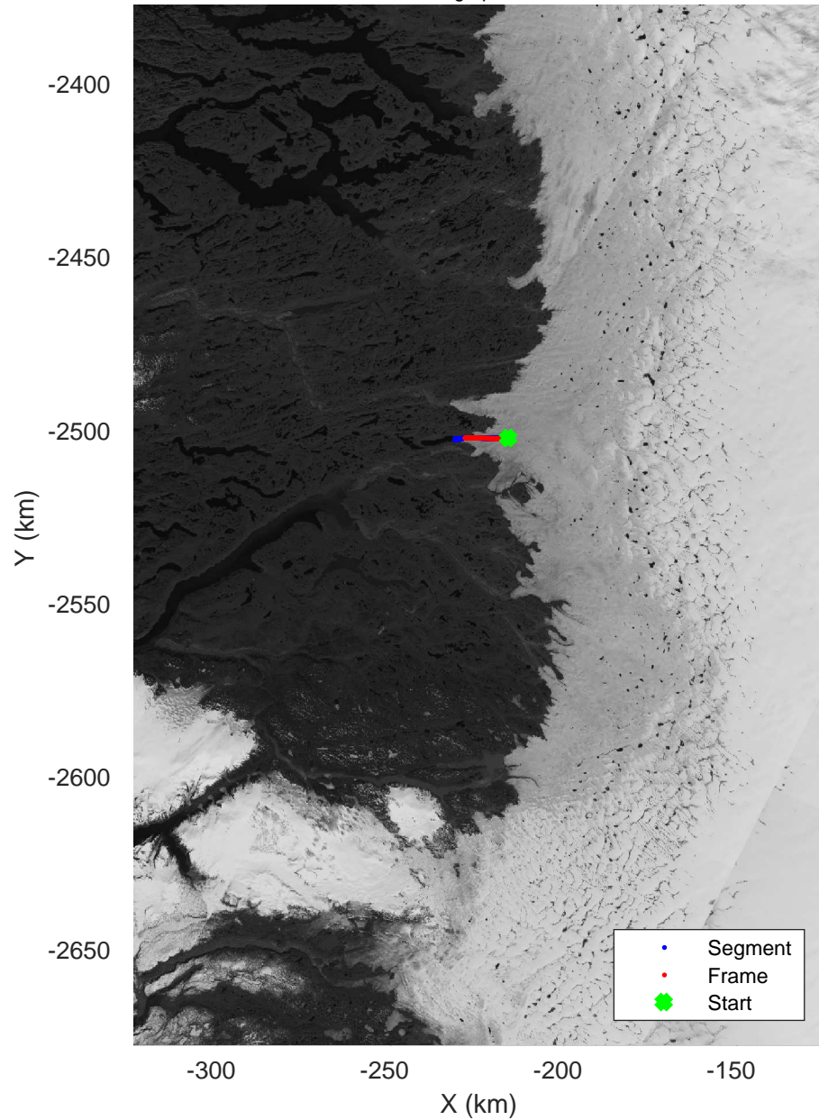
Bad line 3 20160417_03_003 Polar Stereograph 70N/-45E
