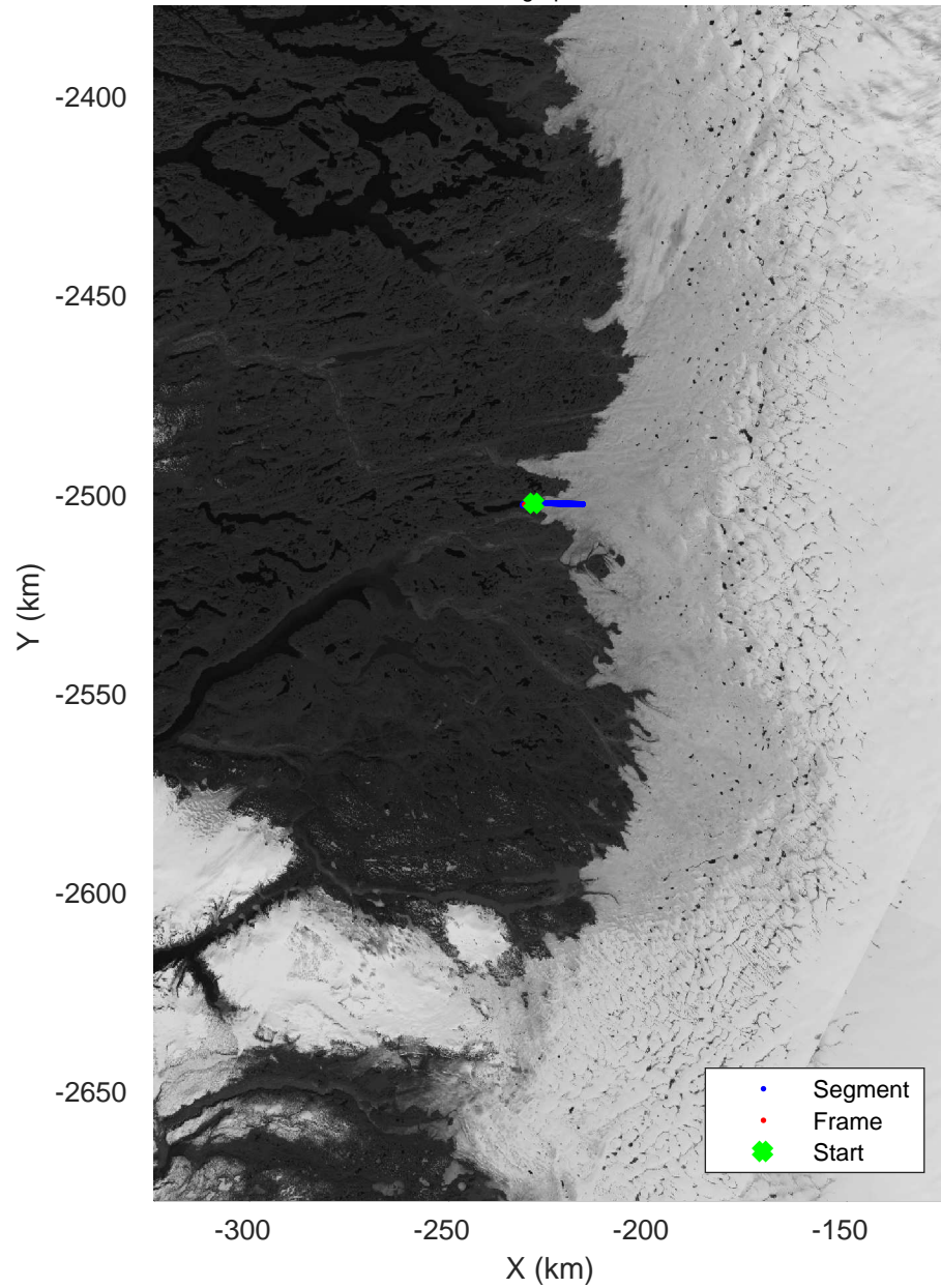
Bad line 3 20160417_03_006 Polar Stereograph 70N/-45E
