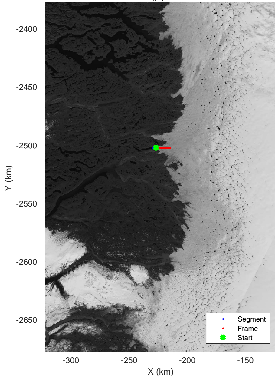
Bad line 3 20160417_03_004 Polar Stereograph 70N/-45E
