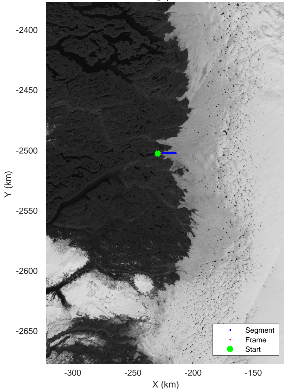
Bad line 3 20160417_03_001 Polar Stereograph 70N/-45E
