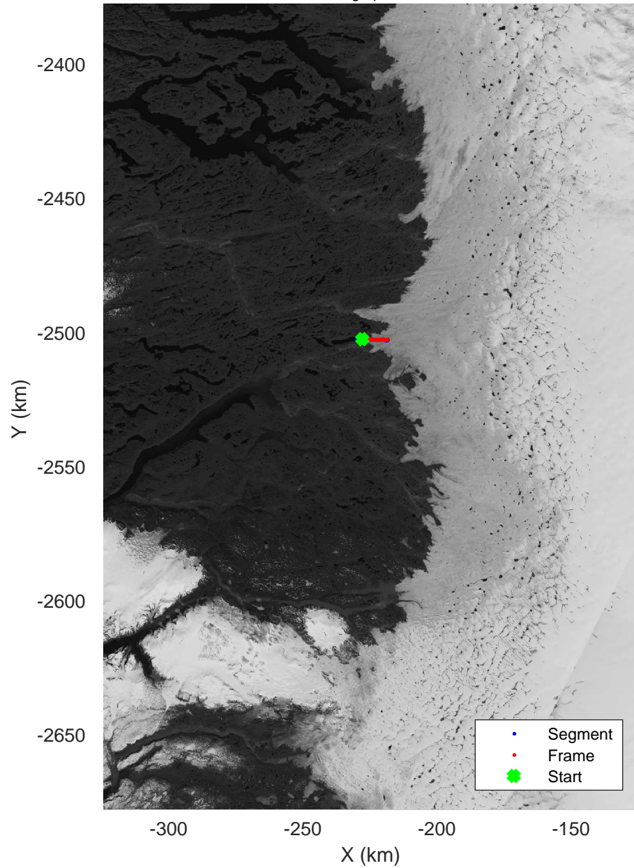
Medium line 1 20160416_01_004 Polar Stereograph 70N/-45E
