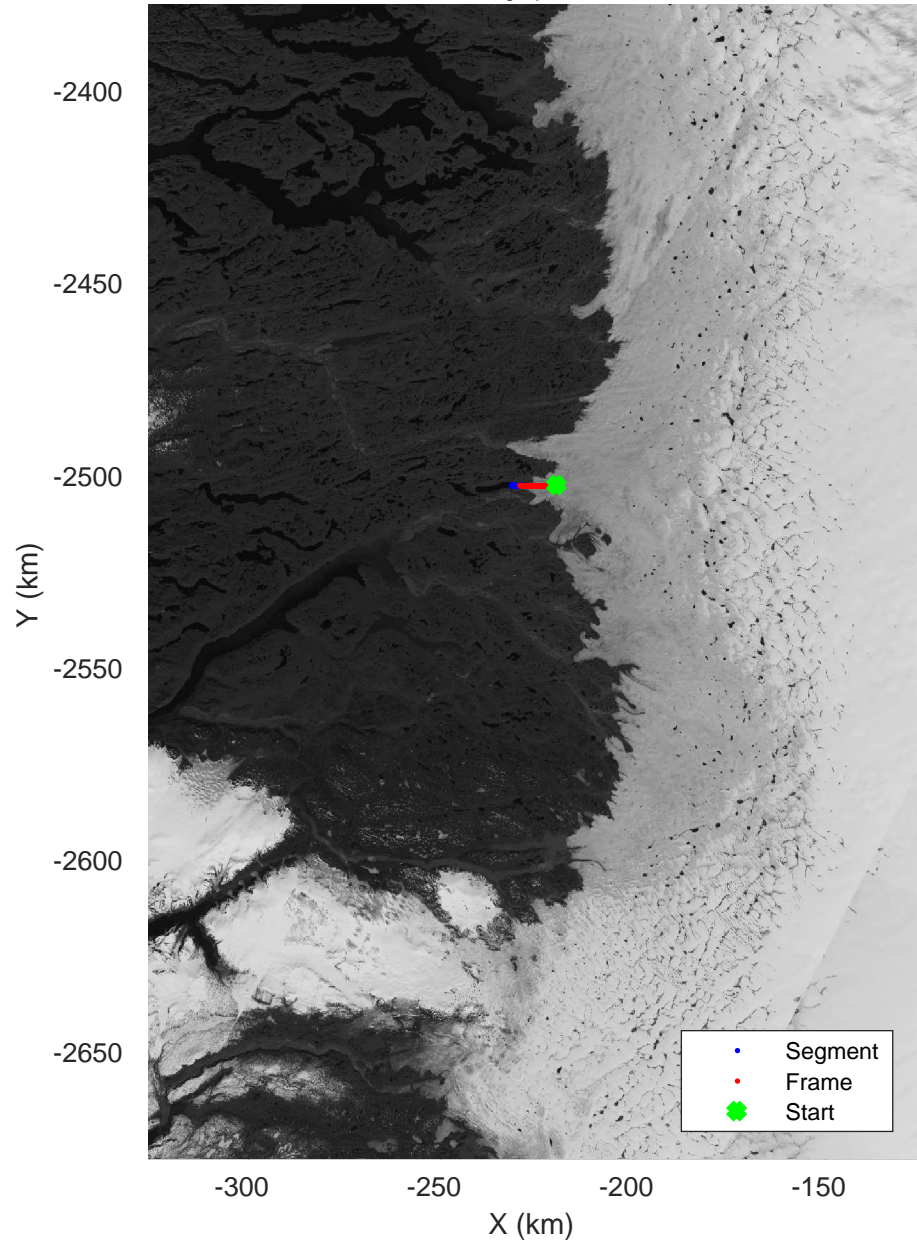
Medium line 1 20160416_01_003 Polar Stereograph 70N/-45E
