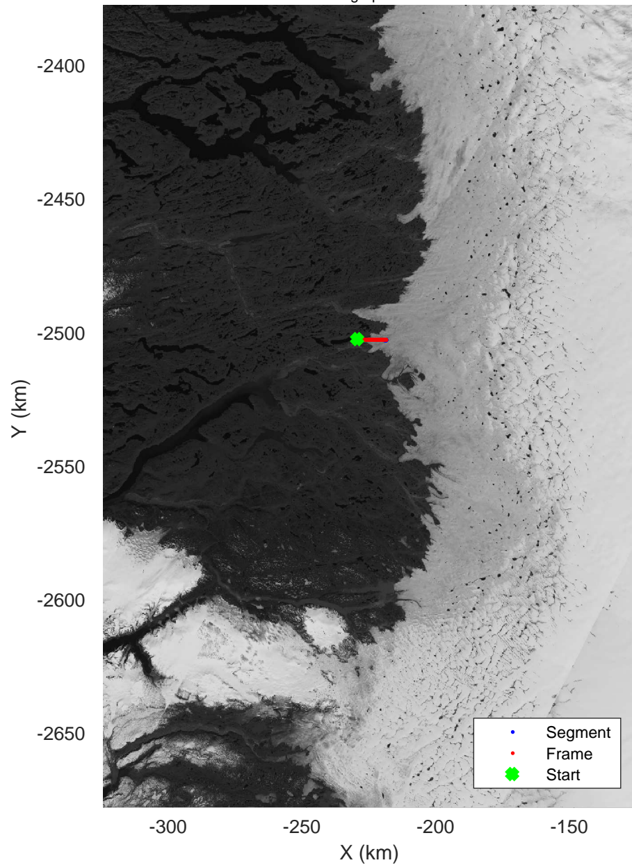
Medium line 1 20160416_01_002 Polar Stereograph 70N/-45E
