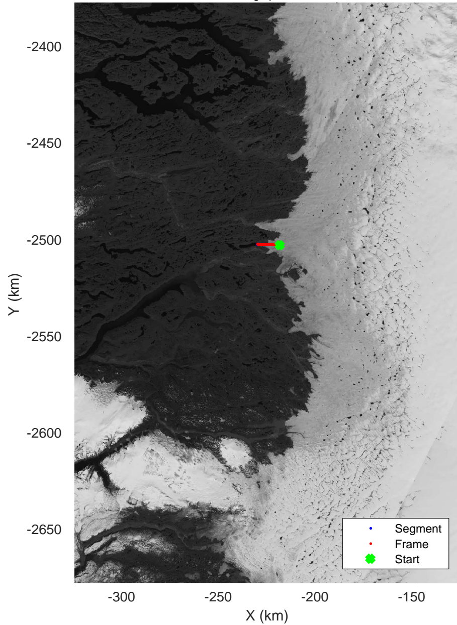
Medium line 1 20160416_01_005 Polar Stereograph 70N/-45E
