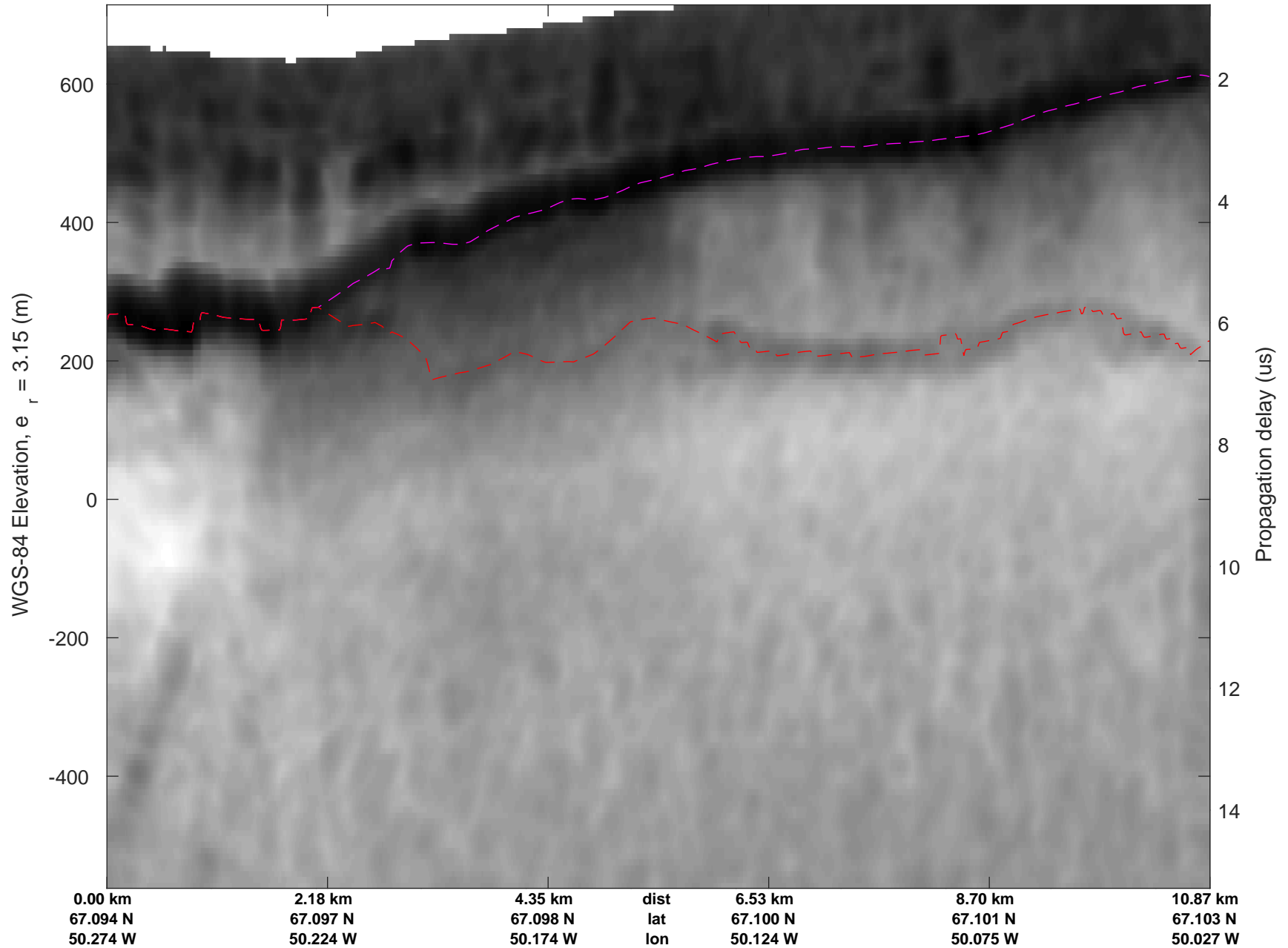
rds 2016_Greenland_G1XB: "Medium line 1" 20160416_01_002: 20:39:24.8 to 20:46:34.9 GPS
