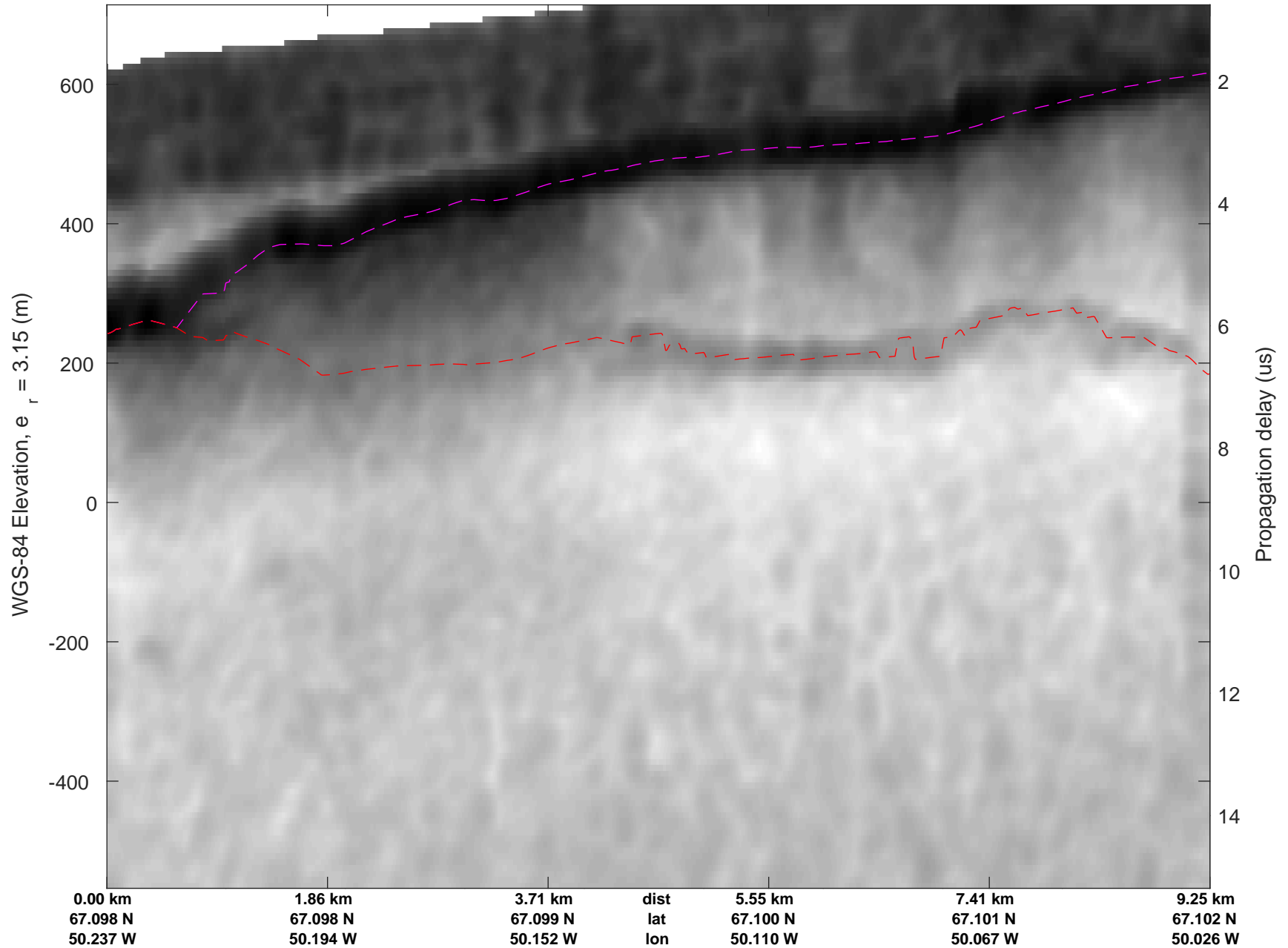
rds 2016_Greenland_G1XB: "Medium line 1" 20160416_01_004: 20:52:18.1 to 20:58:35.7 GPS
