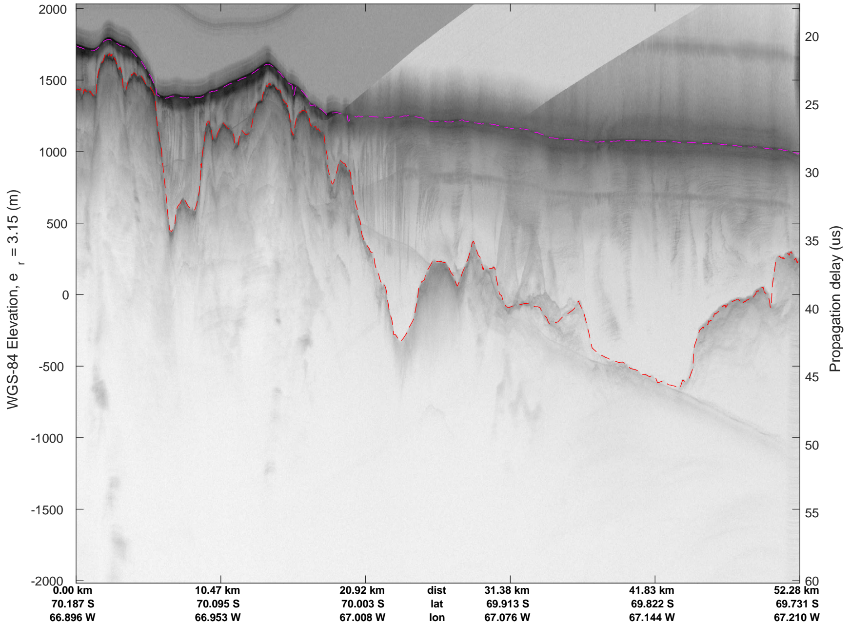
rds 2016_Antarctica_DC8: "South Peninsula" 20161114_04_062: 21:13:43.4 to 21:19:08.1 GPS
