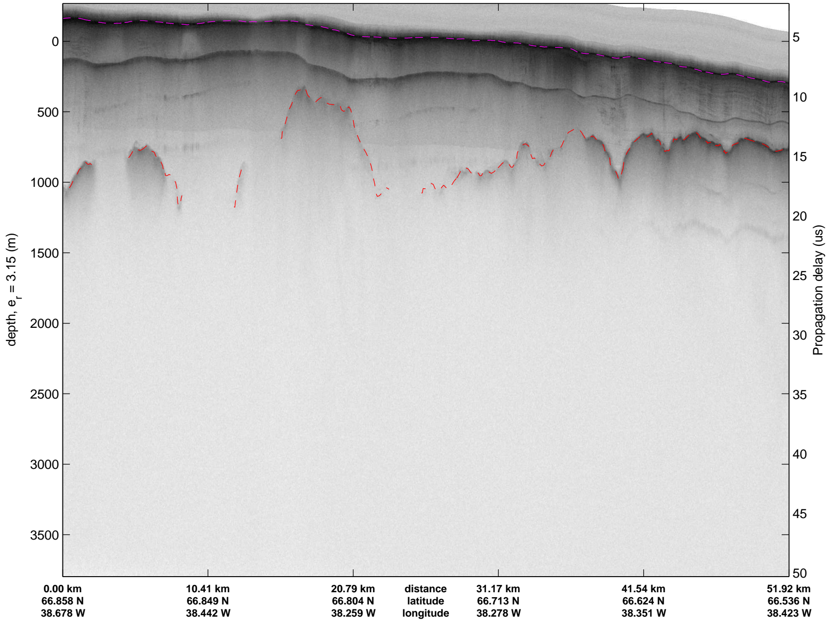
mcords3 2013_Greenland_P3: "F14: Southeast Glaciers 02" 20130409_01_011: 12:08:32.1 to 12:15:08.6 GPS
