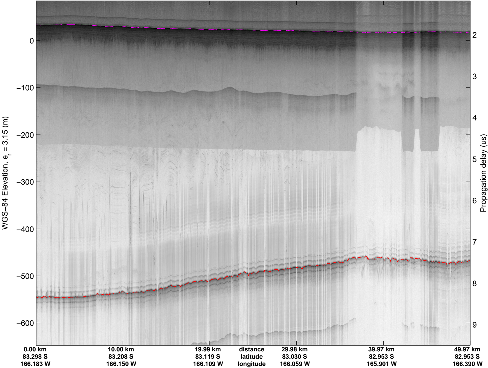
mcords4 2013_Antarctica_Basler: "Whillans Grounding Line South" 20131223_04_004: 02:37:48.6 to 02:48:05.9 GPS
