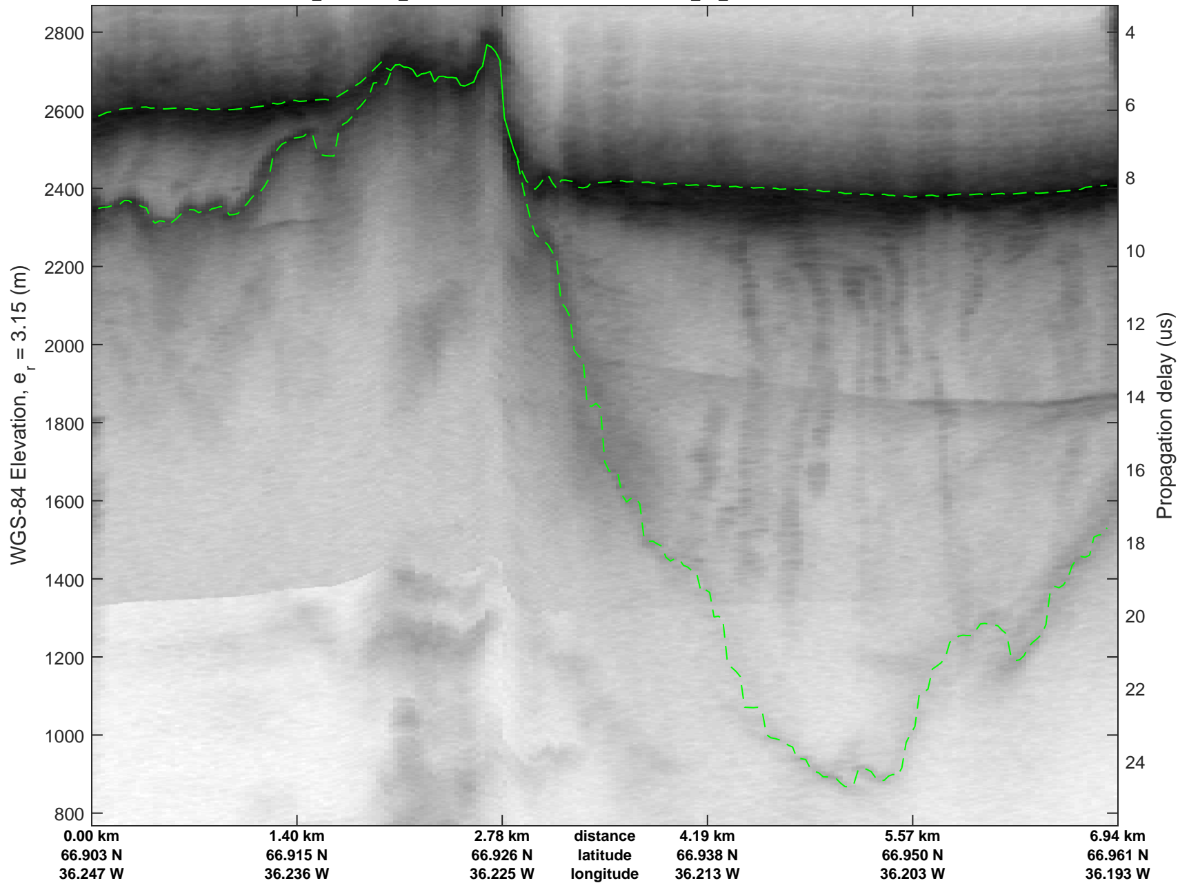
mcrds 2008_Greenland_TO: "Southeast Greenland" 20080730_04_001: 19:04:23.2 to 19:06:07.0 GPS
