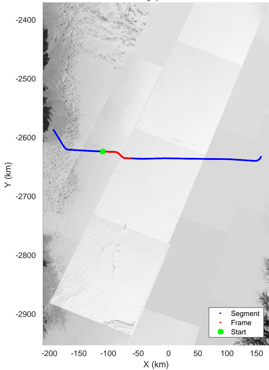
20020604_02_003 Polar Stereograph 70N/-45E
