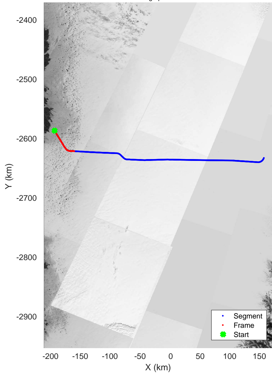
20020604_02_001 Polar Stereograph 70N/-45E
