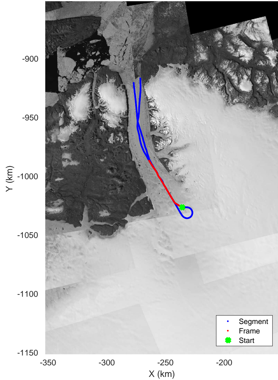
20020528_09_004 Polar Stereograph 70N/-45E
