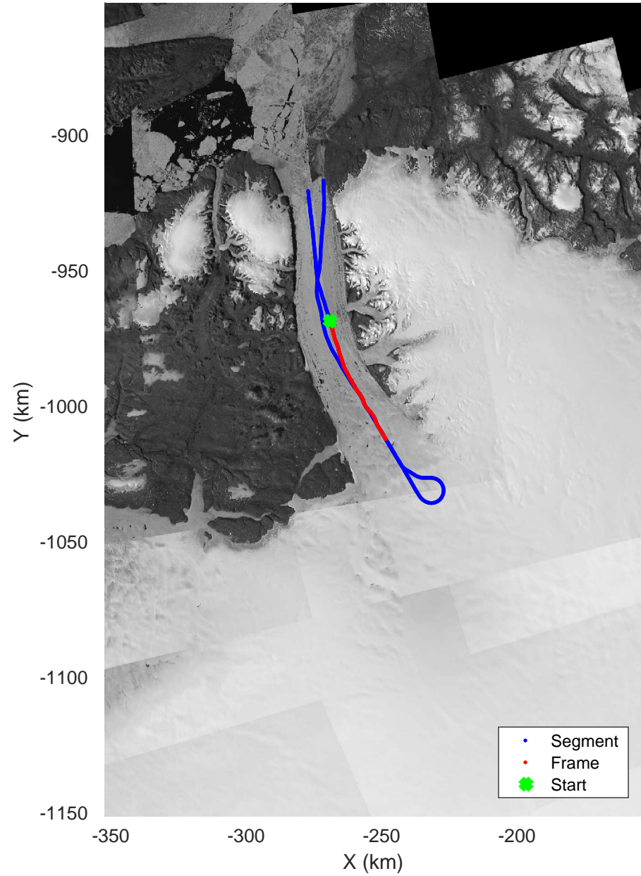
20020528_09_002 Polar Stereograph 70N/-45E
