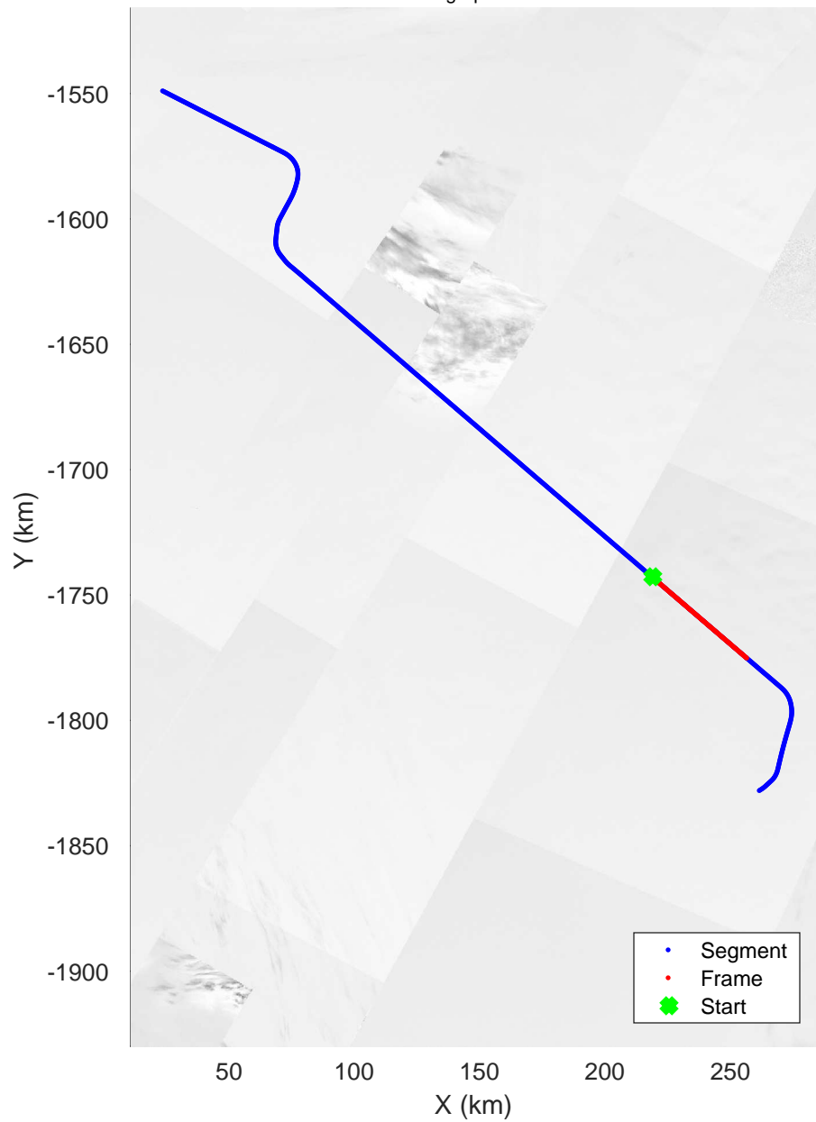
20020518_01_007 Polar Stereograph 70N/-45E
