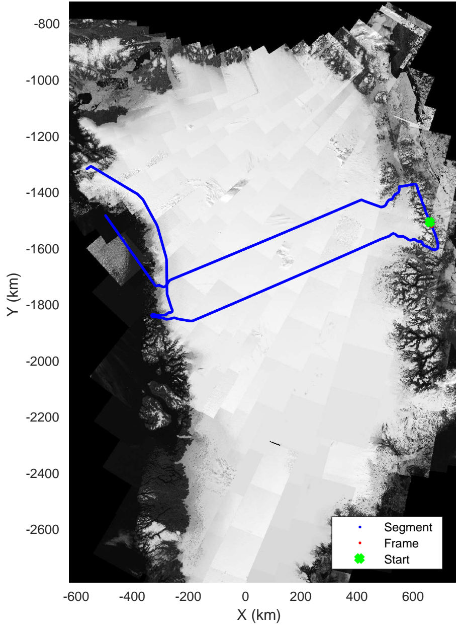
North Central Gap 03 20170410_01_077 Polar Stereograph 70N/-45E
