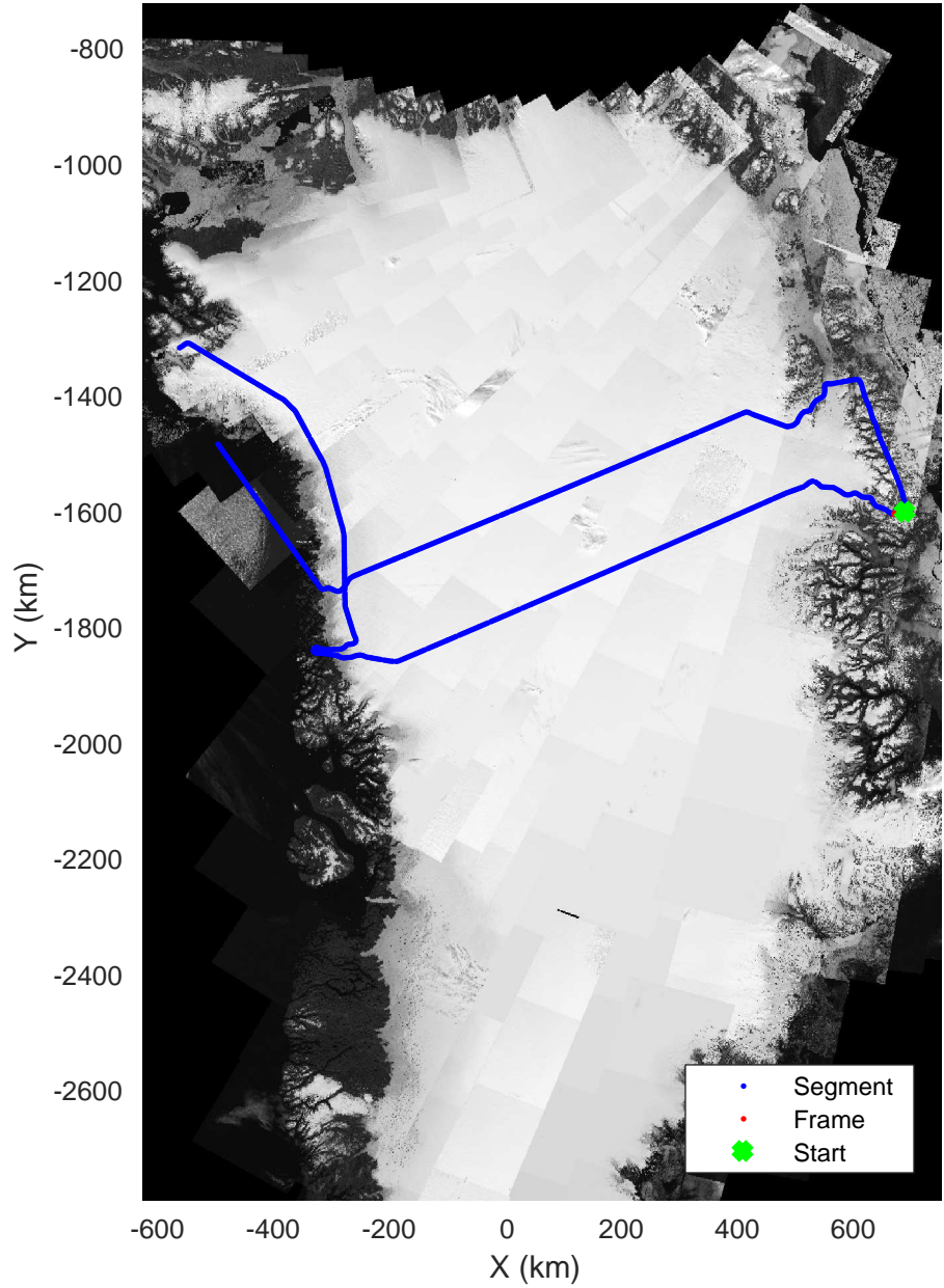
North Central Gap 03 20170410_01_082 Polar Stereograph 70N/-45E
