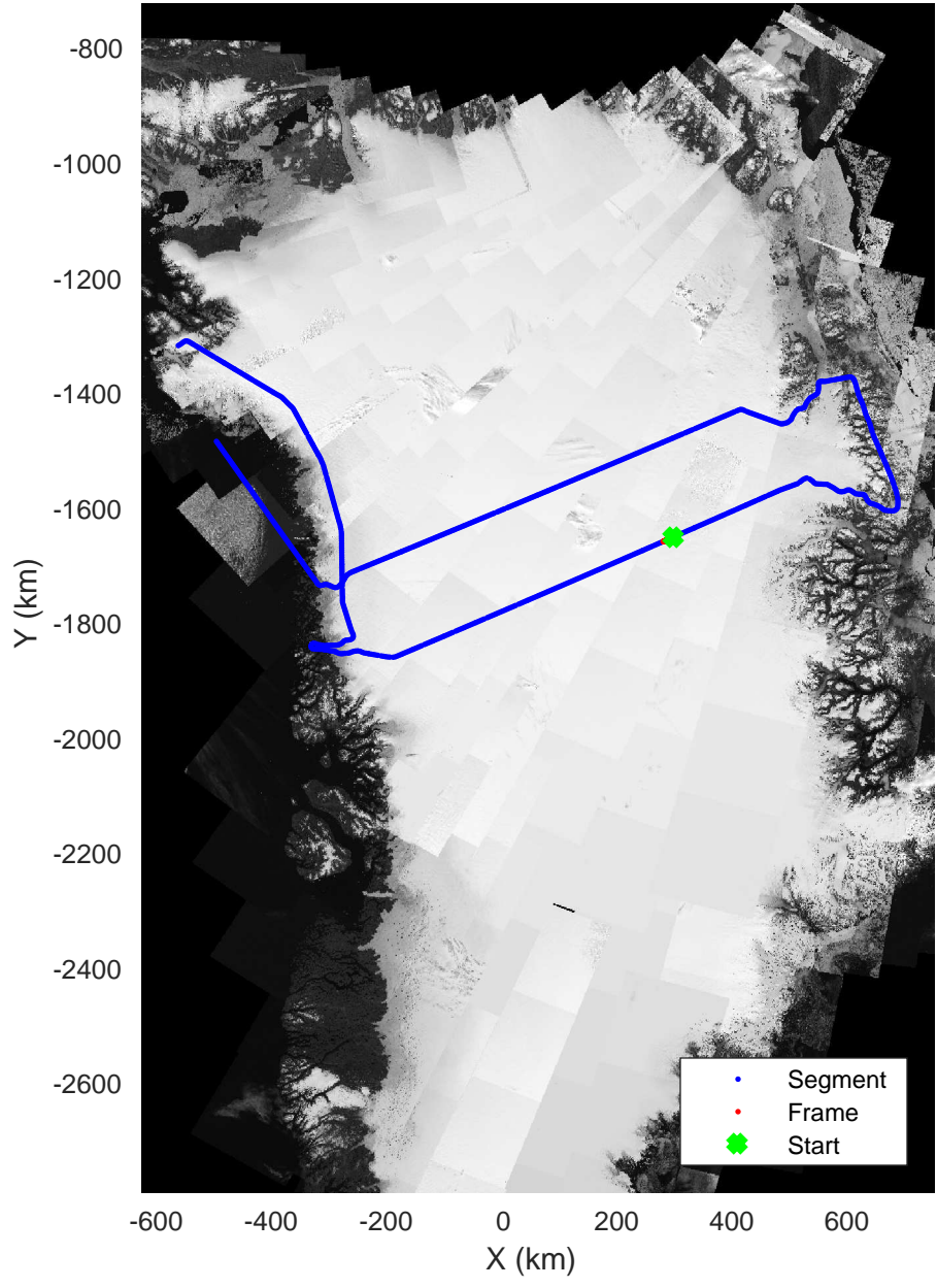
North Central Gap 03 20170410_01_104 Polar Stereograph 70N/-45E
