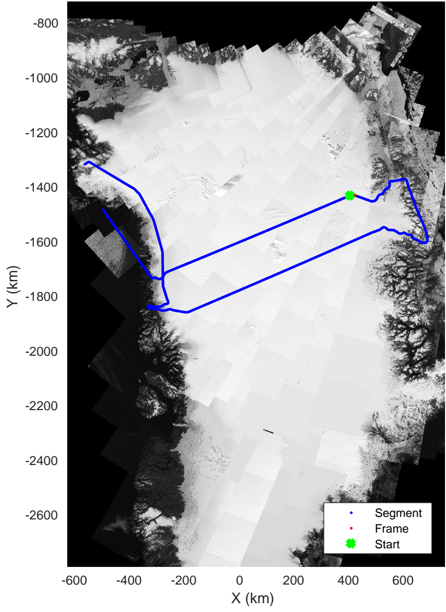
North Central Gap 03 20170410_01_057 Polar Stereograph 70N/-45E
