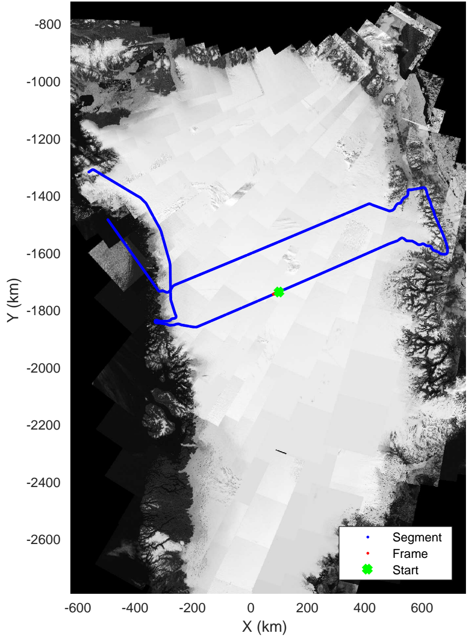
North Central Gap 03 20170410_01_115 Polar Stereograph 70N/-45E
