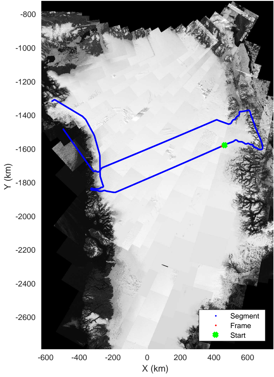
North Central Gap 03 20170410_01_095 Polar Stereograph 70N/-45E
