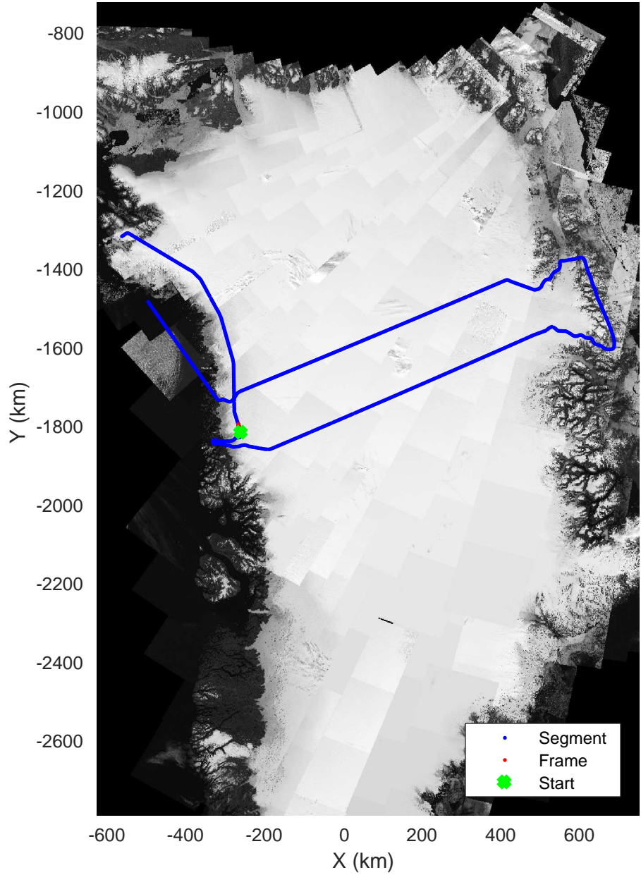
North Central Gap 03 20170410_01_143 Polar Stereograph 70N/-45E
