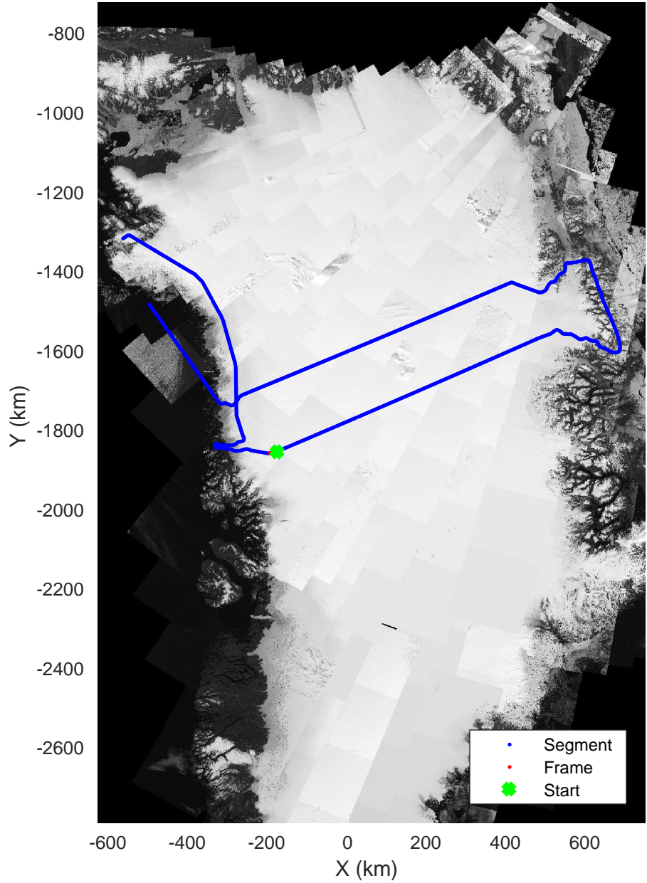
North Central Gap 03 20170410_01_130 Polar Stereograph 70N/-45E
