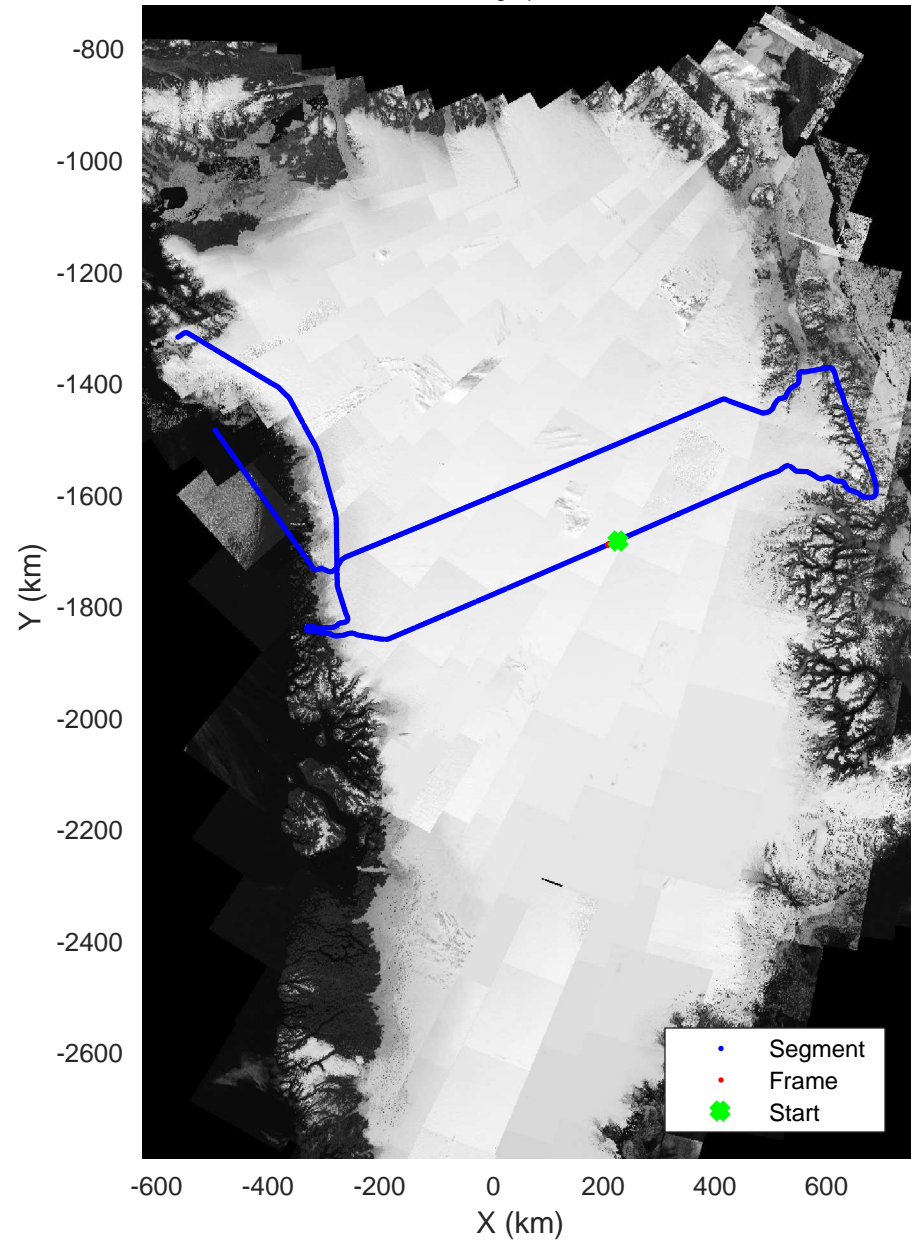
North Central Gap 03 20170410_01_108 Polar Stereograph 70N/-45E
