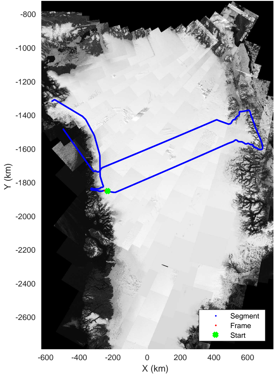
North Central Gap 03 20170410_01_133 Polar Stereograph 70N/-45E
