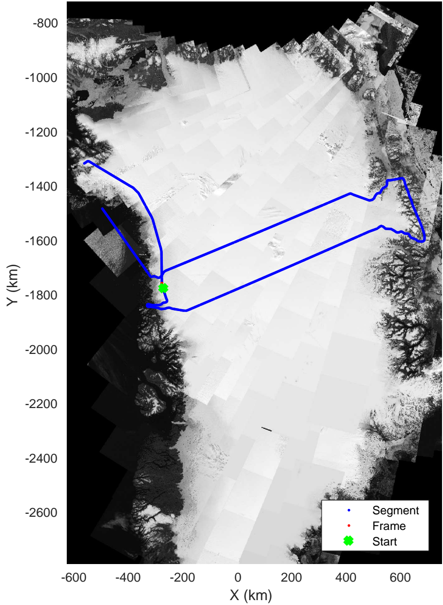
North Central Gap 03 20170410_01_145 Polar Stereograph 70N/-45E
