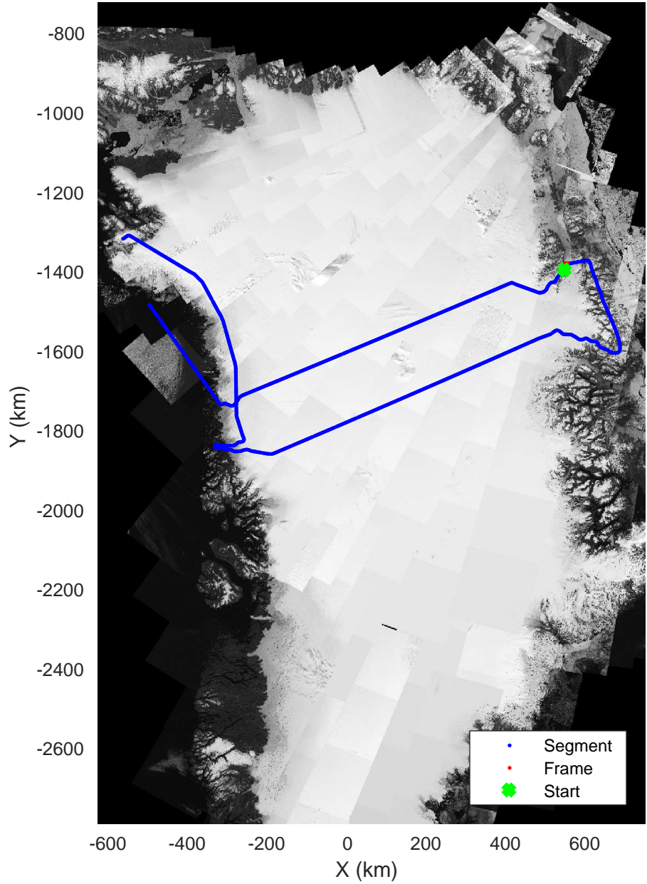
North Central Gap 03 20170410_01_066 Polar Stereograph 70N/-45E
