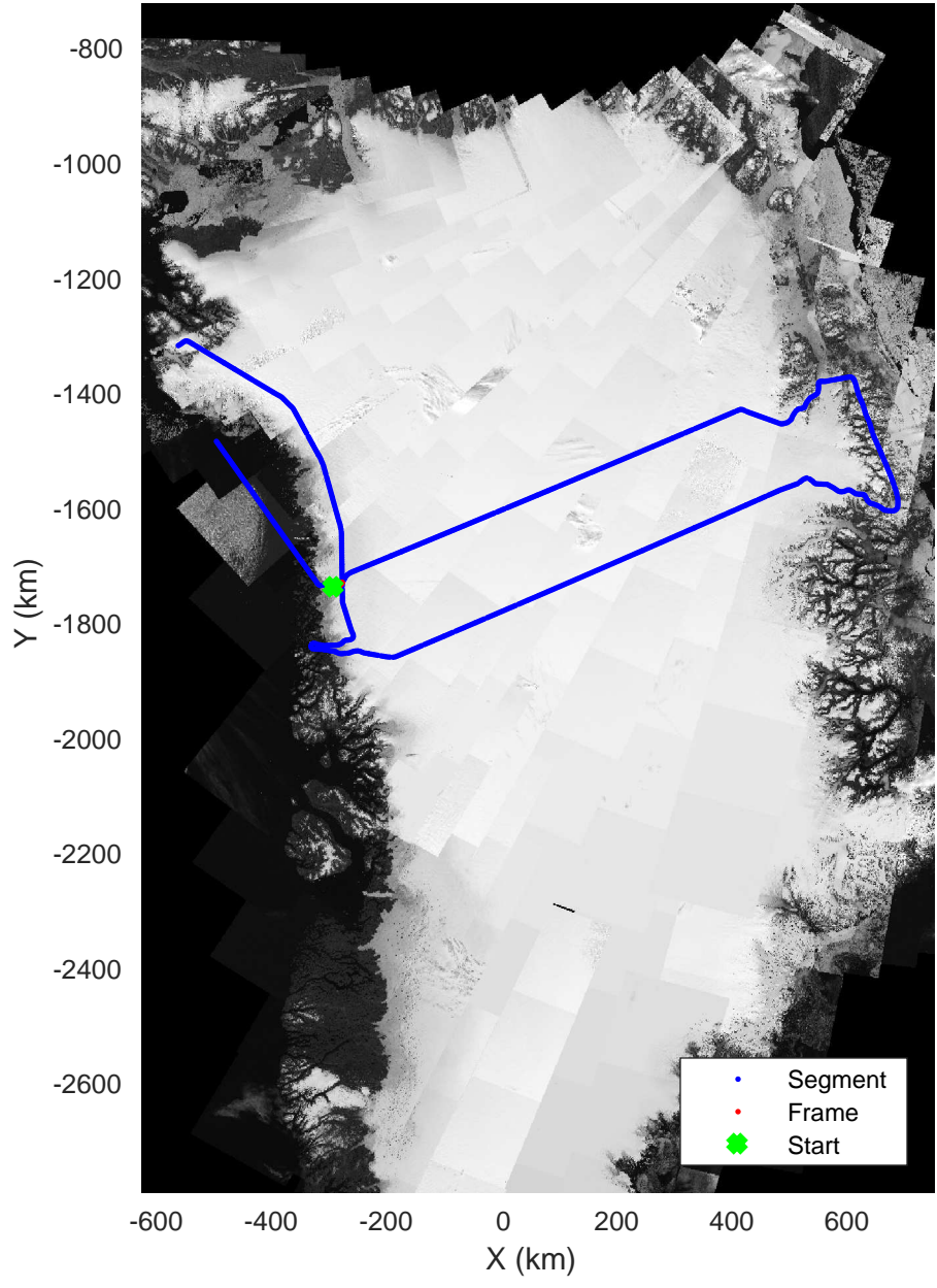
North Central Gap 03 20170410_01_018 Polar Stereograph 70N/-45E
