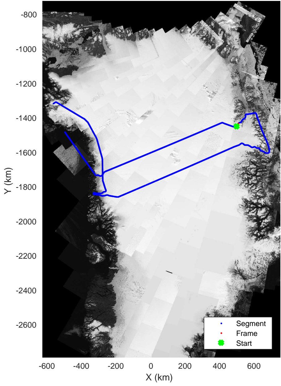
North Central Gap 03 20170410_01_062 Polar Stereograph 70N/-45E
