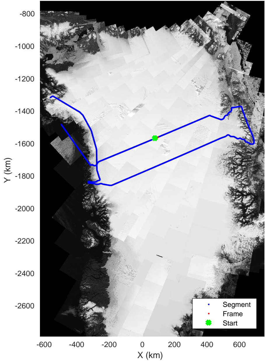
North Central Gap 03 20170410_01_039 Polar Stereograph 70N/-45E
