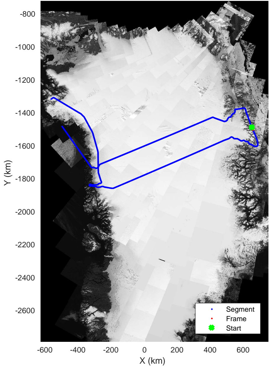
North Central Gap 03 20170410_01_076 Polar Stereograph 70N/-45E
