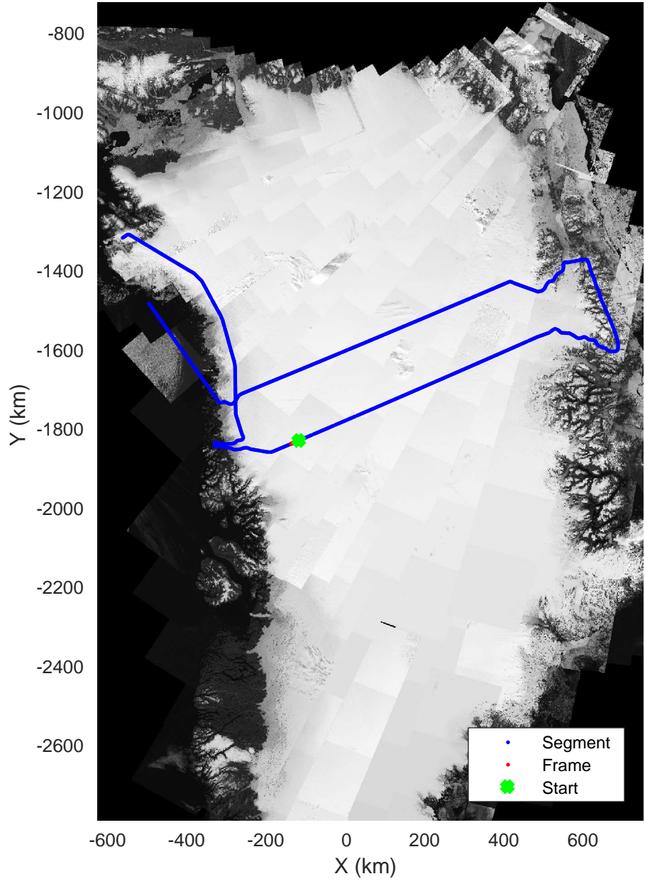
North Central Gap 03 20170410_01_127 Polar Stereograph 70N/-45E
