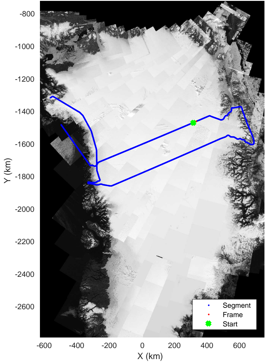
North Central Gap 03 20170410_01_052 Polar Stereograph 70N/-45E
