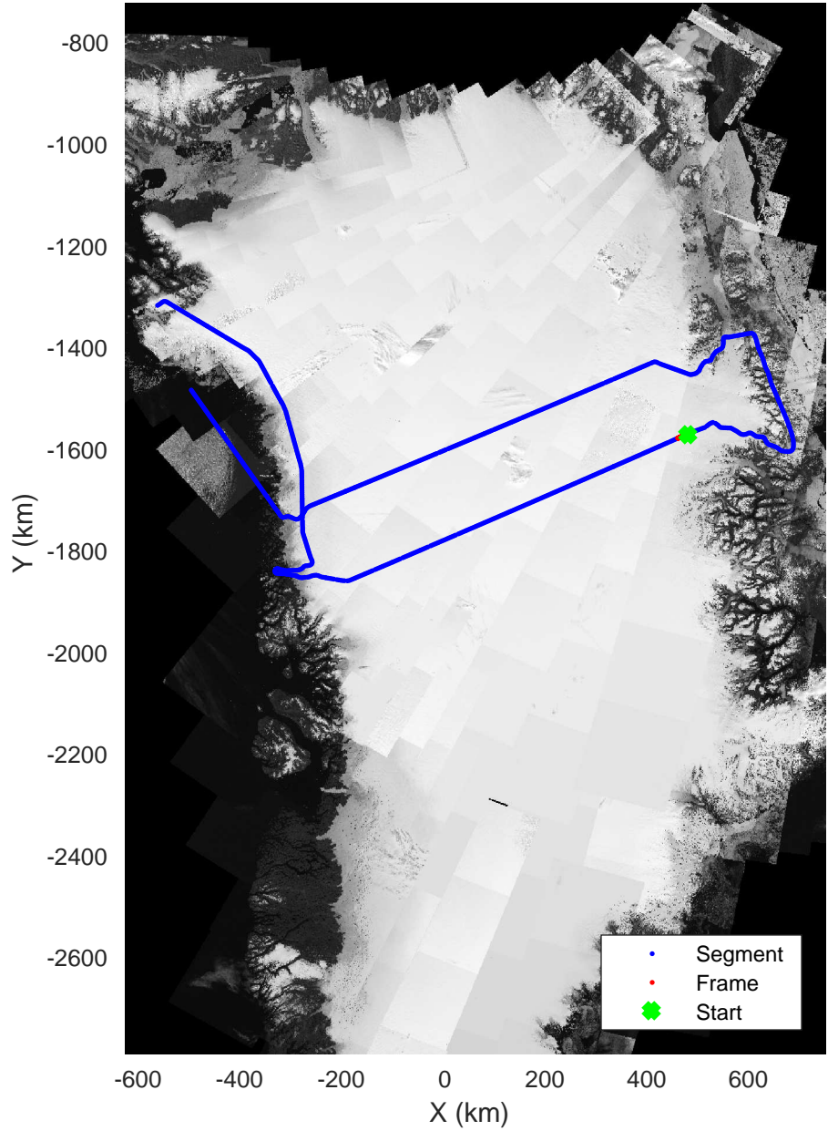
North Central Gap 03 20170410_01_094 Polar Stereograph 70N/-45E
