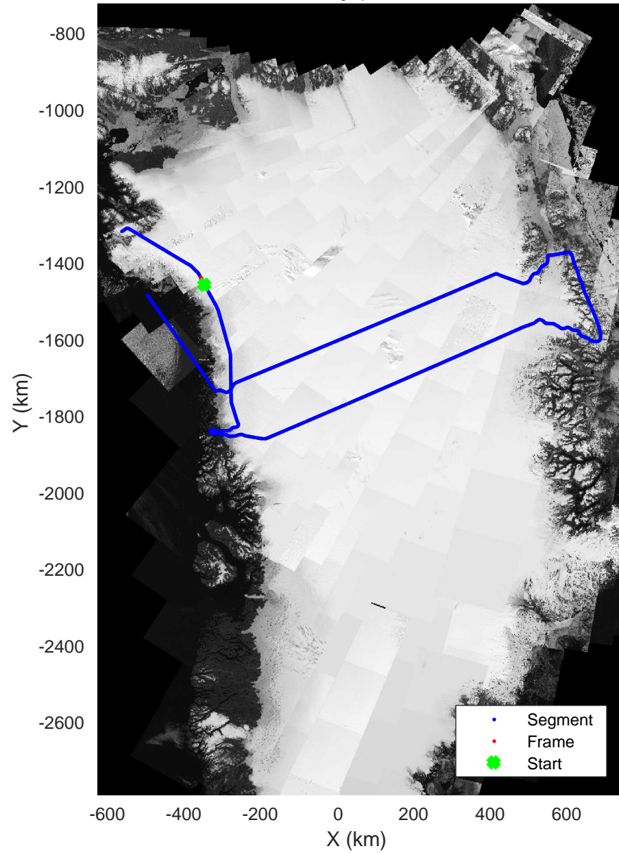
North Central Gap 03 20170410_01_162 Polar Stereograph 70N/-45E
