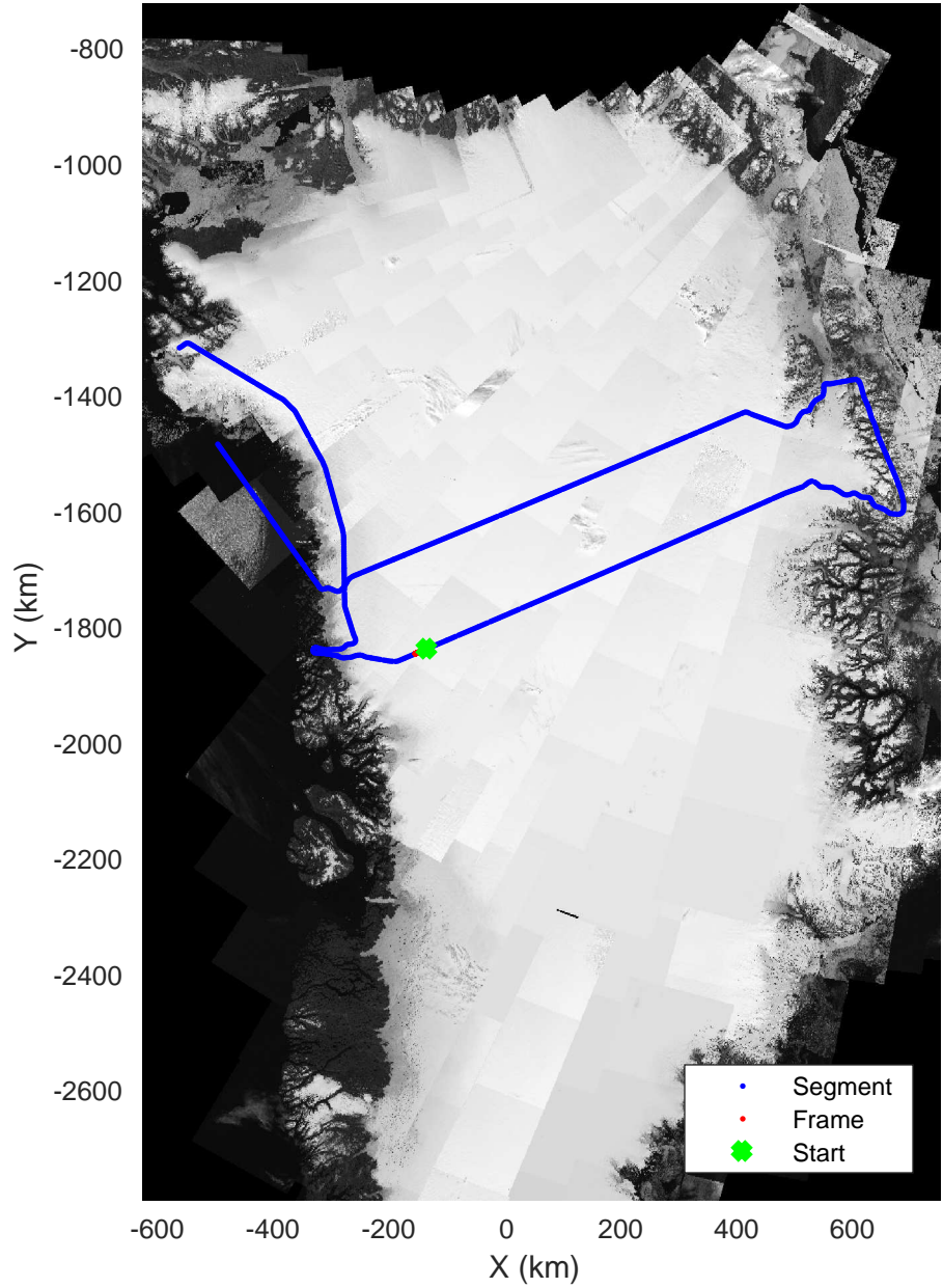
North Central Gap 03 20170410_01_128 Polar Stereograph 70N/-45E
