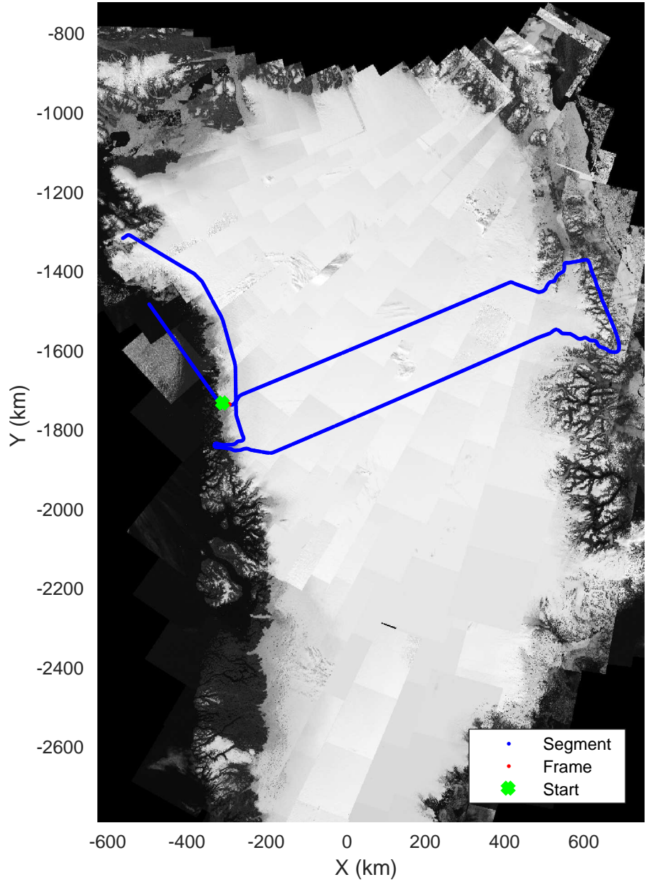
North Central Gap 03 20170410_01_017 Polar Stereograph 70N/-45E
