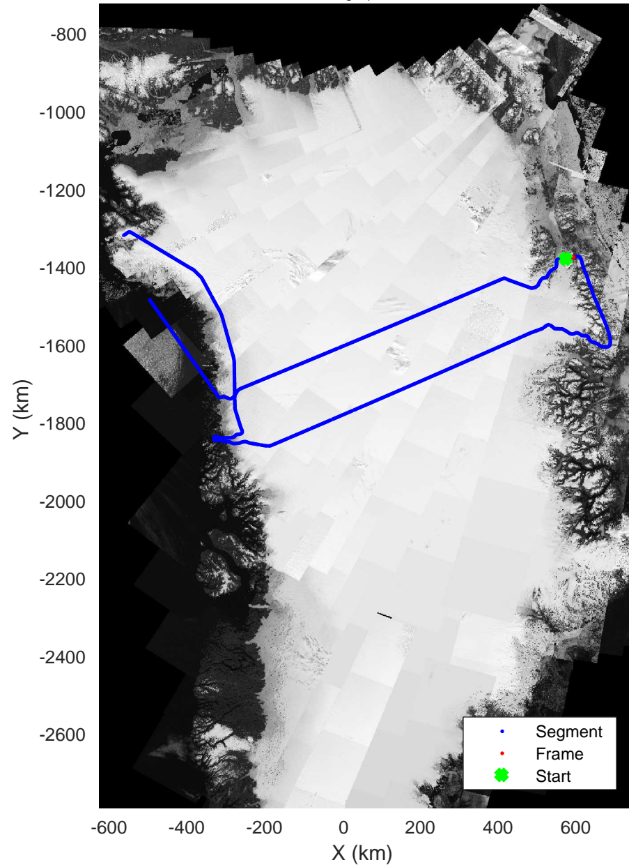
North Central Gap 03 20170410_01_068 Polar Stereograph 70N/-45E
