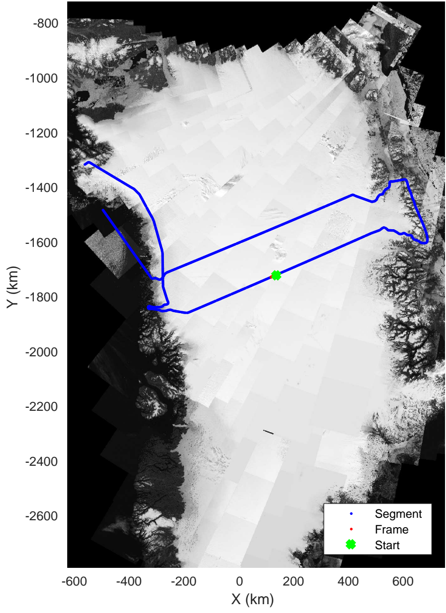
North Central Gap 03 20170410_01_113 Polar Stereograph 70N/-45E
