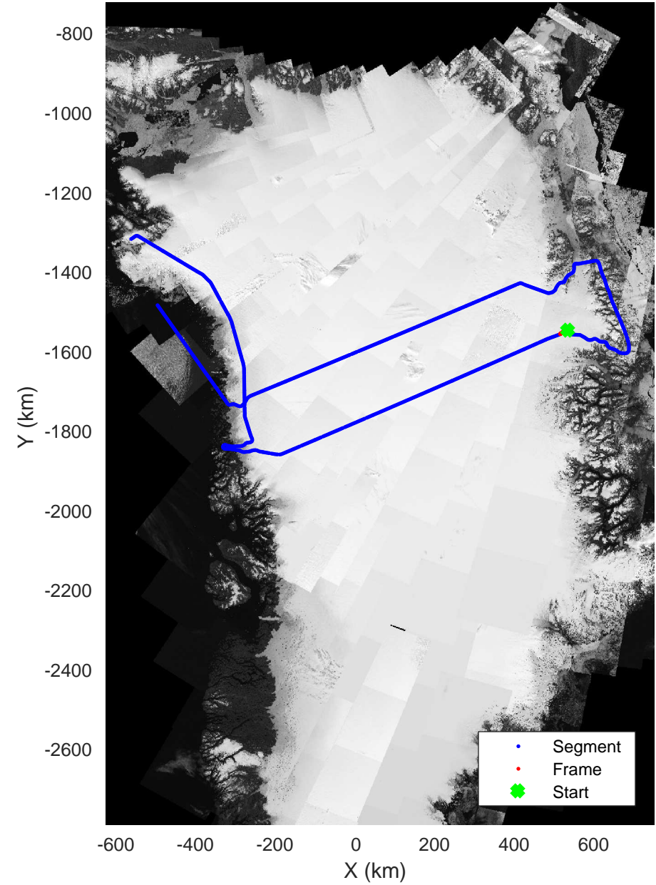
North Central Gap 03 20170410_01_091 Polar Stereograph 70N/-45E
