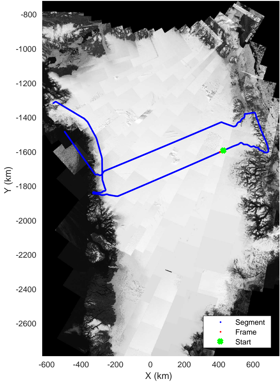
North Central Gap 03 20170410_01_097 Polar Stereograph 70N/-45E
