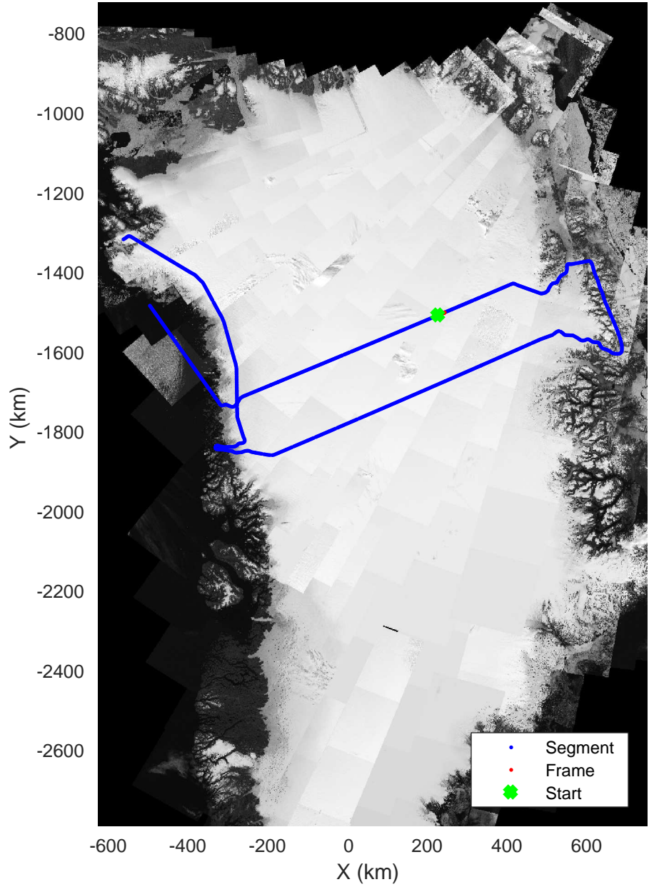
North Central Gap 03 20170410_01_047 Polar Stereograph 70N/-45E
