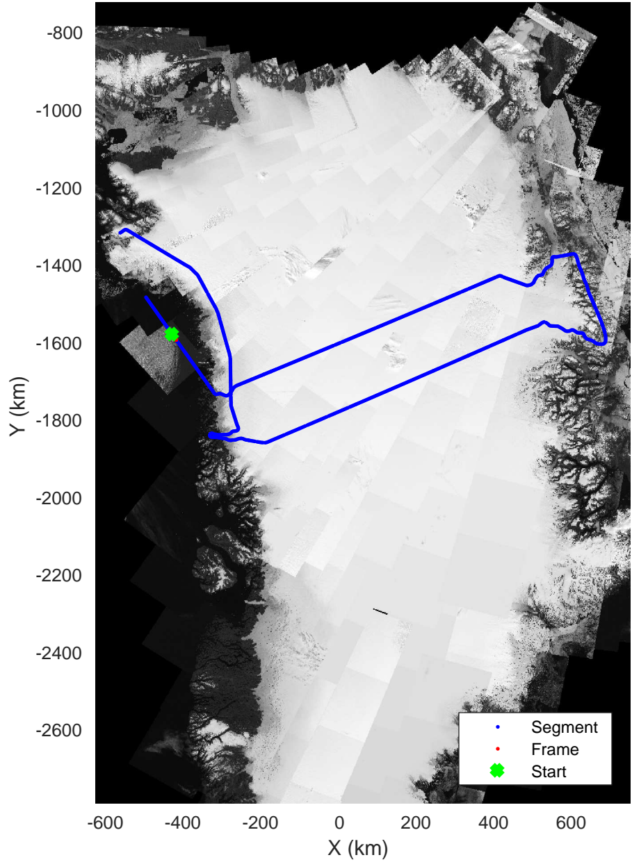
North Central Gap 03 20170410_01_007 Polar Stereograph 70N/-45E
