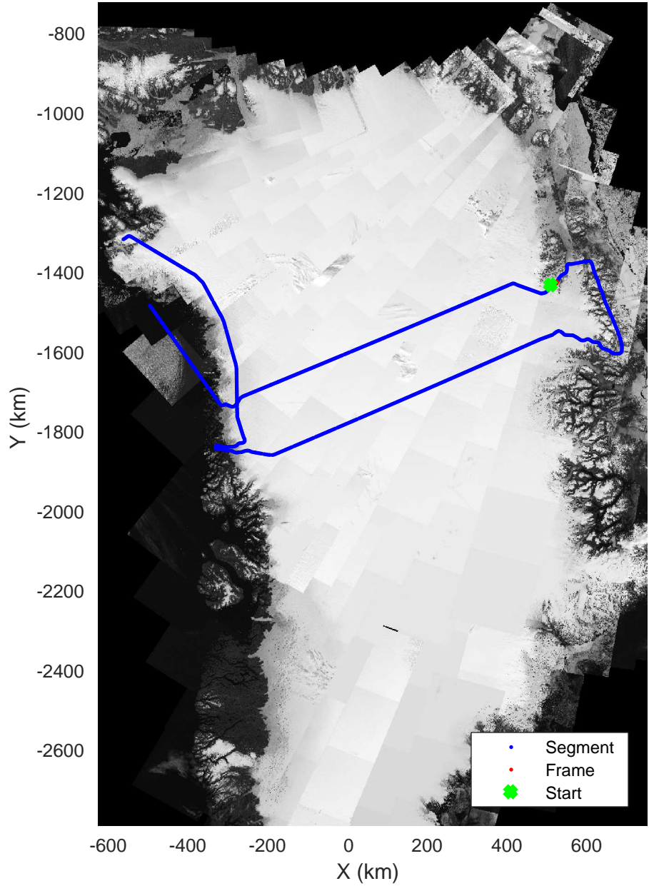
North Central Gap 03 20170410_01_063 Polar Stereograph 70N/-45E
