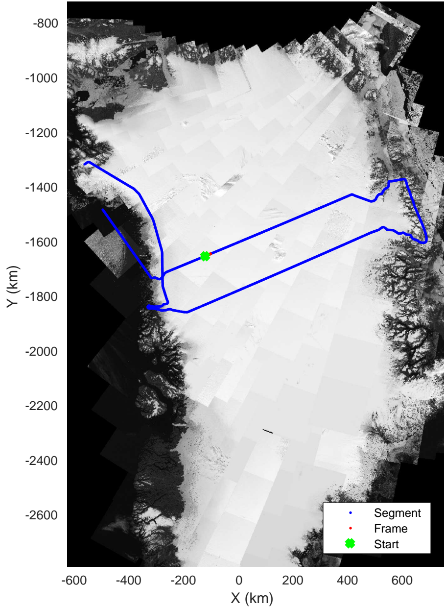
North Central Gap 03 20170410_01_028 Polar Stereograph 70N/-45E
