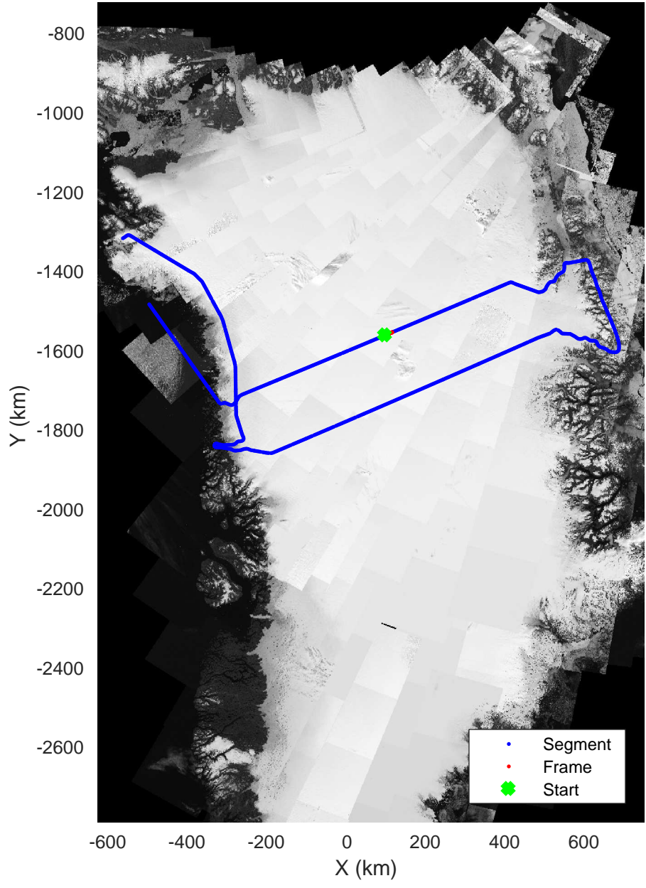
North Central Gap 03 20170410_01_040 Polar Stereograph 70N/-45E
