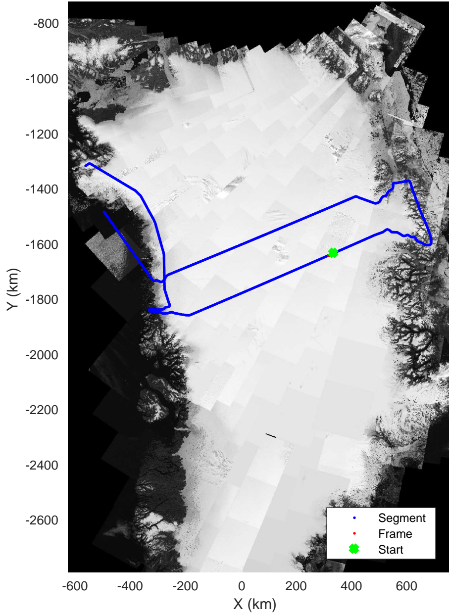
North Central Gap 03 20170410_01_102 Polar Stereograph 70N/-45E
