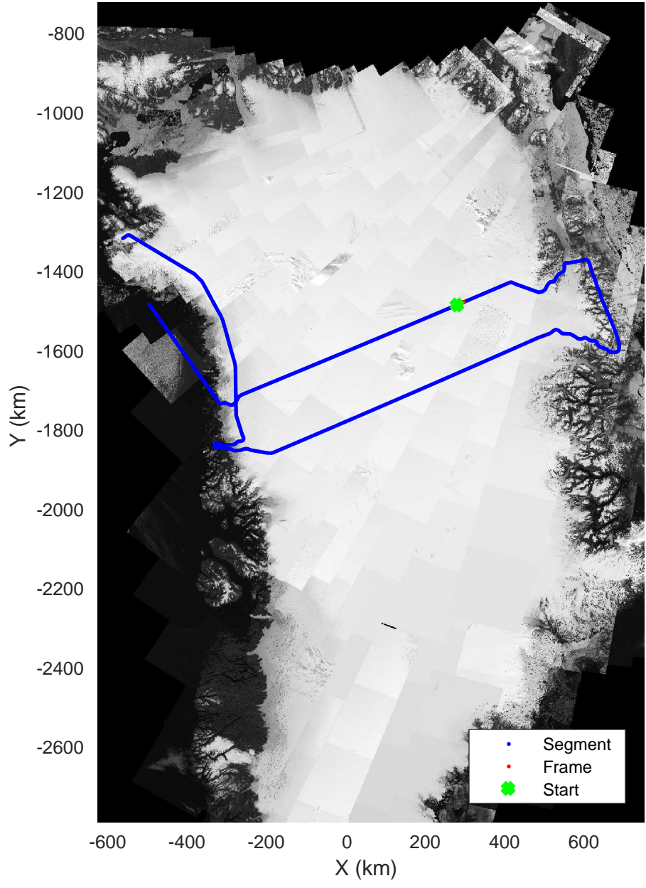
North Central Gap 03 20170410_01_050 Polar Stereograph 70N/-45E
