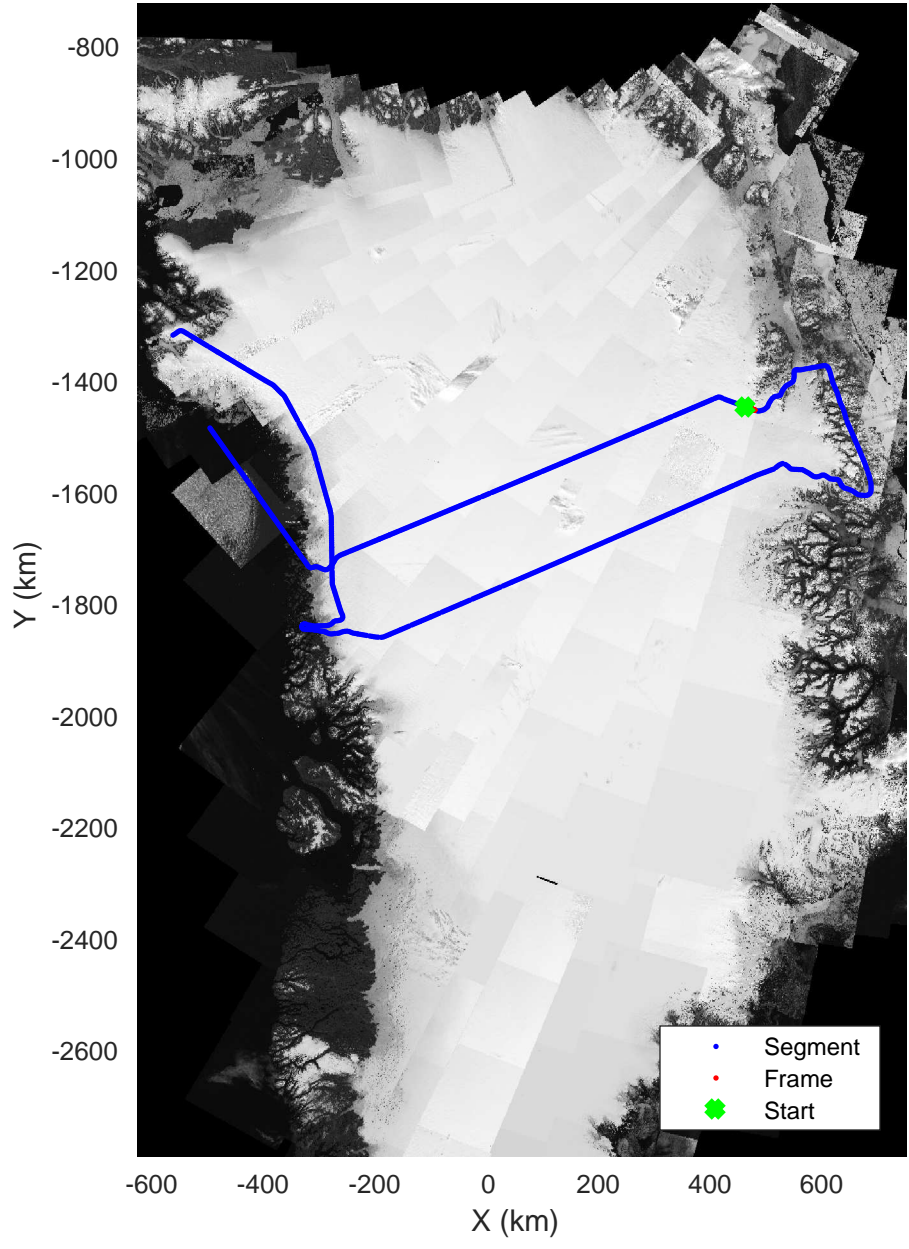
North Central Gap 03 20170410_01_060 Polar Stereograph 70N/-45E
