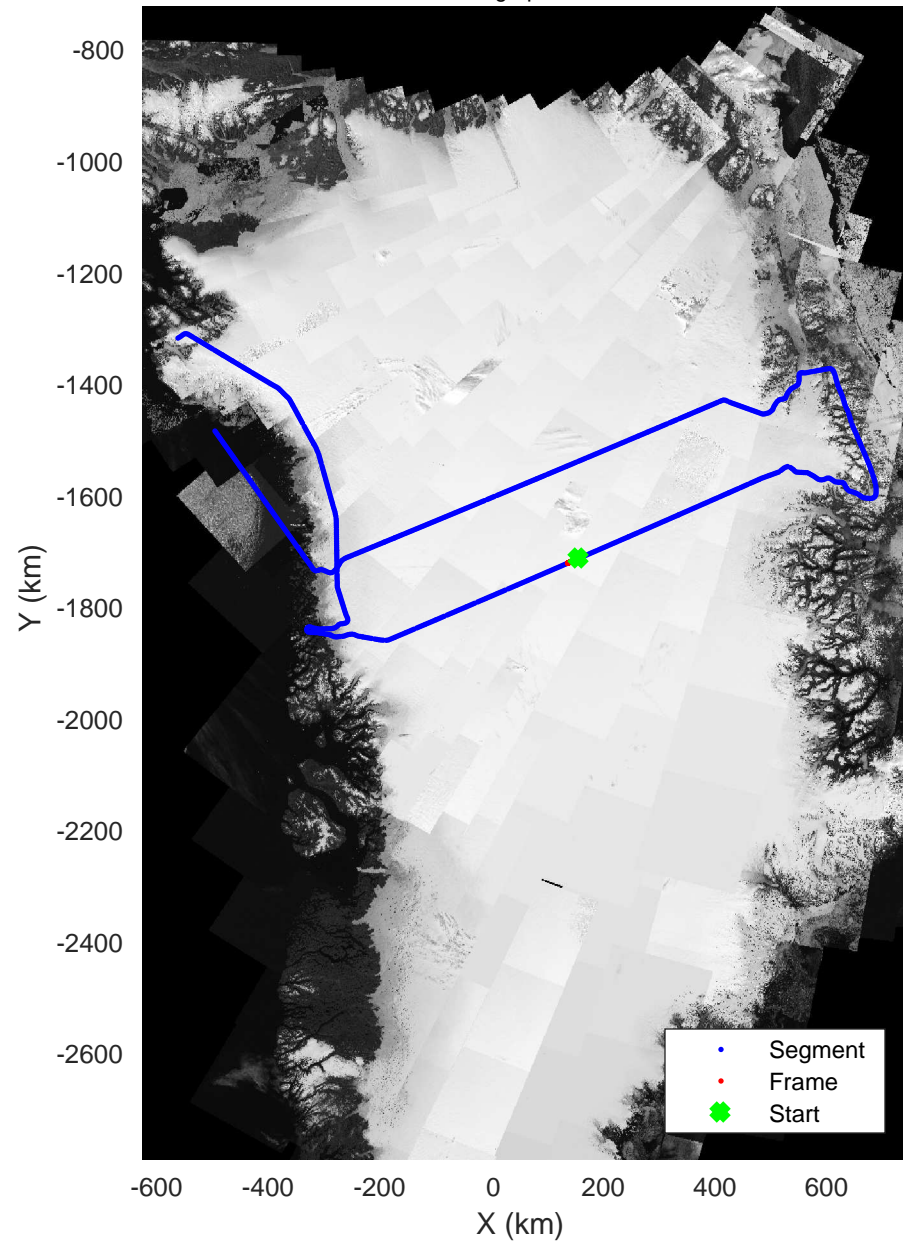
North Central Gap 03 20170410_01_112 Polar Stereograph 70N/-45E
