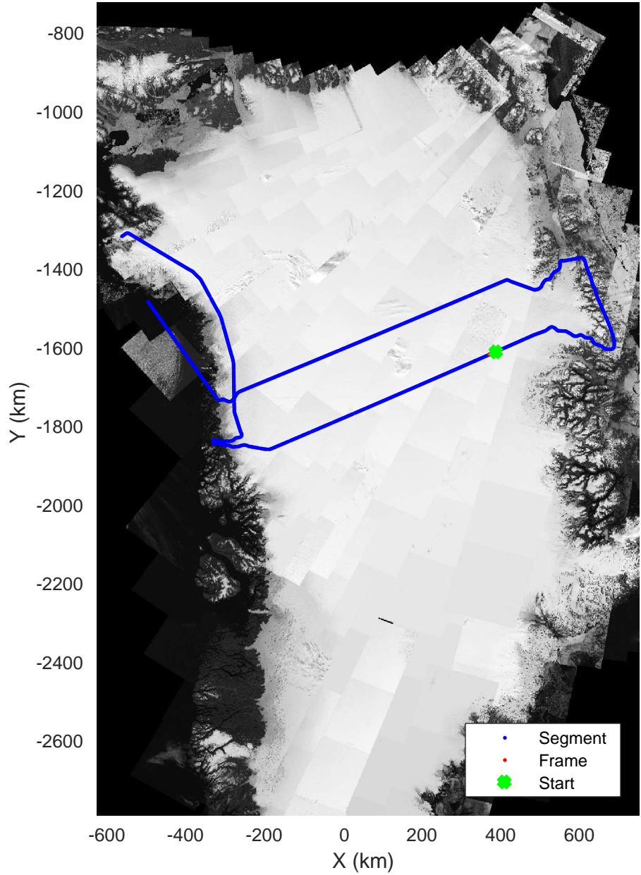
North Central Gap 03 20170410_01_099 Polar Stereograph 70N/-45E
