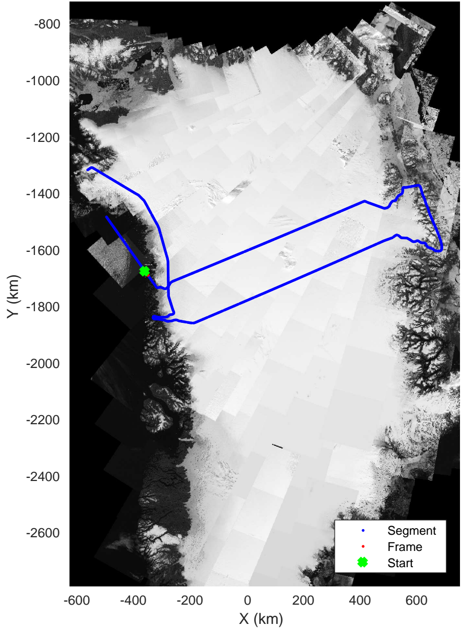
North Central Gap 03 20170410_01_013 Polar Stereograph 70N/-45E
