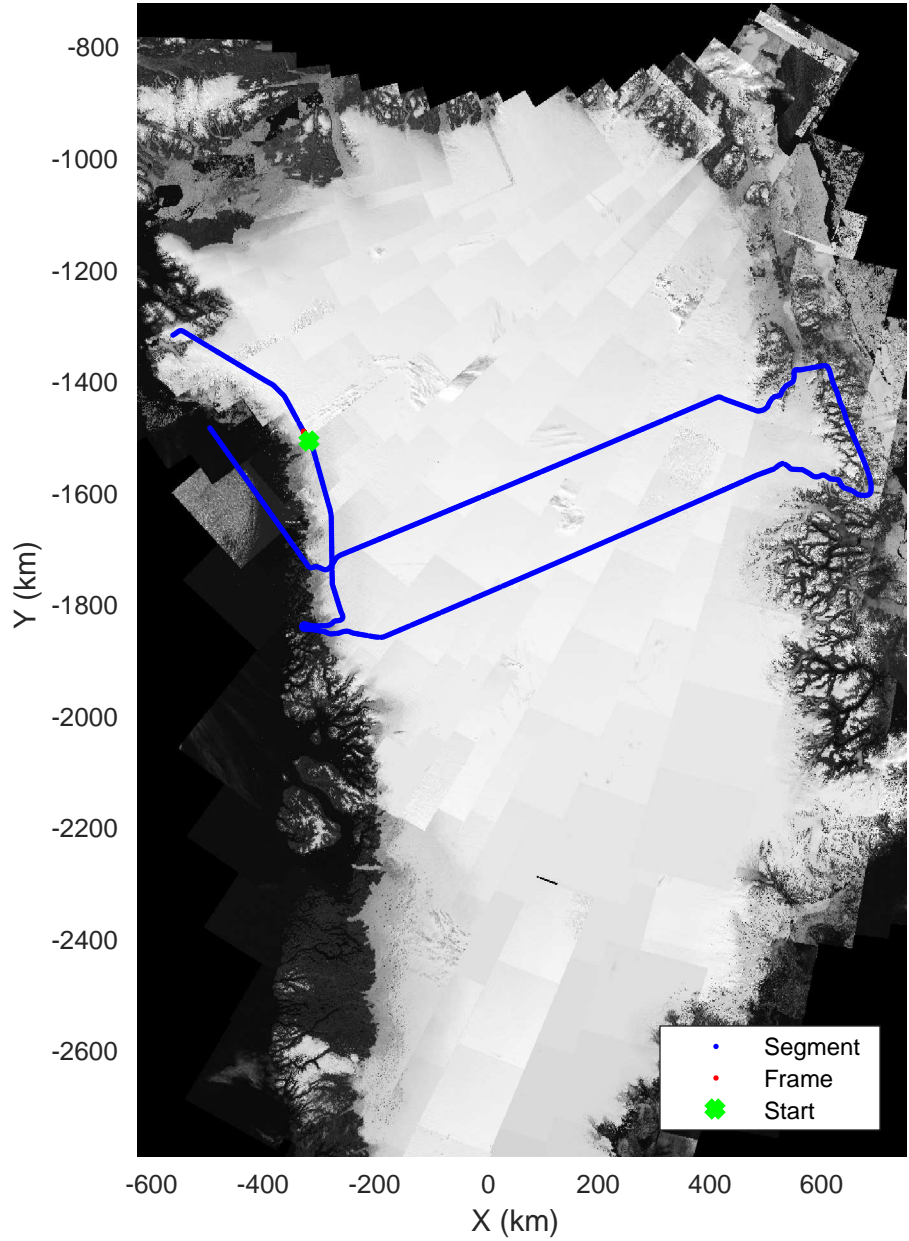
North Central Gap 03 20170410_01_159 Polar Stereograph 70N/-45E
