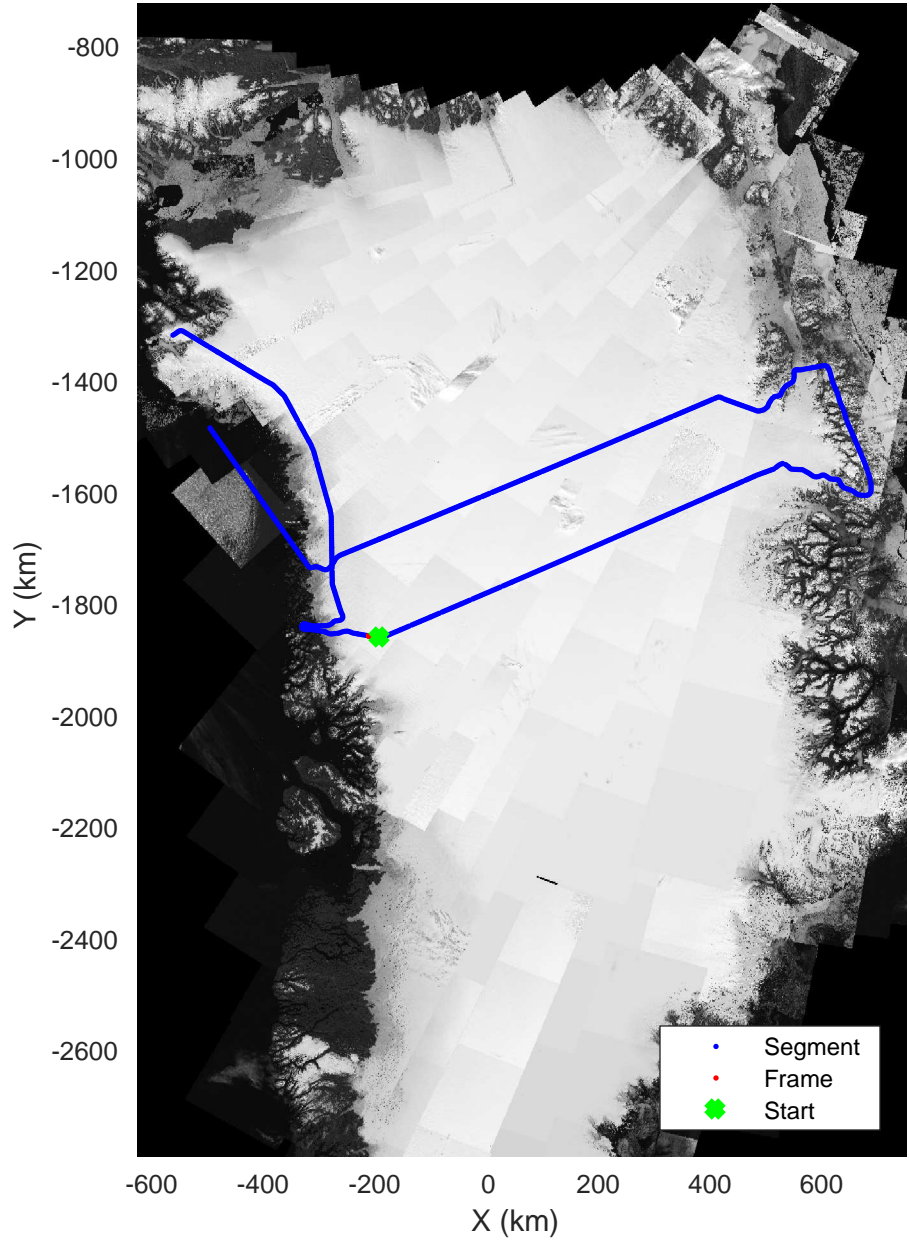
North Central Gap 03 20170410_01_131 Polar Stereograph 70N/-45E
