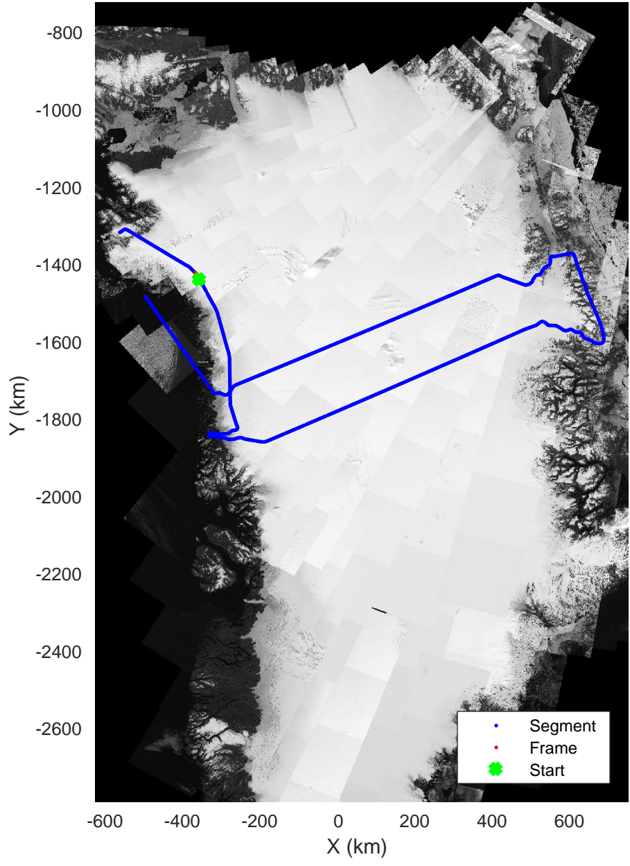
North Central Gap 03 20170410_01_163 Polar Stereograph 70N/-45E
