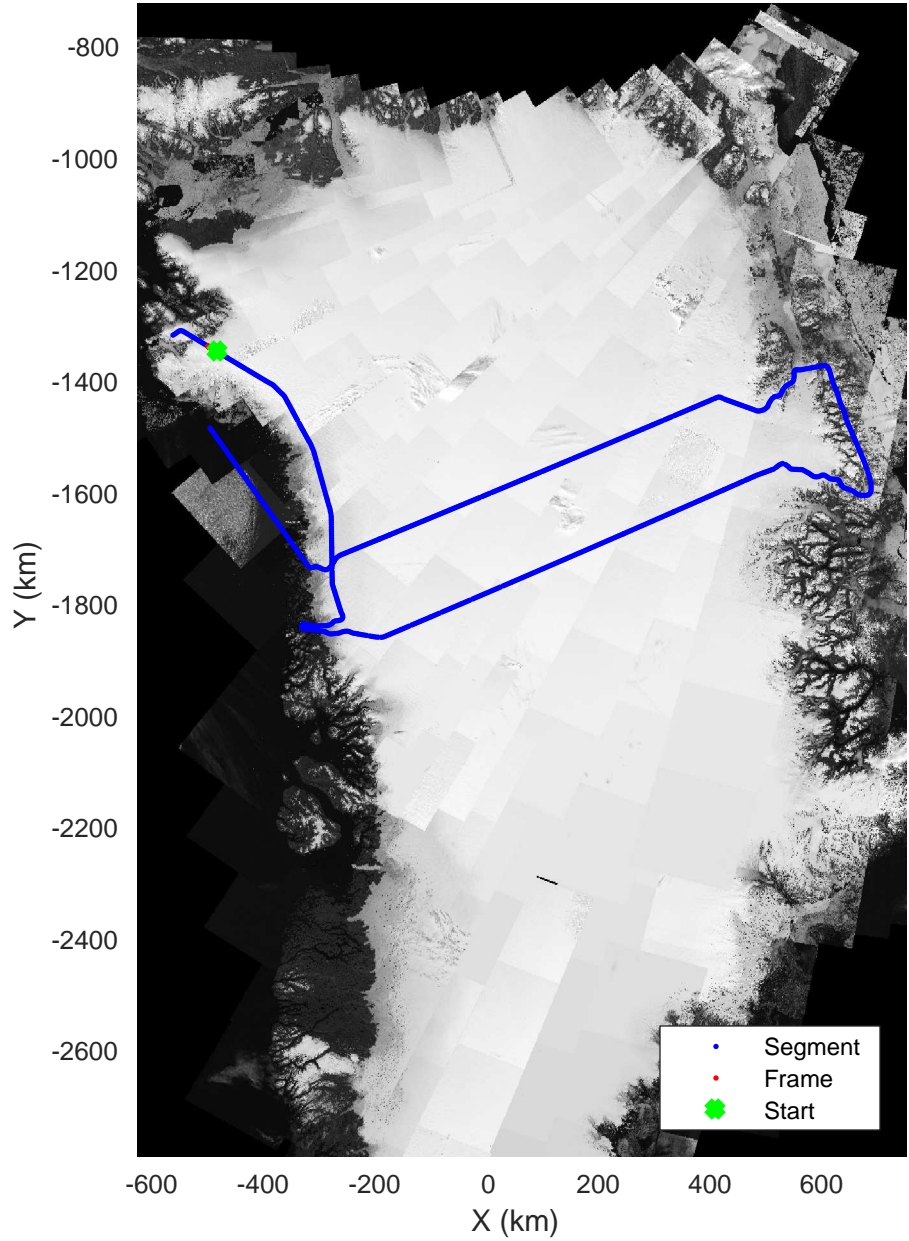
North Central Gap 03 20170410_01_171 Polar Stereograph 70N/-45E
