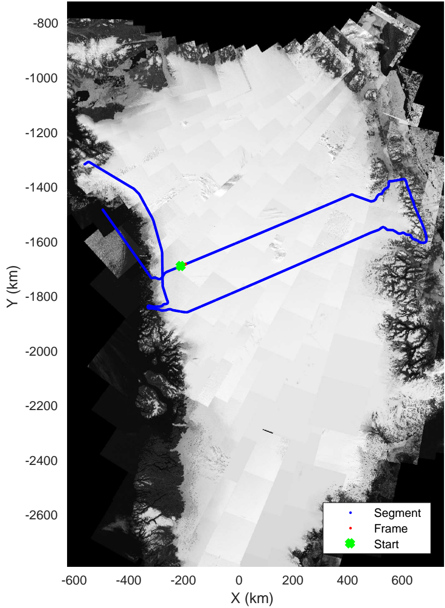
North Central Gap 03 20170410_01_023 Polar Stereograph 70N/-45E
