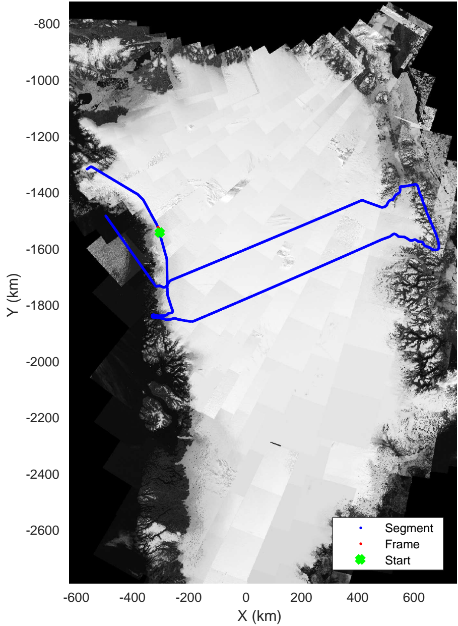
North Central Gap 03 20170410_01_157 Polar Stereograph 70N/-45E
