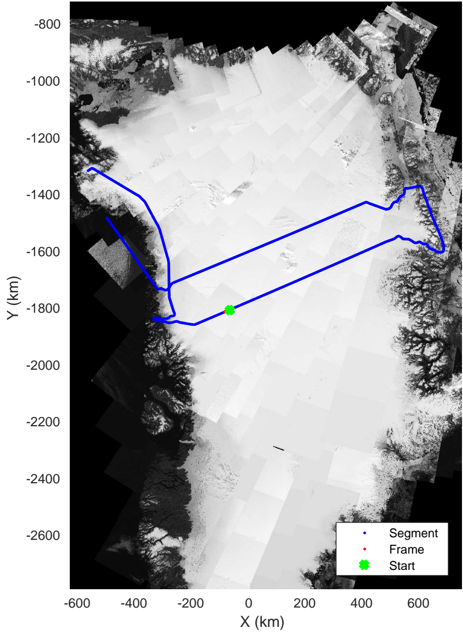
North Central Gap 03 20170410_01_124 Polar Stereograph 70N/-45E
