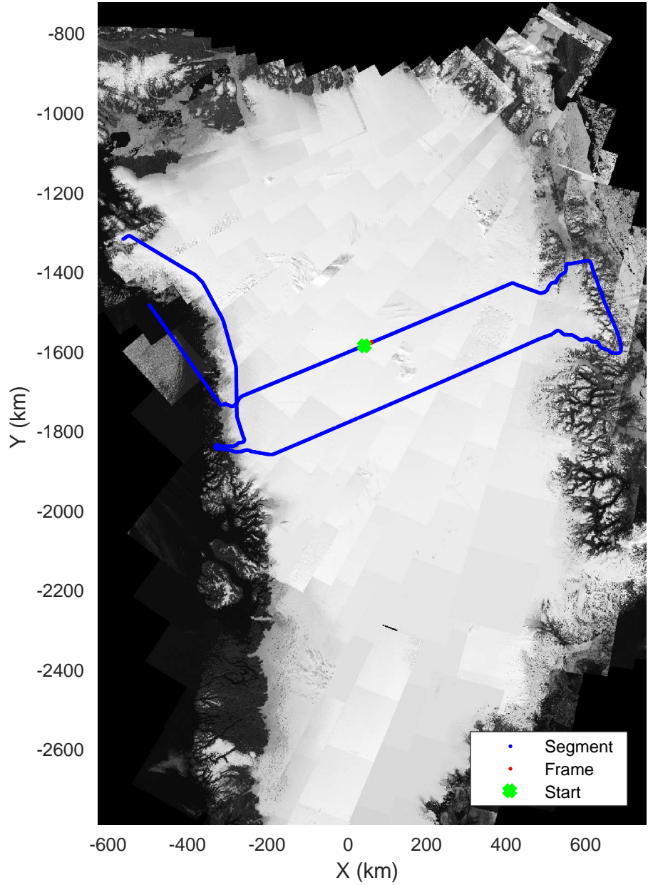
North Central Gap 03 20170410_01_037 Polar Stereograph 70N/-45E
