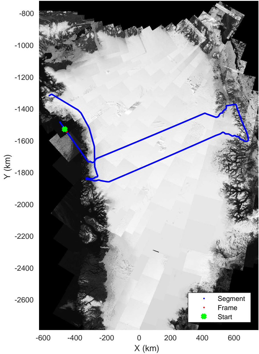
North Central Gap 03 20170410_01_004 Polar Stereograph 70N/-45E
