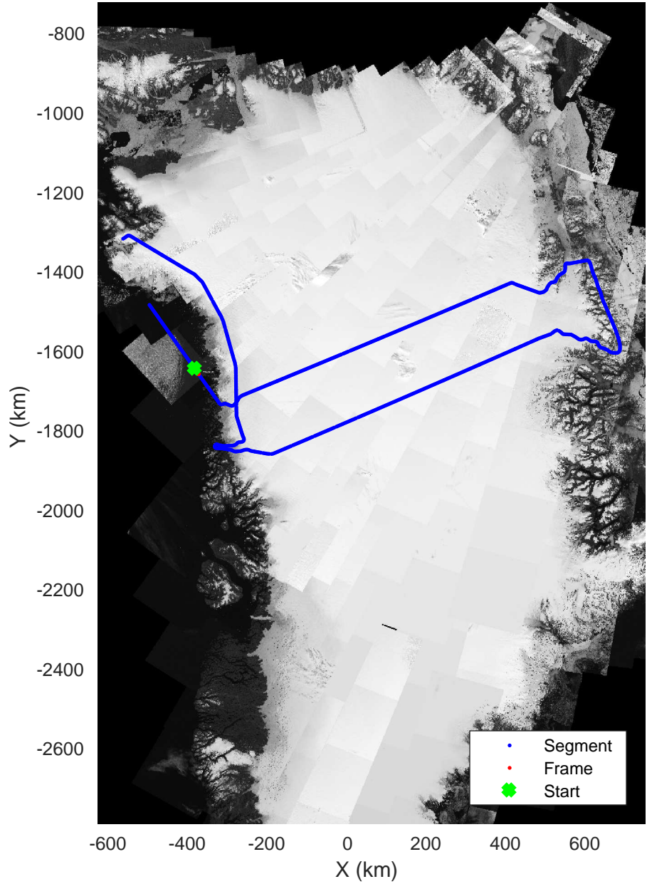
North Central Gap 03 20170410_01_011 Polar Stereograph 70N/-45E
