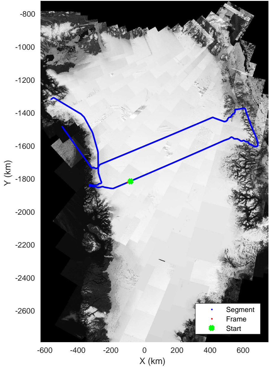
North Central Gap 03 20170410_01_125 Polar Stereograph 70N/-45E
