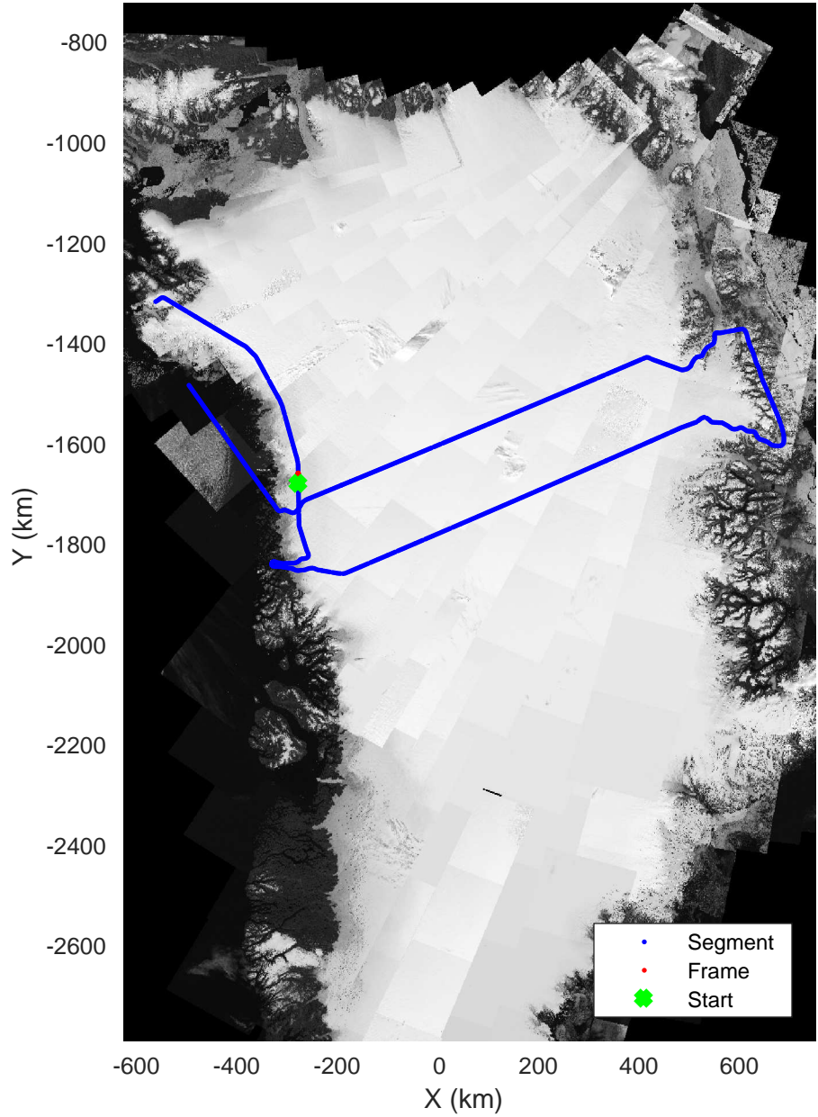
North Central Gap 03 20170410_01_150 Polar Stereograph 70N/-45E
