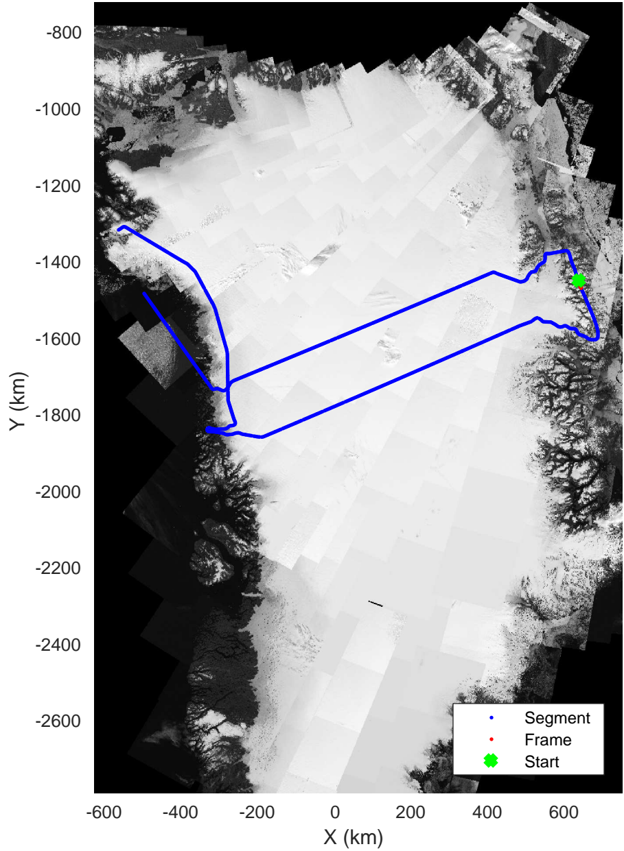
North Central Gap 03 20170410_01_074 Polar Stereograph 70N/-45E
