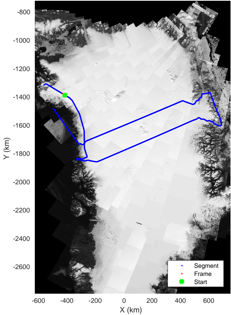
North Central Gap 03 20170410_01_167 Polar Stereograph 70N/-45E
