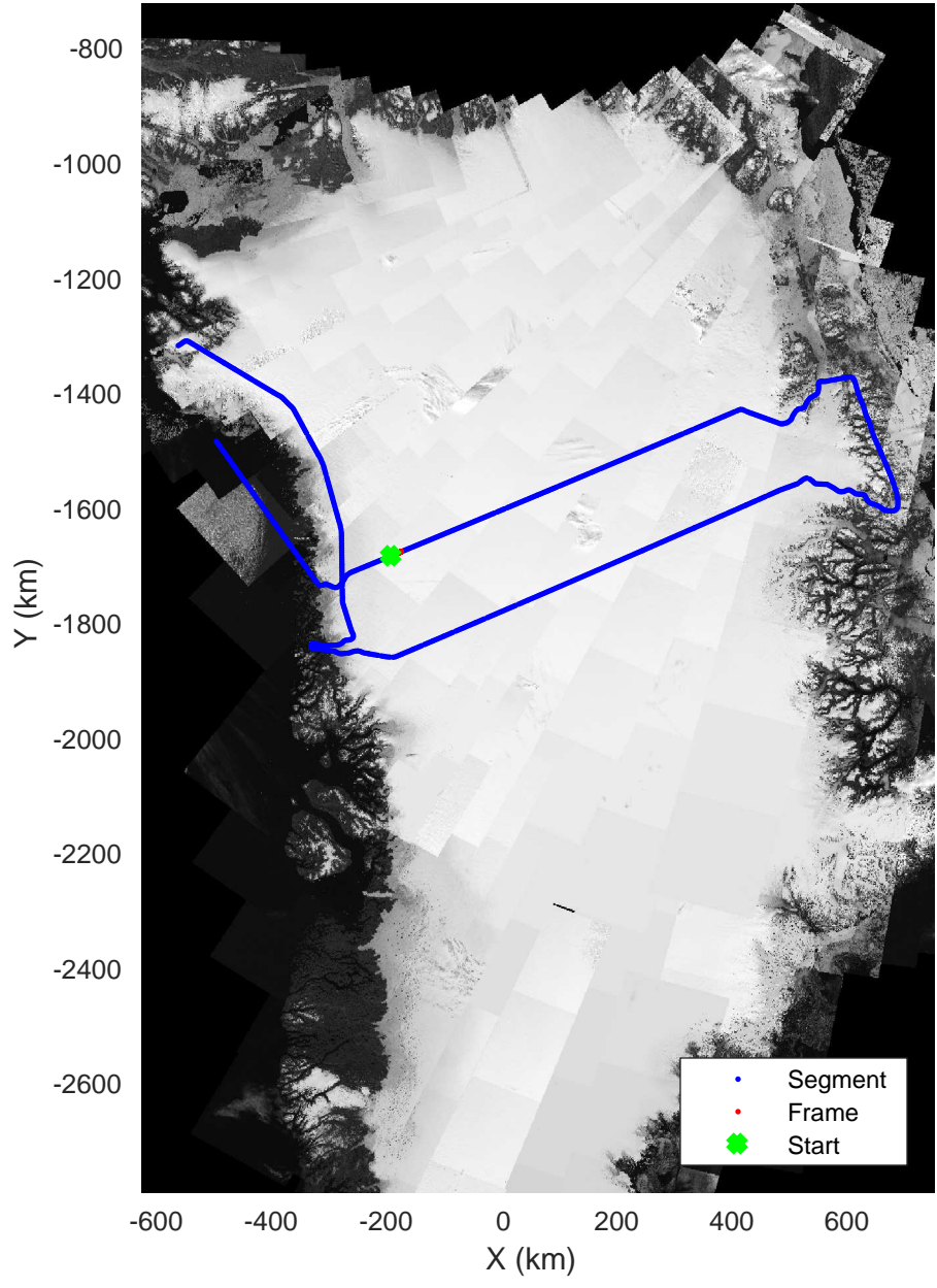
North Central Gap 03 20170410_01_024 Polar Stereograph 70N/-45E
