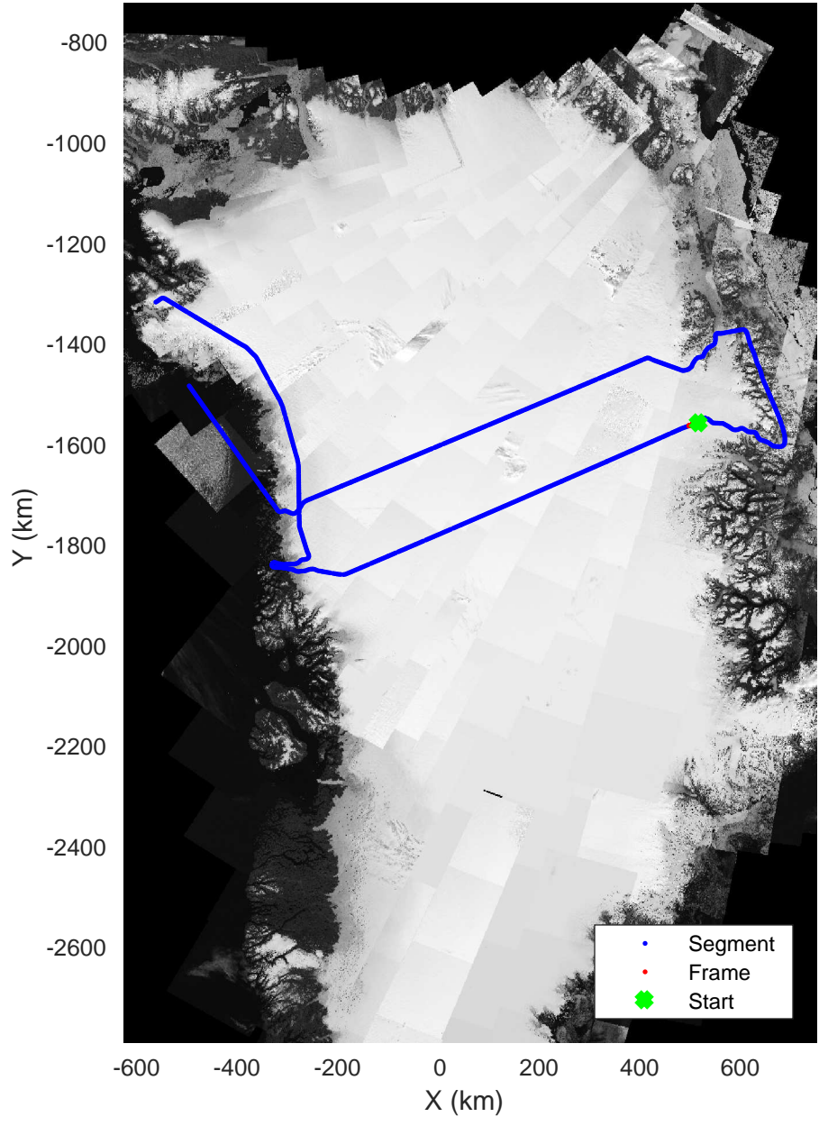
North Central Gap 03 20170410_01_092 Polar Stereograph 70N/-45E
