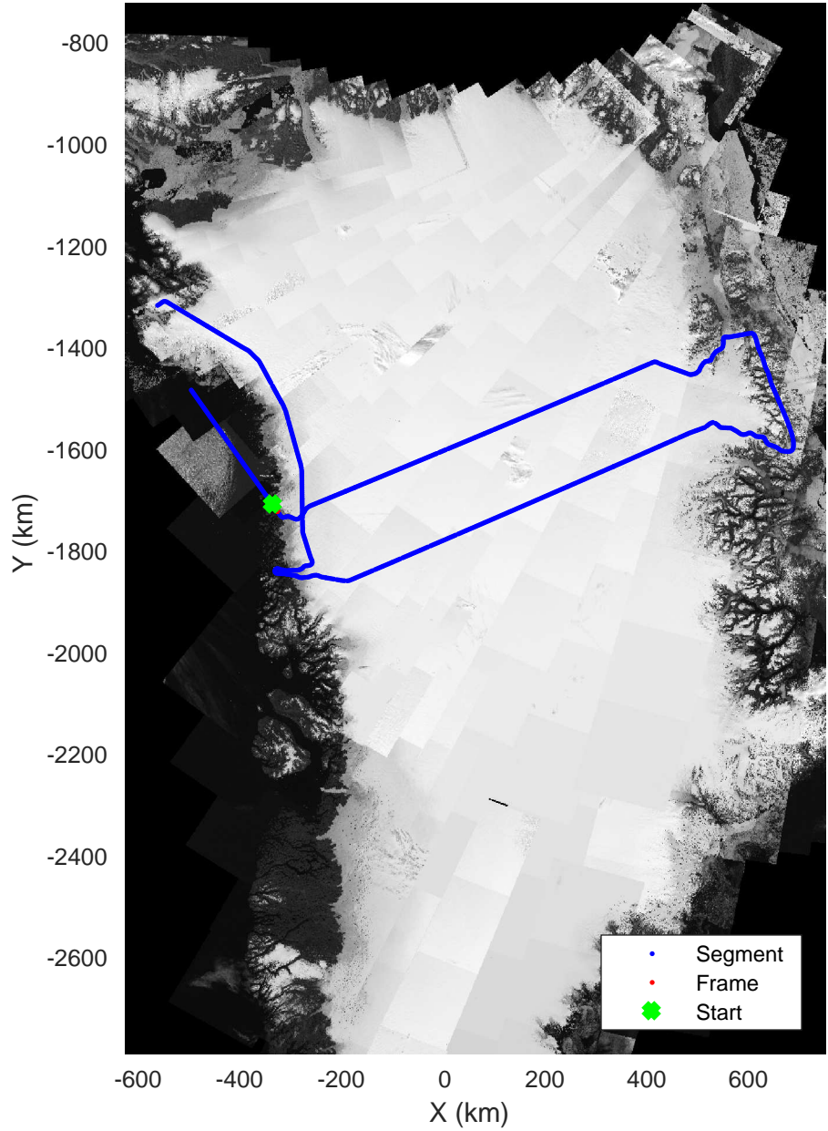
North Central Gap 03 20170410_01_015 Polar Stereograph 70N/-45E
