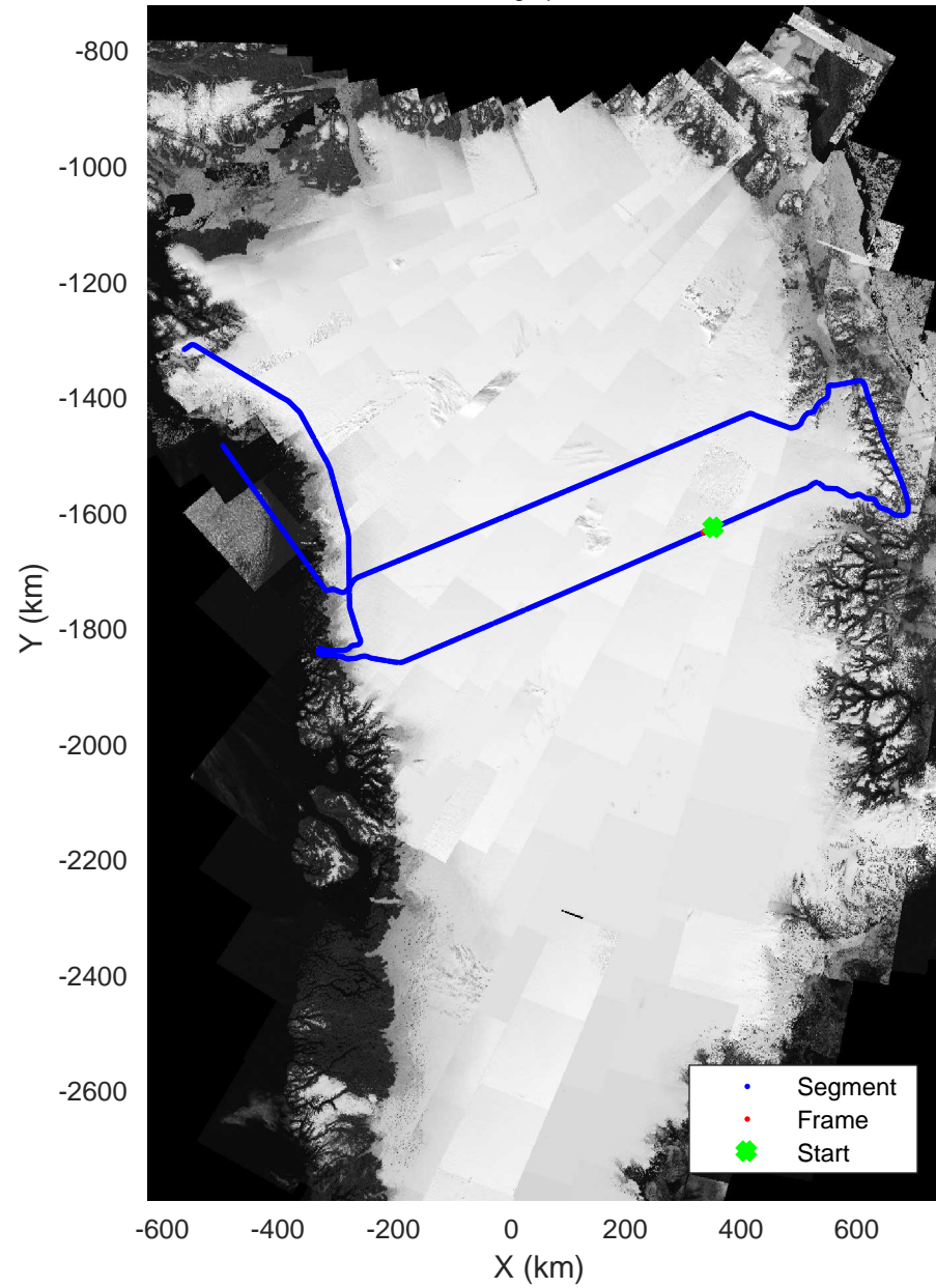
North Central Gap 03 20170410_01_101 Polar Stereograph 70N/-45E
