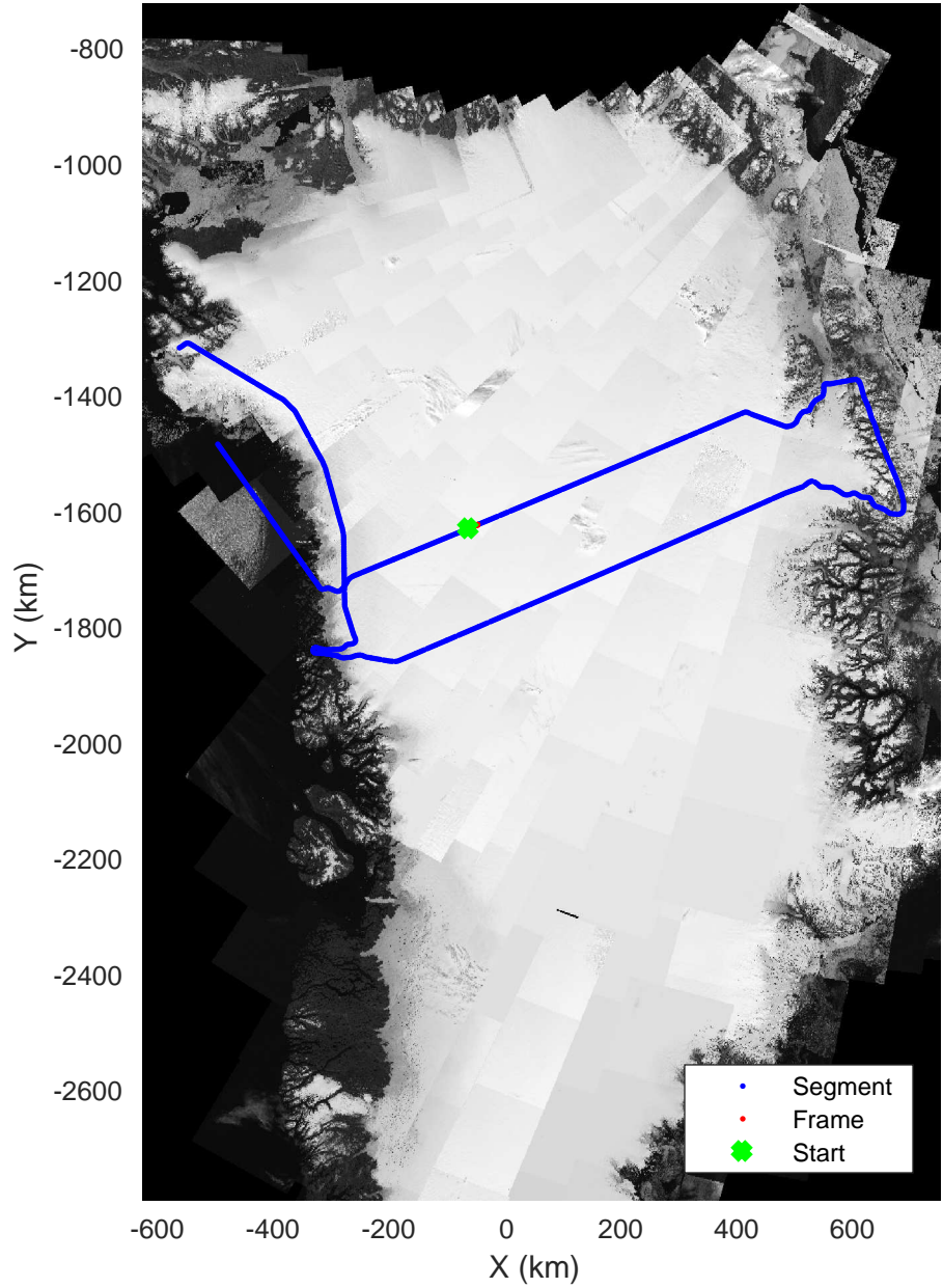
North Central Gap 03 20170410_01_031 Polar Stereograph 70N/-45E
