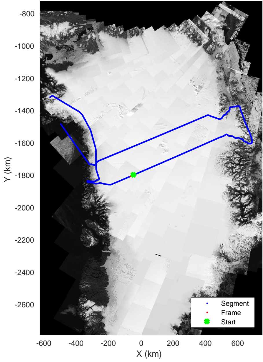
North Central Gap 03 20170410_01_123 Polar Stereograph 70N/-45E
