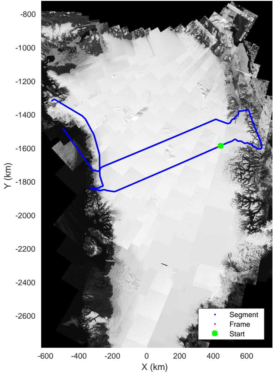
North Central Gap 03 20170410_01_096 Polar Stereograph 70N/-45E
