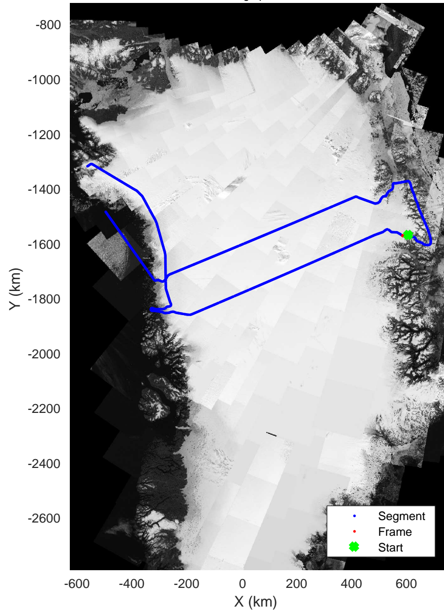
North Central Gap 03 20170410_01_087 Polar Stereograph 70N/-45E
