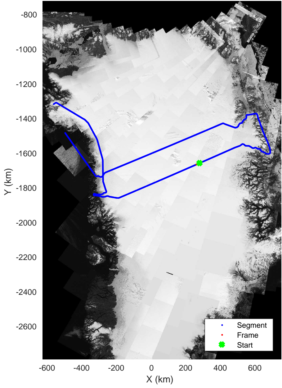
North Central Gap 03 20170410_01_105 Polar Stereograph 70N/-45E
