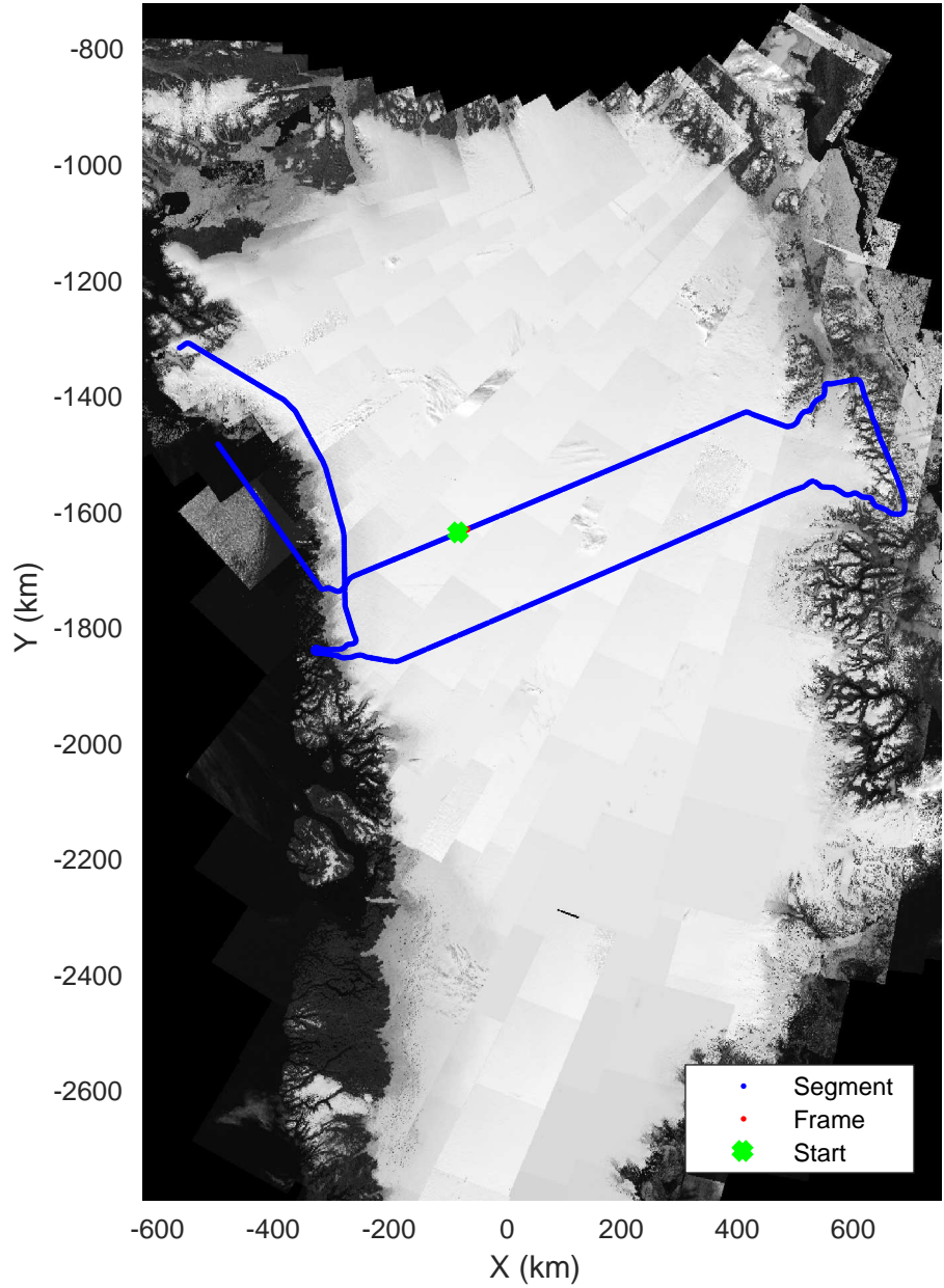
North Central Gap 03 20170410_01_030 Polar Stereograph 70N/-45E
