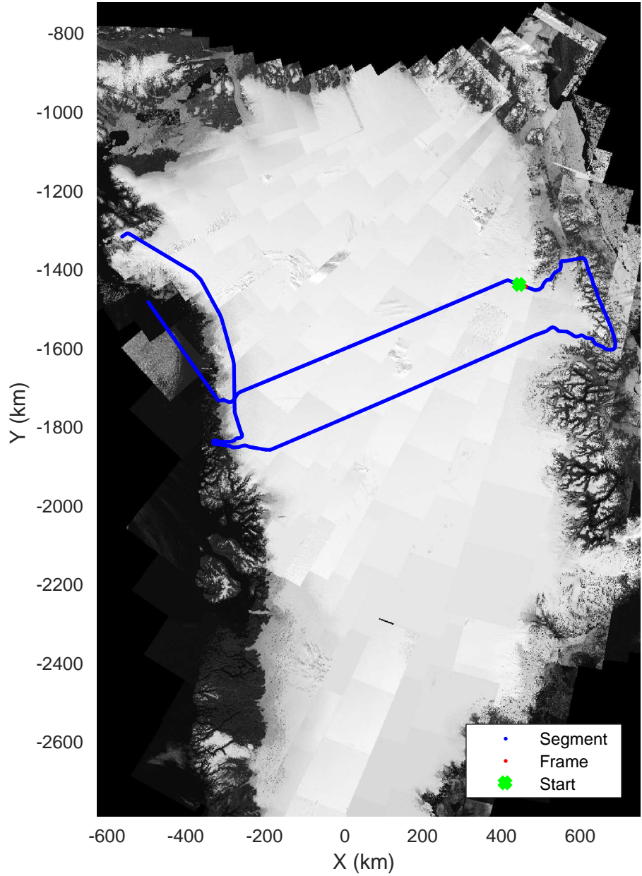
North Central Gap 03 20170410_01_059 Polar Stereograph 70N/-45E
