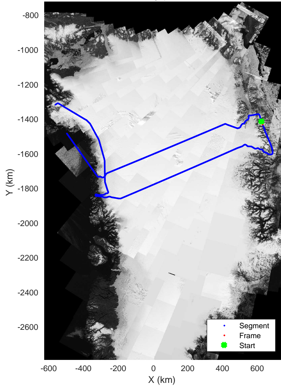
North Central Gap 03 20170410_01_072 Polar Stereograph 70N/-45E
