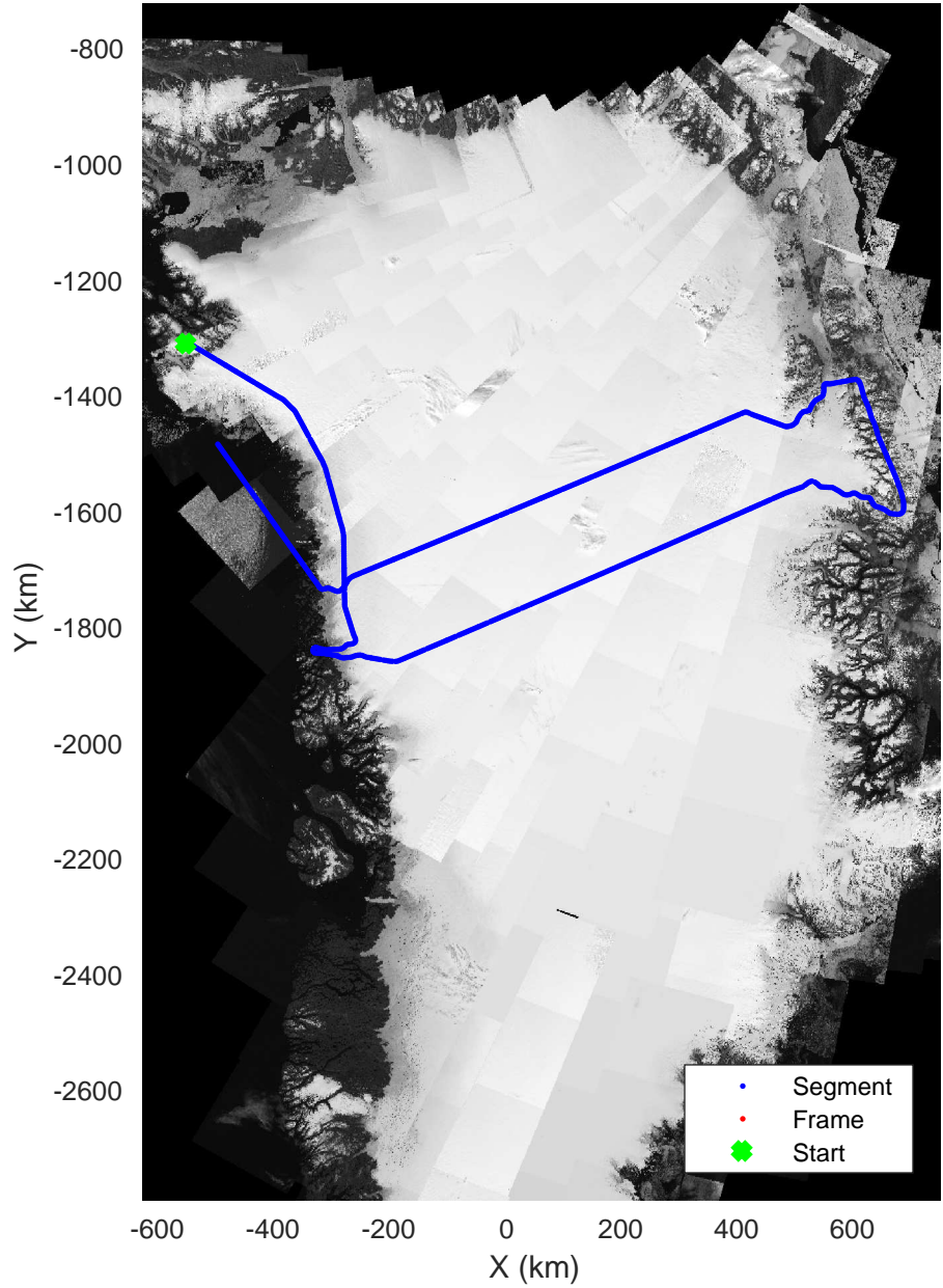
North Central Gap 03 20170410_01_175 Polar Stereograph 70N/-45E
