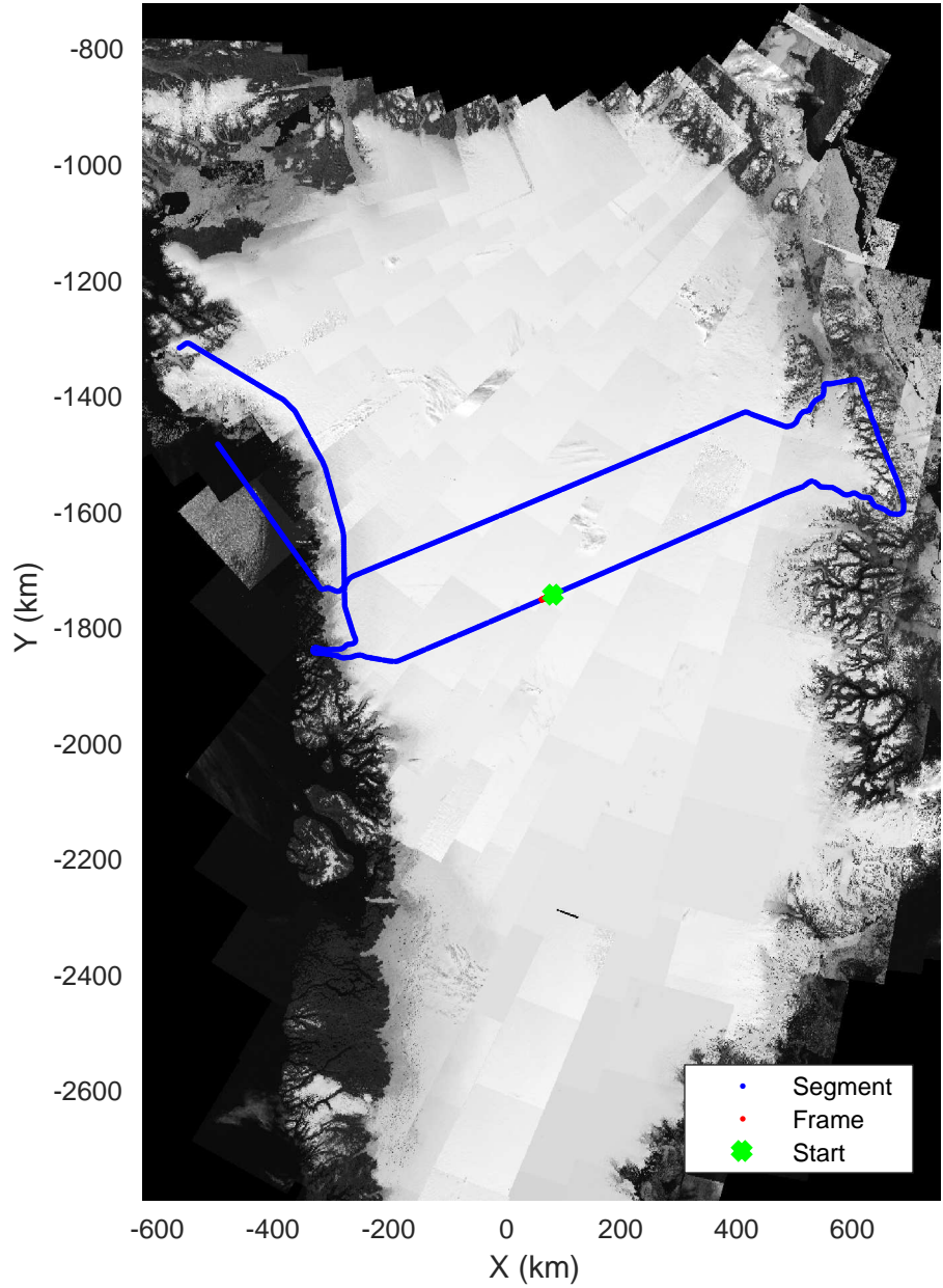
North Central Gap 03 20170410_01_116 Polar Stereograph 70N/-45E
