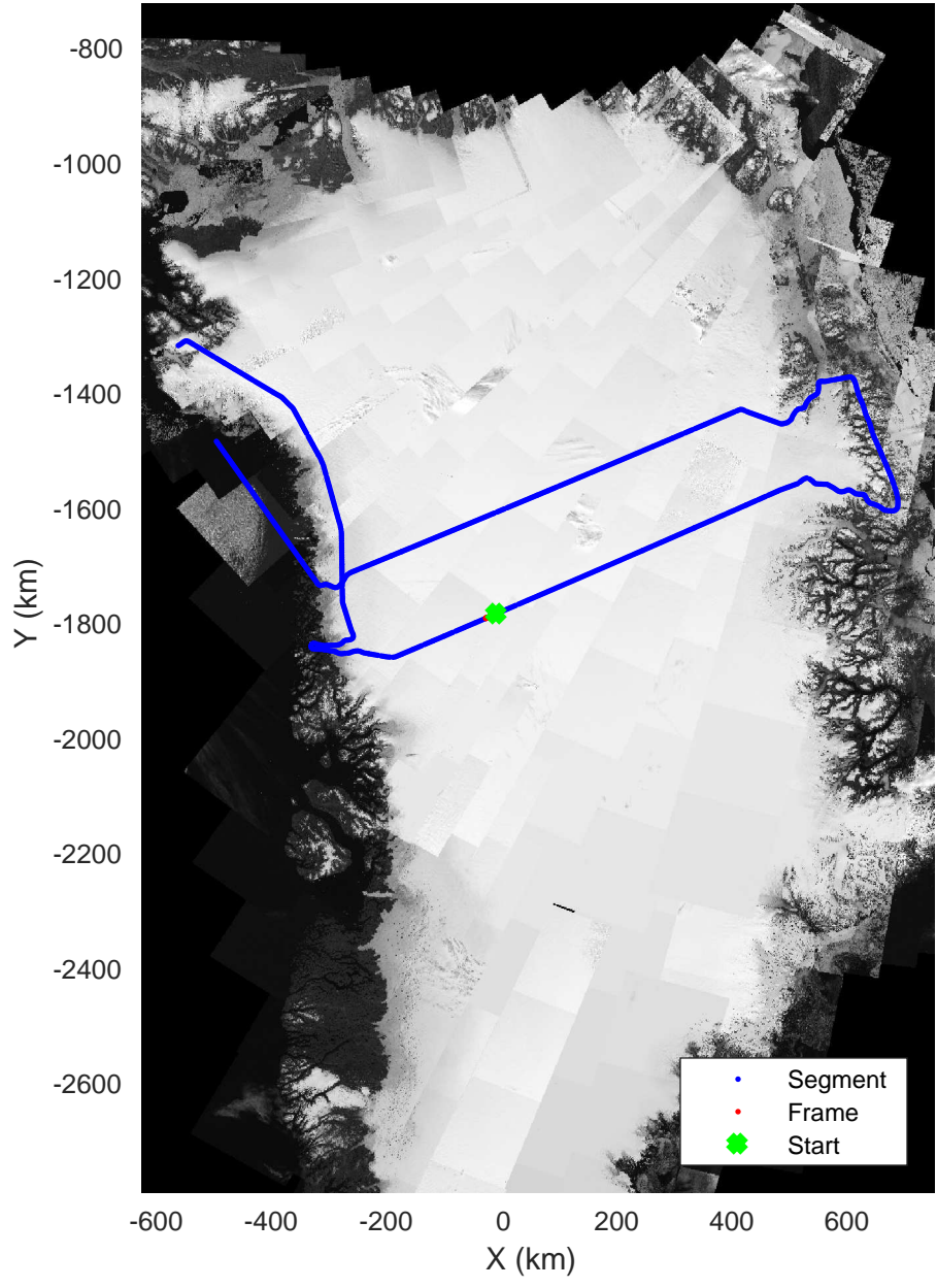
North Central Gap 03 20170410_01_121 Polar Stereograph 70N/-45E
