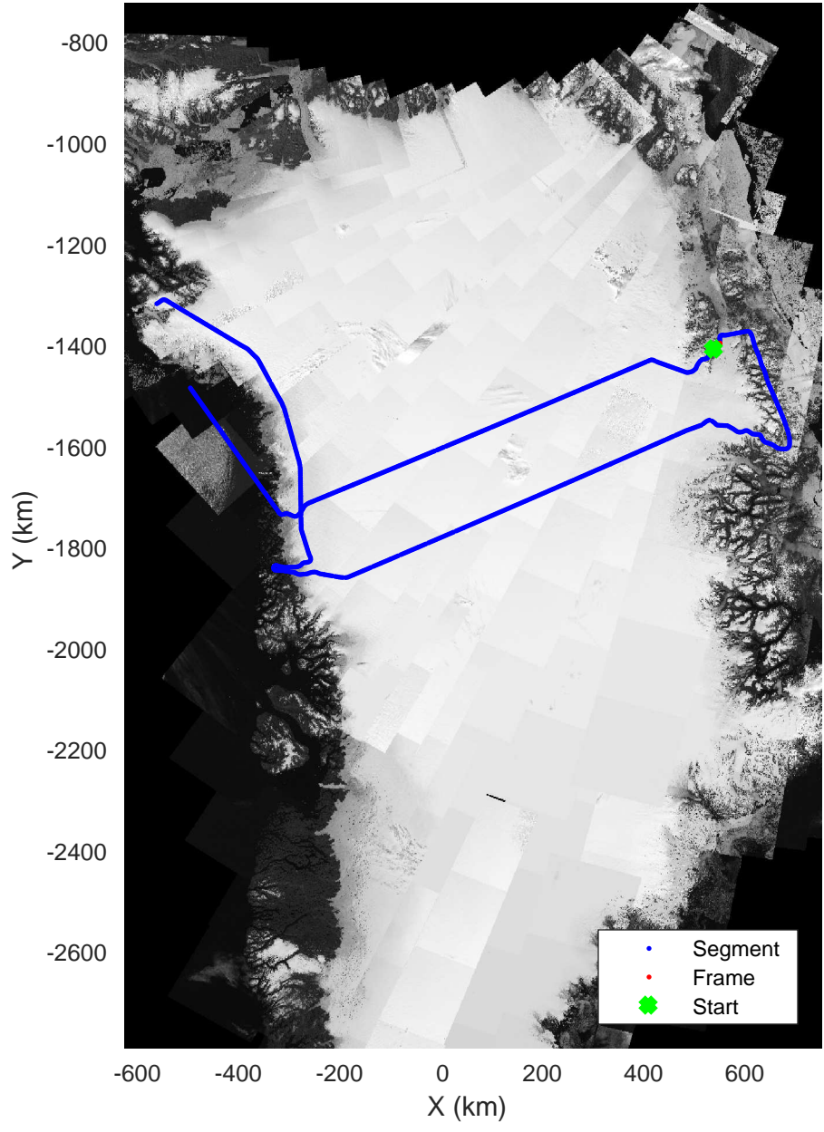
North Central Gap 03 20170410_01_065 Polar Stereograph 70N/-45E
