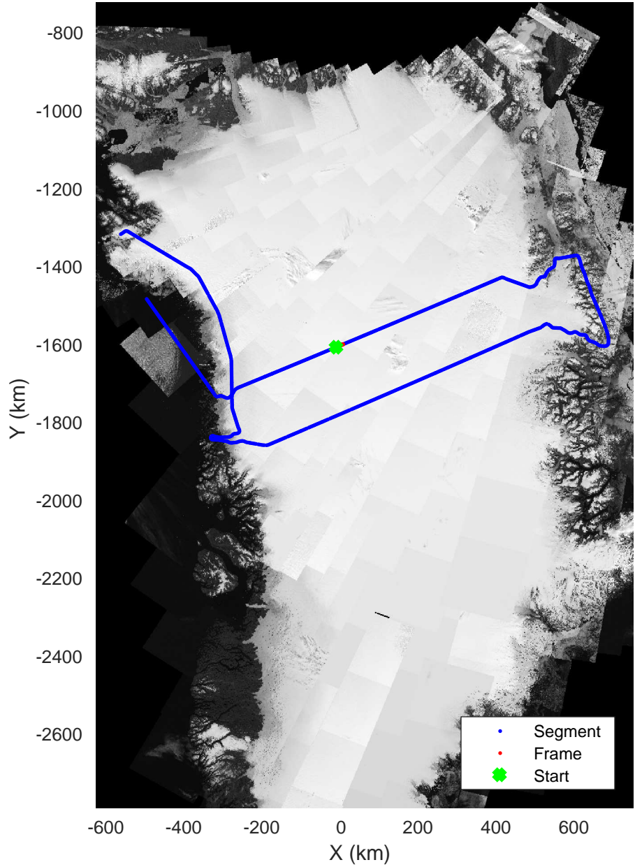
North Central Gap 03 20170410_01_034 Polar Stereograph 70N/-45E
