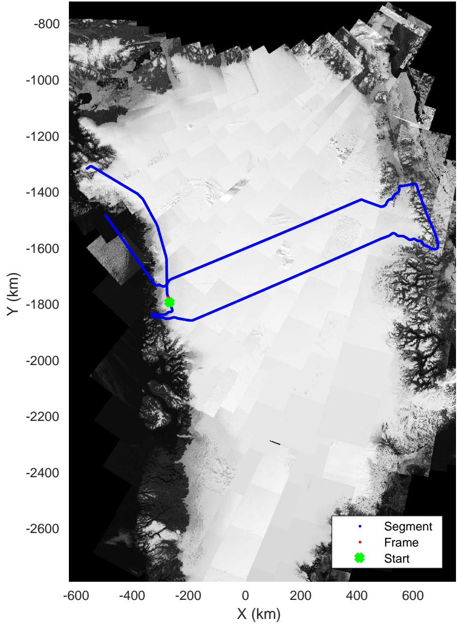
North Central Gap 03 20170410_01_144 Polar Stereograph 70N/-45E
