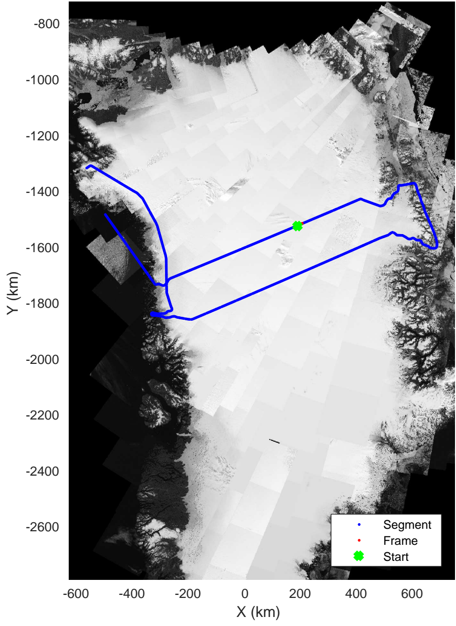
North Central Gap 03 20170410_01_045 Polar Stereograph 70N/-45E
