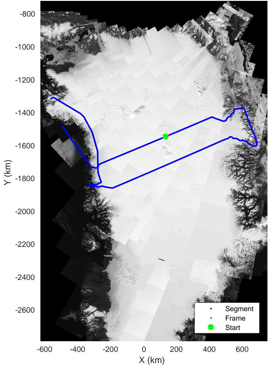
North Central Gap 03 20170410_01_042 Polar Stereograph 70N/-45E
