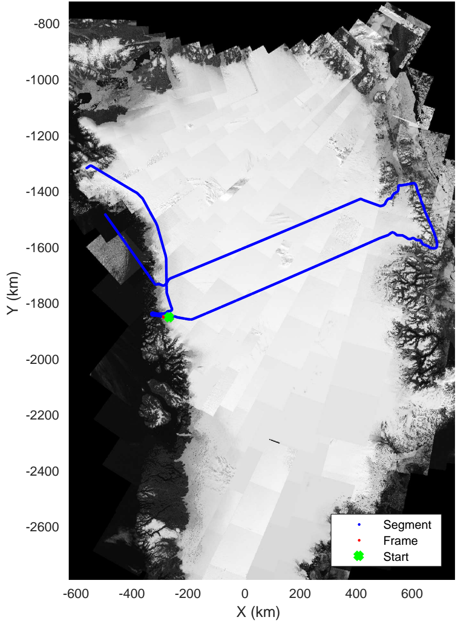
North Central Gap 03 20170410_01_135 Polar Stereograph 70N/-45E
