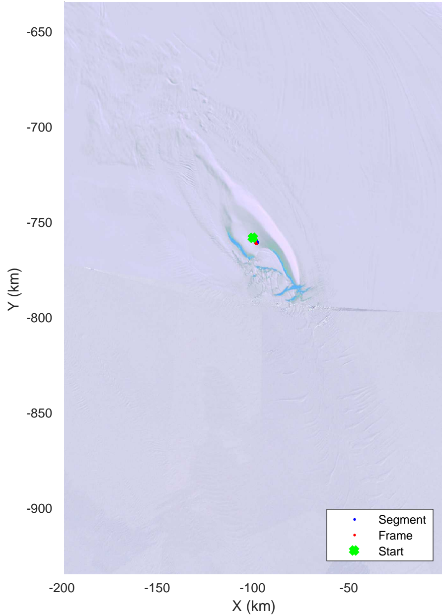
Far side of 6km hyperbola, local time 1221 20151221_01_009 Polar Stereograph -71N/0E
