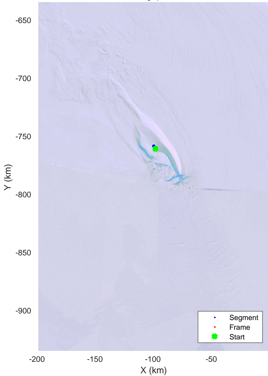
Far side of 6km hyperbola, local time 1221 20151221_01_006 Polar Stereograph -71N/0E
