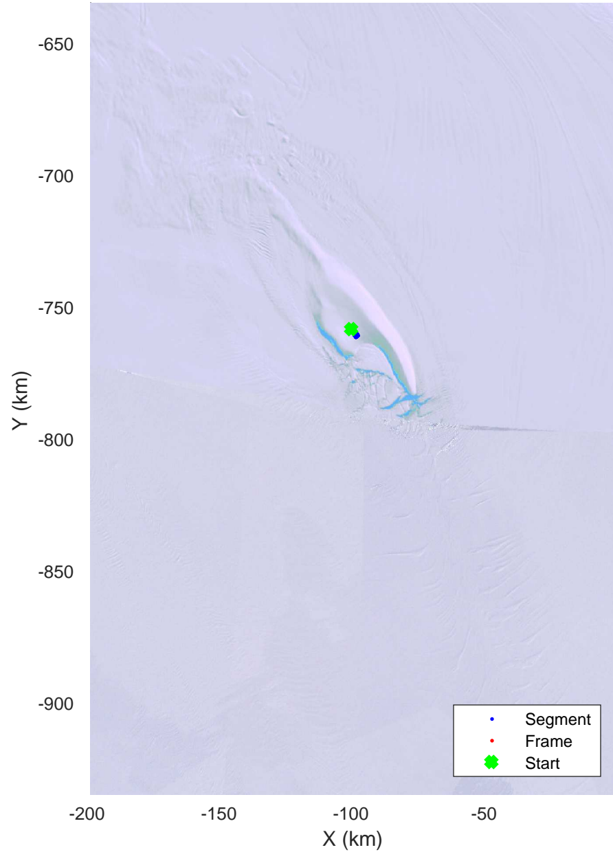
Far side of 6km hyperbola, local time 1221 20151221_01_008 Polar Stereograph -71N/0E
