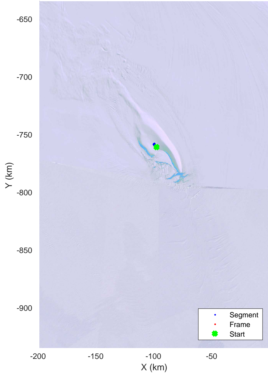
Far side of 6km hyperbola, local time 1221 20151221_01_002 Polar Stereograph -71N/0E
