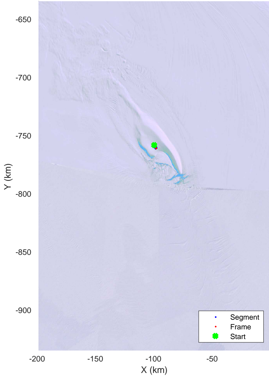
Far side of 6km hyperbola, local time 1221 20151221_01_005 Polar Stereograph -71N/0E
