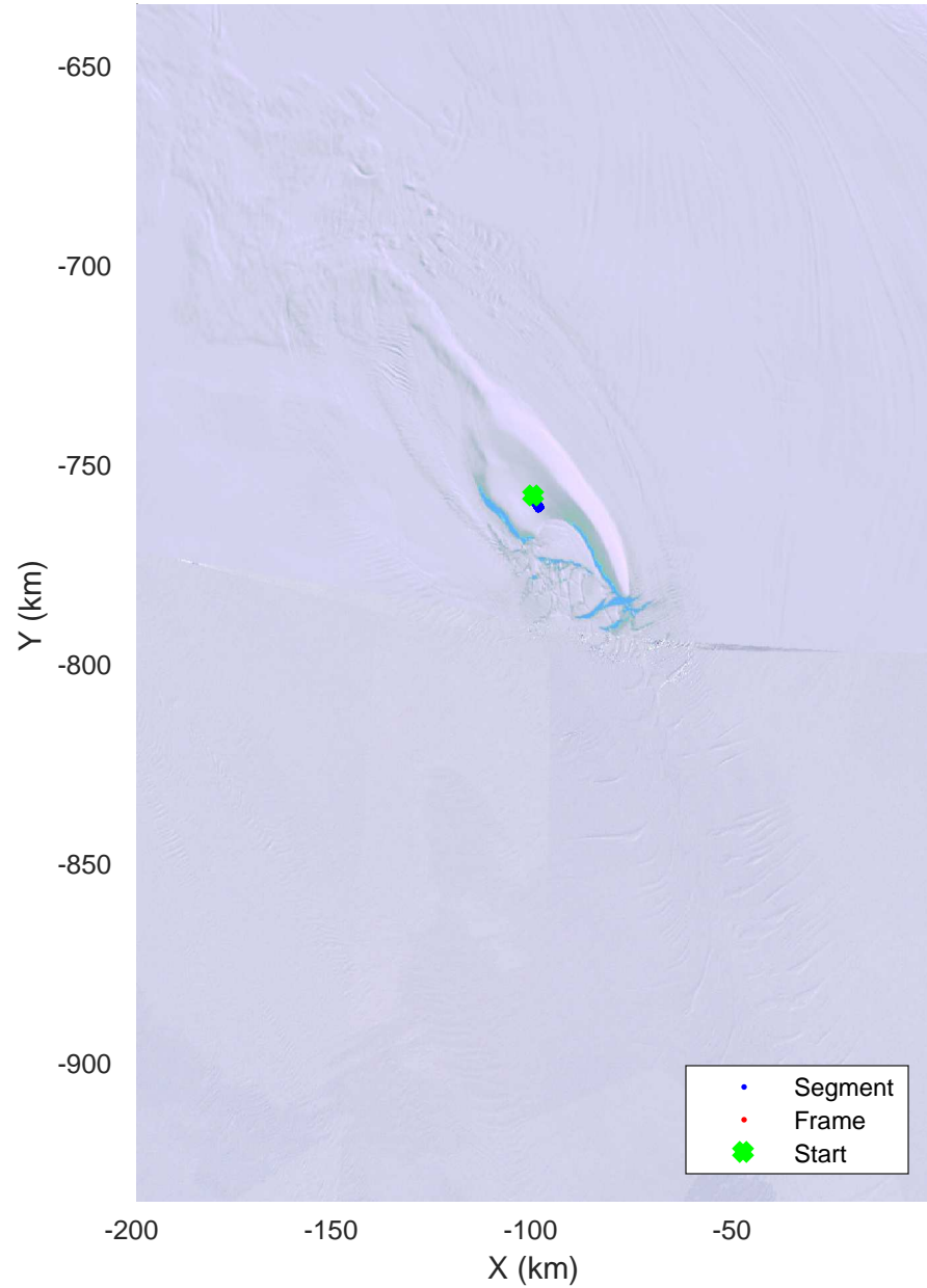
Far side of 6km hyperbola, local time 1221 20151221_01_004 Polar Stereograph -71N/0E
