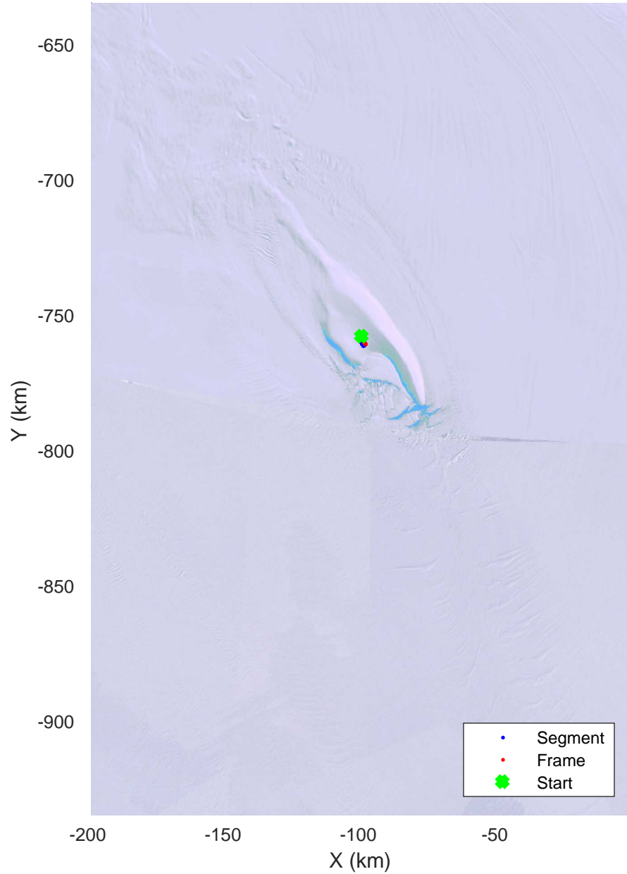
Far side of 6km hyperbola, local time 1221 20151221_01_001 Polar Stereograph -71N/0E
