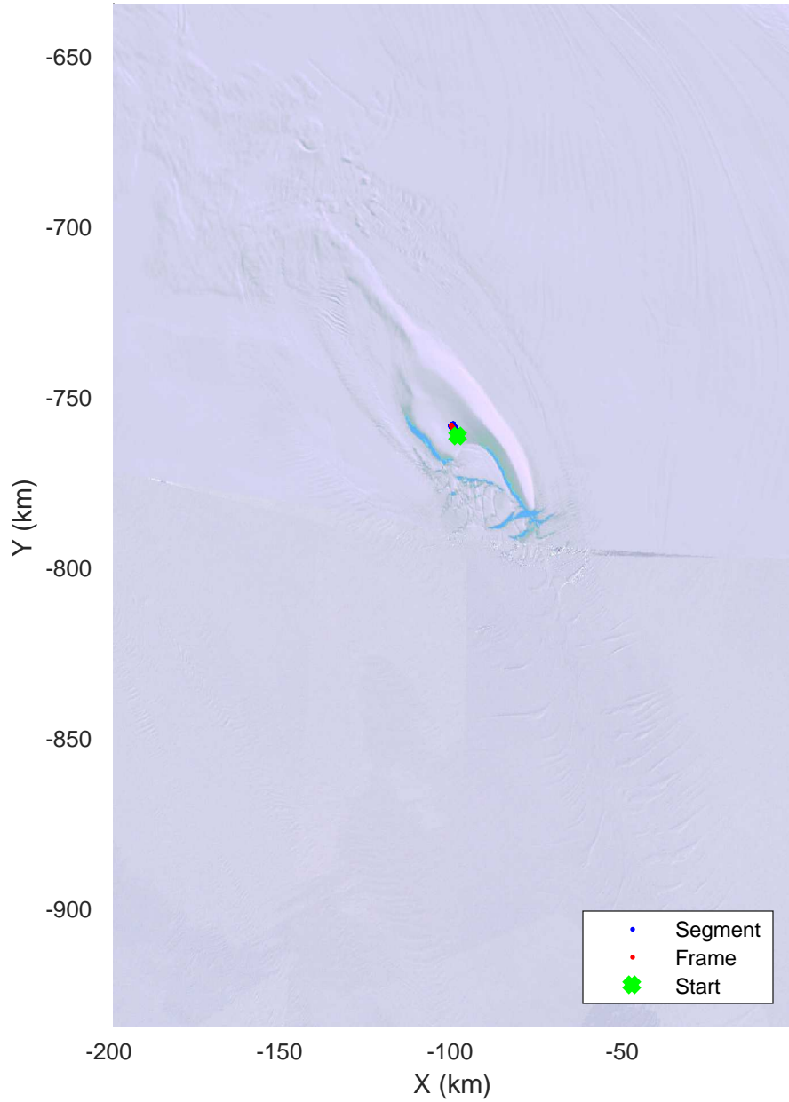
Far side of 6km hyperbola, local time 1221 20151221_01_007 Polar Stereograph -71N/0E
