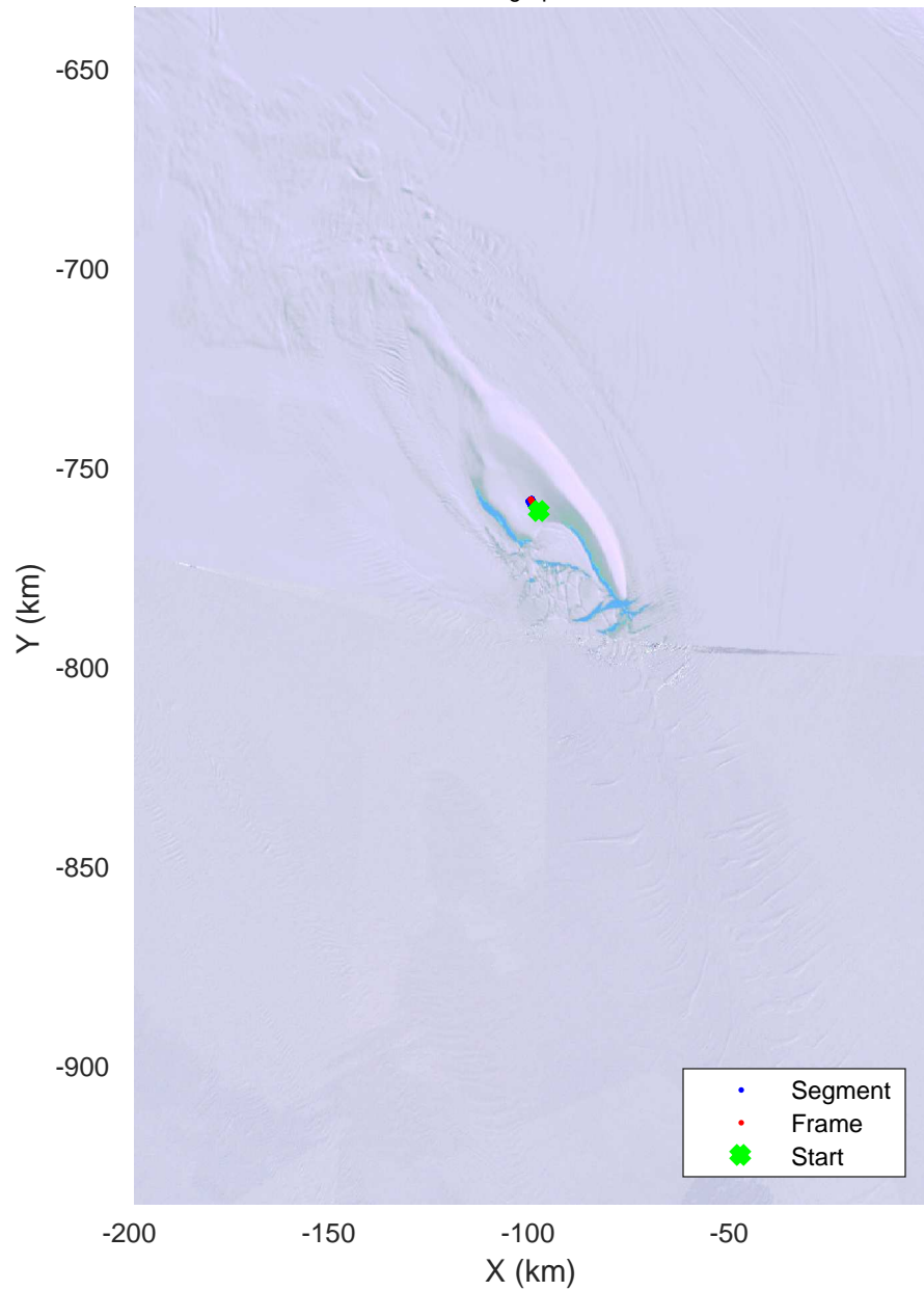
Far side of 6km hyperbola, local time 1221 20151221_01_003 Polar Stereograph -71N/0E
